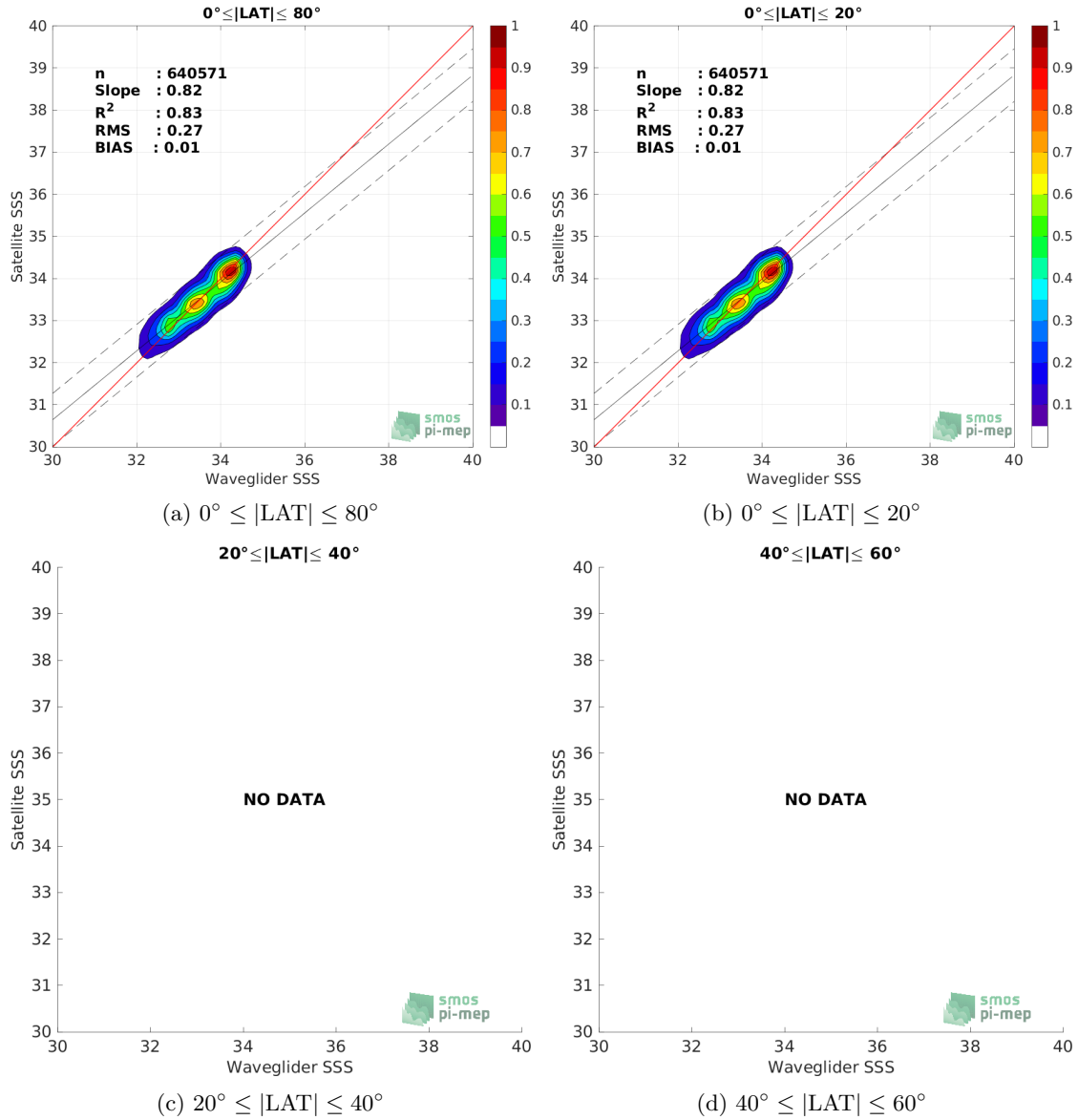
Figure 9: Contour maps of the concentration of SMOS SSS L3 v7 - 9 Days (CATDS-CECOS-LOCEAN) SSS (y-axis) versus Waveglider SSS (x-axis) at match-up pairs for different latitude bands. For each plot, the red line shows x=y . The black thin and dashed lines indicate a linear fit through the data cloud and the \pm 95\% confidence levels, respectively. The number match-up pairs n , the slope and R^2 coefficient of the linear fit, the root mean square (RMS) and the mean bias between satellite and in situ data are indicated for each latitude band in each plots.
