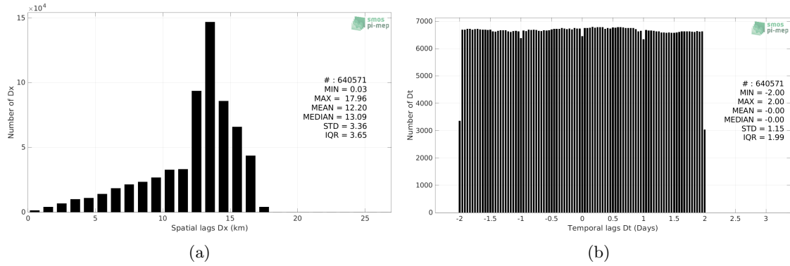
Figure 5: Histograms of the spatial (a) and temporal (b) lags between the location/time of the Waveglider measurement and the date of the corresponding SMOS SSS L3 v7 - 9 Days (CATDS-CECOS-LOCEAN) SSS pixel.
