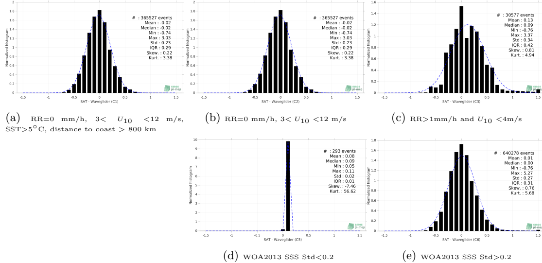
Figure 13: Normalized histogram of \Delta SSS (SMOS SSS L3 v7 - 9 Days (CATDS-CECOS-LOCEAN) - Waveglider) for 5 different subdatasets corresponding to: RR=0 mm/h, 3 < U_{10} < 12 m/s, SST > 5°C, distance to coast > 800 km (a), RR=0 mm/h, 3 < U_{10} < 12 m/s (b), RR > 1mm/h and U_{10} < 4 m/s (c), WOA2013 SSS Std < 0.2 (d), WOA2013 SSS Std > 0.2 (e).
