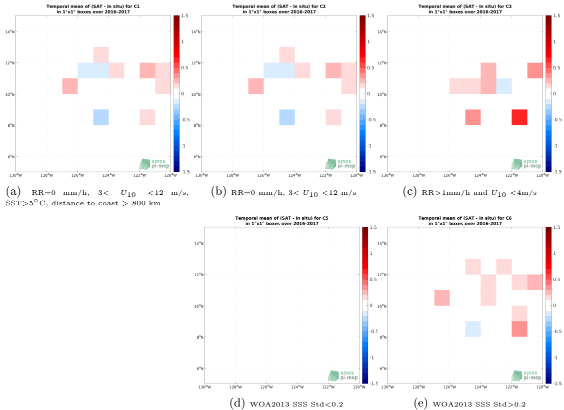
Figure 12: Temporal mean gridded over spatial boxes of size 1^\circ \times 1^\circ of \Delta SSS (SMOS SSS L3 v7 - 9 Days (CATDS-CECOS-LOCEAN) - Waveglider) for 5 different subdatasets corresponding to: RR=0 mm/h, 3 < U_{10} < 12 m/s, SST > 5^\circ\text{C} , distance to coast > 800 km (a), RR=0 mm/h, 3 < U_{10} < 12 m/s (b), RR > 1 mm/h and U_{10} < 4 m/s (c), WOA2013 SSS Std < 0.2 (d), WOA2013 SSS Std > 0.2 (e).
