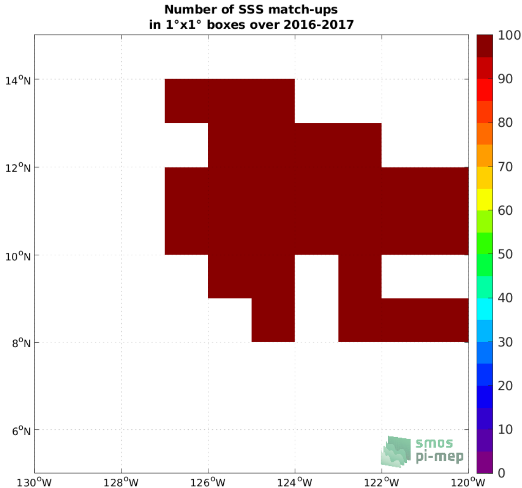
Figure 4: Number of SSS match-ups between Waveglider SSS and the SMOS SSS L3 v7 - 9 Days (CATDS-CECOS-LOCEAN) SSS product for the SPURS 2 Pi-MEP region over 1^\circ \times 1^\circ boxes and for the full satellite product period.
