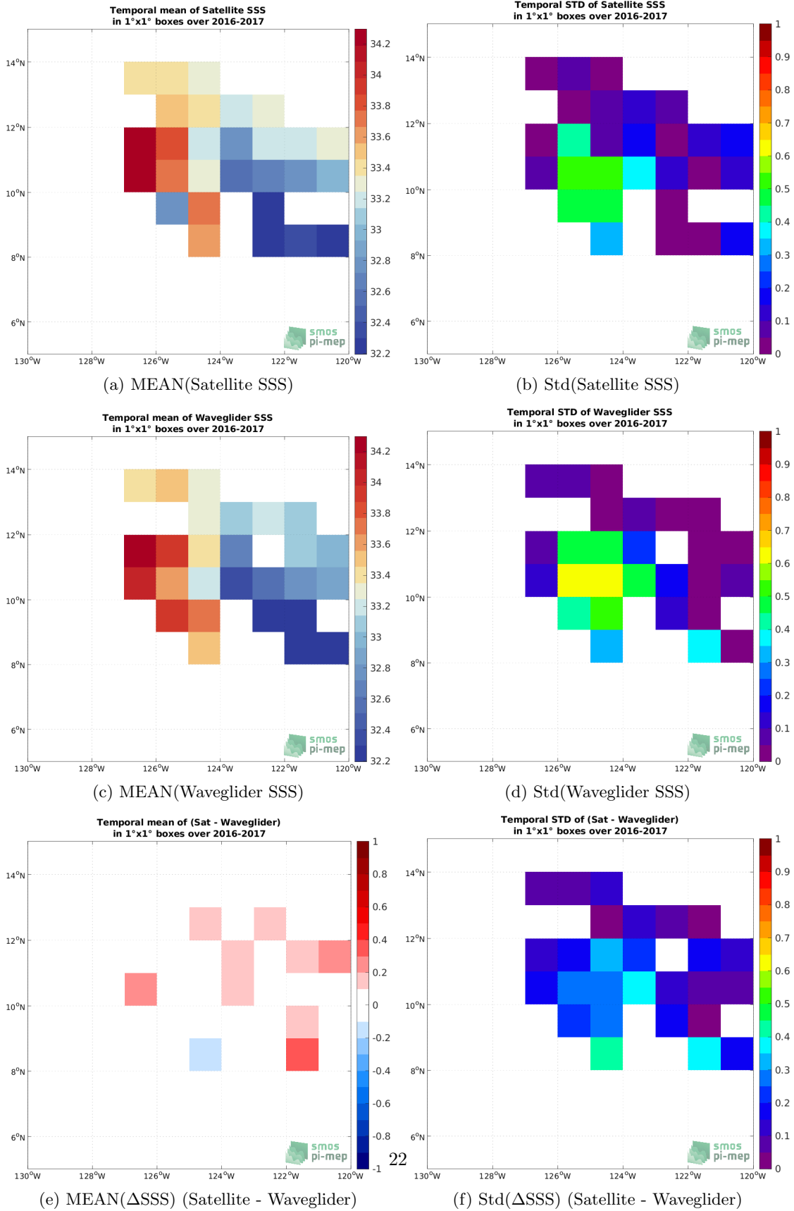
Figure 6: Temporal mean (left) and Std (right) of SSS from SMOS SSS L3 v7 - 9 Days (CATDS-CECOS-LOCEAN) (top), Waveglider (middle), and of \Delta SSS (Satellite - Waveglider). Only match-up pairs are used to generate these maps.
