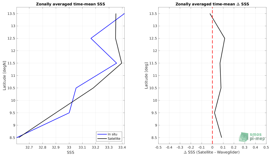
Figure 8: Left panel: Zonal mean SSS from SMOS SSS L3 v7 - 9 Days (CATDS-CECOS-LOCEAN) satellite product (black) and from Waveglider (blue). Right panel: Zonal mean of \Delta SSS (Satellite - Waveglider) for all the collected Pi-MEP match-up pairs estimated over the full satellite product period.
