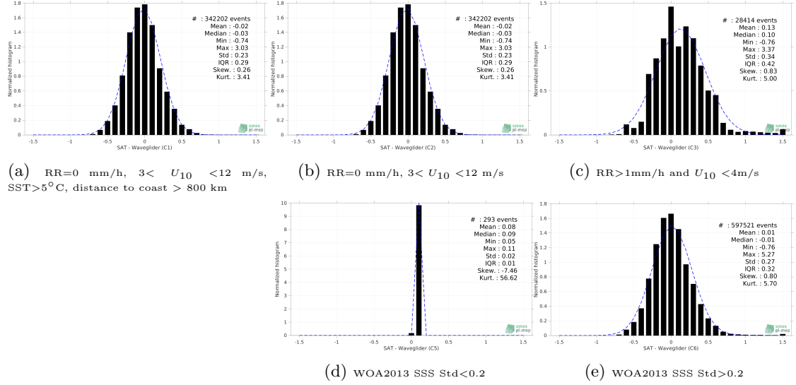
Figure 12: Normalized histogram of \Delta\text{SSS} (SMOS SSS L3 v7 - 9 Days (CATDS-CECOS-LOCEAN) - Waveglider) for 5 different subdatasets corresponding to: RR=0 mm/h, 3 < U_{10} < 12 m/s, SST >5^{\circ}\text{C} , distance to coast > 800 km (a), RR=0 mm/h, 3 < U_{10} < 12 m/s (b), RR >1 mm/h and U_{10} < 4 m/s (c), WOA2013 SSS Std <0.2 (d), WOA2013 SSS Std >0.2 (e).
