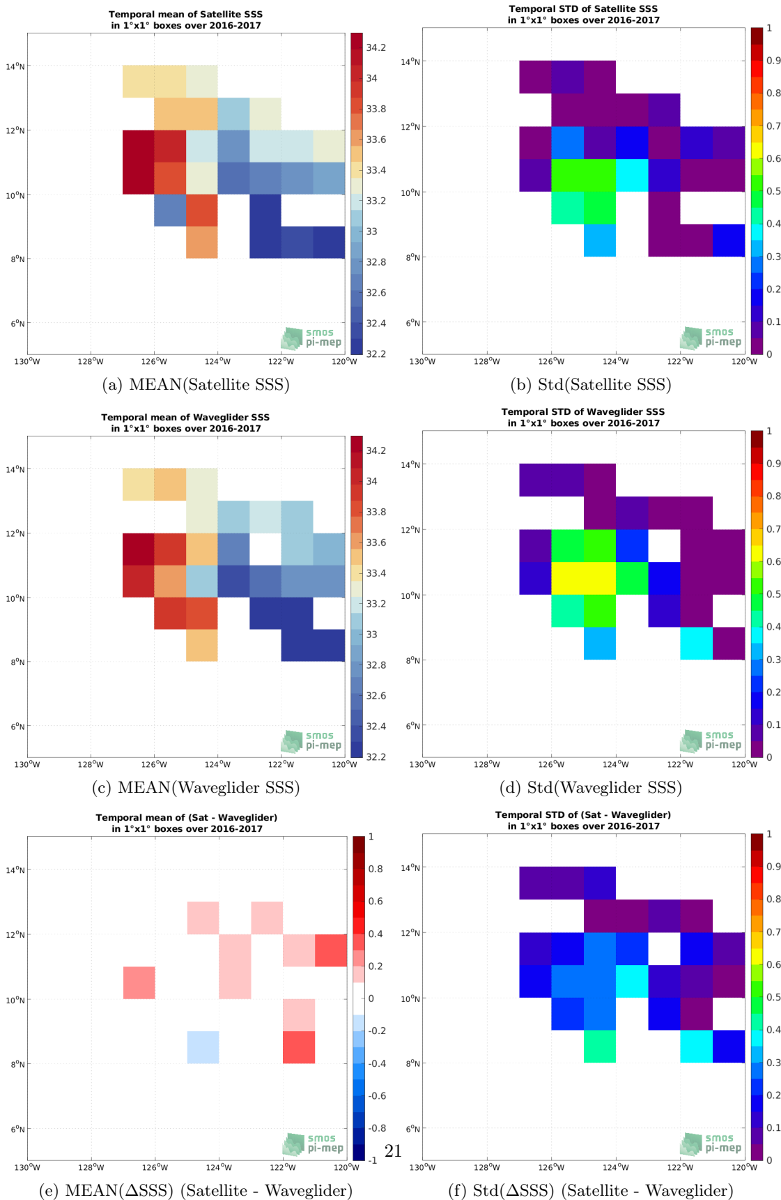
Figure 5: Temporal mean (left) and Std (right) of SSS from SMOS SSS L3 v7 - 9 Days (CATDS-CECOS-LOCEAN) (top), Waveglider (middle), and of \Delta SSS (Satellite - Waveglider). Only match-up pairs are used to generate these maps.
