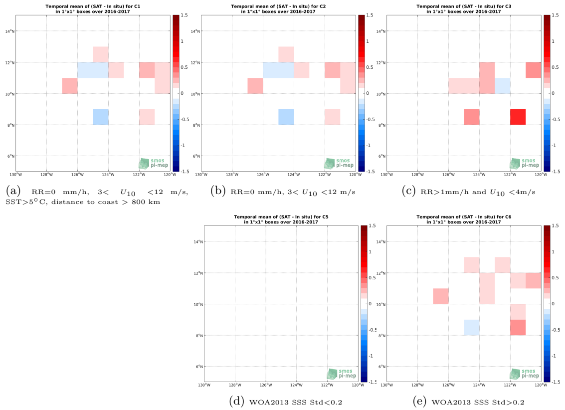
Figure 11: Temporal mean gridded over spatial boxes of size 1^\circ \times 1^\circ of \Delta SSS (SMOS SSS L3 v7 - 9 Days (CATDS-CECOS-LOCEAN) - Waveglider) for 5 different subdatasets corresponding to:RR=0 mm/h, 3 < U_{10} < 12 m/s, SST >5^\circ C, distance to coast > 800 km (a), RR=0 mm/h, 3 < U_{10} < 12 m/s (b), RR >1 mm/h and U_{10} < 4 m/s (c), WOA2013 SSS Std <0.2 (d), WOA2013 SSS Std >0.2 (e).
