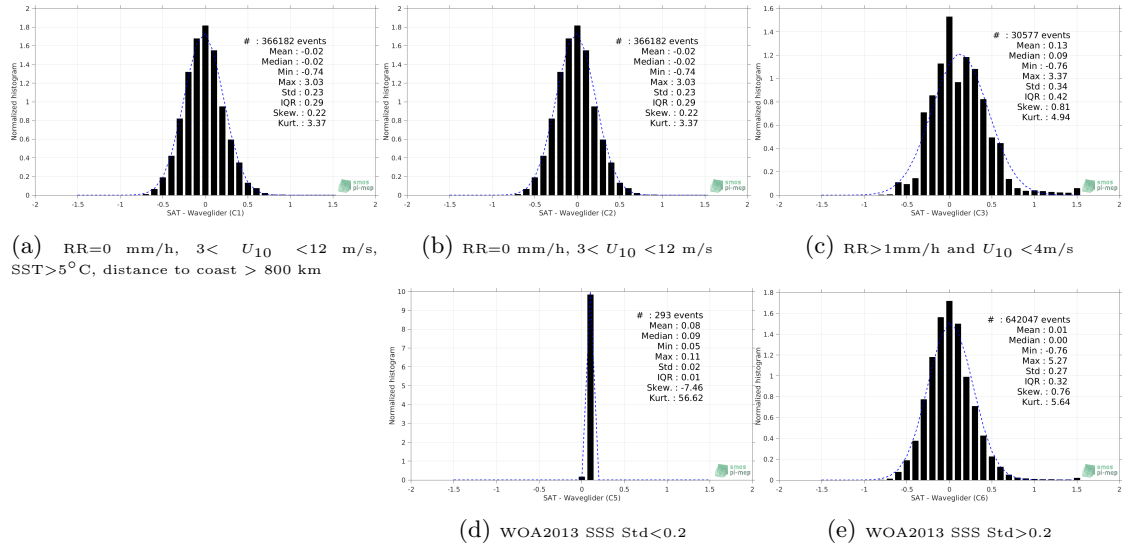
Figure 12: Normalized histogram of \Delta SSS (SMOS SSS L3 v7 - 9 Days (CATDS-CECOS-LOCEAN) - Waveglider) for 5 different subdatasets corresponding to: RR=0 mm/h, 3 < U_{10} < 12 m/s, SST>5°C, distance to coast > 800 km (a), RR=0 mm/h, 3 < U_{10} < 12 m/s (b), RR>1mm/h and U_{10} < 4 m/s (c), WOA2013 SSS Std<0.2 (d), WOA2013 SSS Std>0.2 (e).
