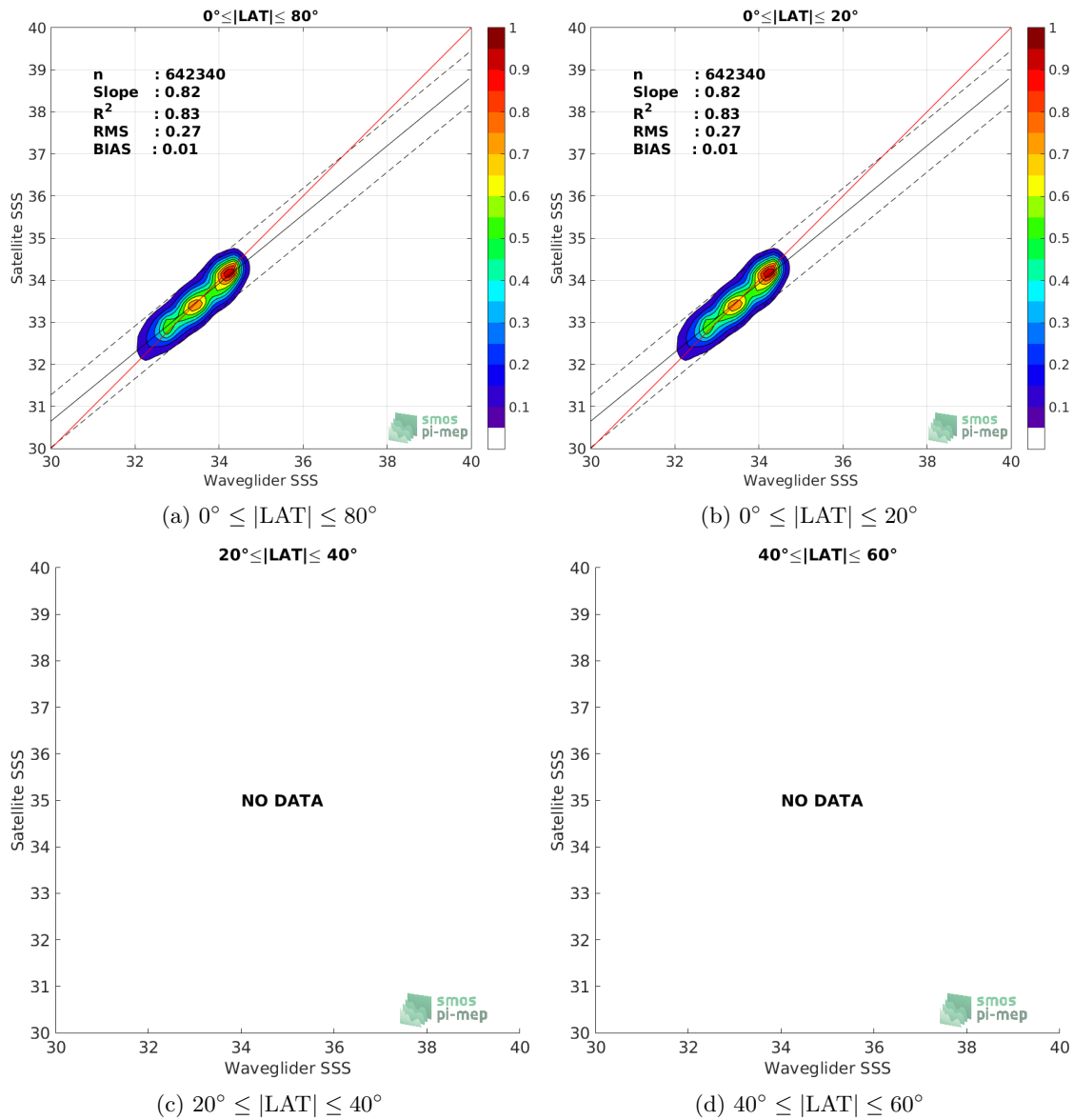
Figure 8: Contour maps of the concentration of SMOS SSS L3 v7 - 9 Days (CATDS-CECOS-LOCEAN) SSS (y-axis) versus Waveglider SSS (x-axis) at match-up pairs for different latitude bands. For each plot, the red line shows x=y . The black thin and dashed lines indicate a linear fit through the data cloud and the \pm 95\% confidence levels, respectively. The number match-up pairs n , the slope and R^2 coefficient of the linear fit, the root mean square (RMS) and the mean bias between satellite and in situ data are indicated for each latitude band in each plots.
