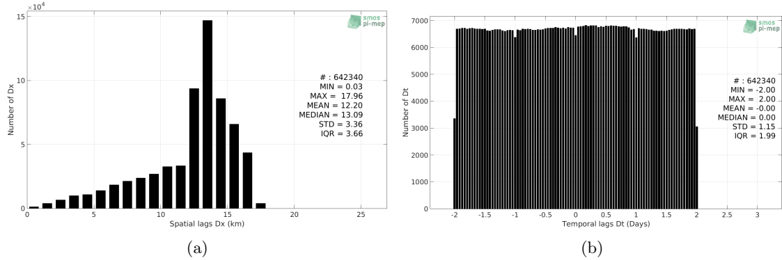
Figure 4: Histograms of the spatial (a) and temporal (b) lags between the location/time of the Waveglider measurement and the date of the corresponding SMOS SSS L3 v7 - 9 Days (CATDS-CECOS-LOCEAN) SSS pixel.
