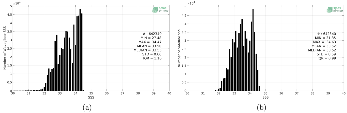
Figure 2: Histograms of SSS from Waveglider (a) and SMOS SSS L3 v7 - 9 Days (CATDS-CECOS-LOCEAN) (b) considering all match-up pairs per bins of 0.1 over the SPURS 2 Pi-MEP region and for the full satellite product period.
