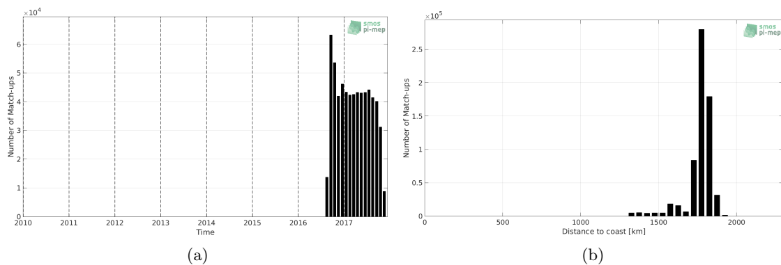
Figure 1: Number of match-ups between Waveglider and SMOS SSS L3 v7 - 9 Days (CATDS-CECOS-LOCEAN) SSS as a function of time (a) and as function of the distance to coast (b) over the SPURS 2 Pi-MEP region and for the full satellite product period.
