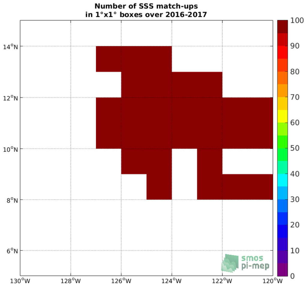
Figure 3: Number of SSS match-ups between Waveglider SSS and the SMOS SSS L3 v7 - 9 Days (CATDS-CECOS-LOCEAN) SSS product for the SPURS 2 Pi-MEP region over 1°x1° boxes and for the full satellite product period.
