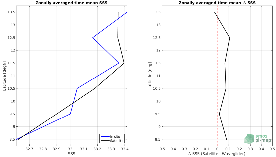
Figure 7: Left panel: Zonal mean SSS from SMOS SSS L3 v7 - 9 Days (CATDS-CECOS-LOCEAN) satellite product (black) and from Waveglider (blue). Right panel: Zonal mean of \Delta SSS (Satellite - Waveglider) for all the collected Pi-MEP match-up pairs estimated over the full satellite product period.
