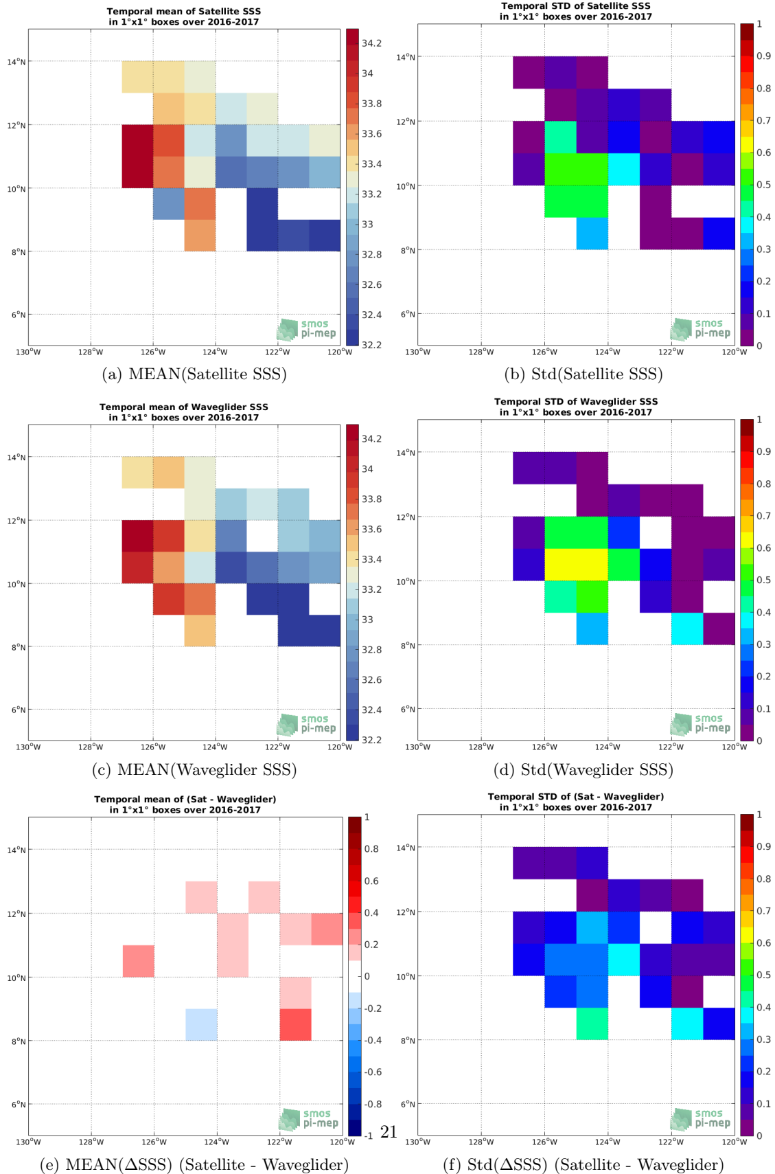
Figure 5: Temporal mean (left) and Std (right) of SSS from SMOS SSS L3 v7 - 9 Days (CATDS-CECOS-LOCEAN) (top), Waveglider (middle), and of \Delta SSS (Satellite - Waveglider). Only match-up pairs are used to generate these maps.
