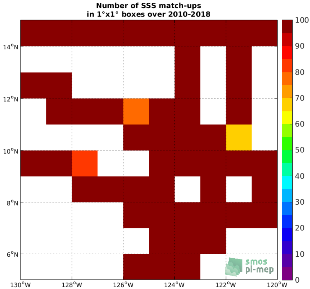
Figure 4: Number of SSS match-ups between TSG (SAMOS) SSS and the SMOS SSS L3 v7 - 9 Days (CATDS-CECOS-LOCEAN) SSS product for the SPURS 2 Pi-MEP region over 1°x1° boxes and for the full satellite product period.
