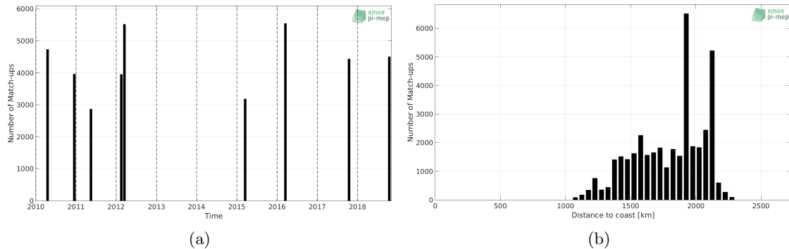
Figure 1: Number of match-ups between TSG (SAMOS) and SMOS SSS L3 v7 - 9 Days (CATDS-CECOS-LOCEAN) SSS as a function of time (a) and as function of the distance to coast (b) over the SPURS 2 Pi-MEP region and for the full satellite product period.
