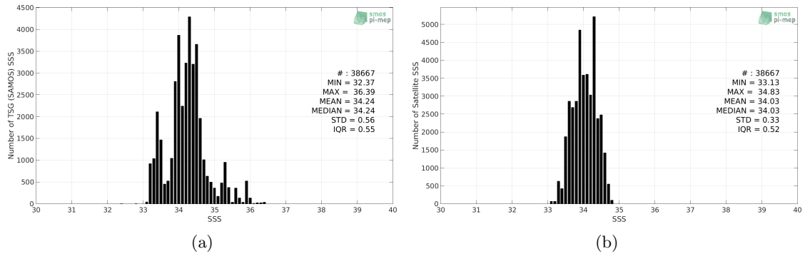
Figure 2: Histograms of SSS from TSG (SAMOS) (a) and SMOS SSS L3 v7 - 9 Days (CATDS-CECOS-LOCEAN) (b) considering all match-up pairs per bins of 0.1 over the SPURS 2 Pi-MEP region and for the full satellite product period.
