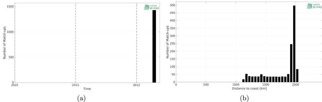
Figure 1: Number of match-ups between TSG (GOSUD-Research-vessel) and SMOS SSS L3 v7 - 9 Days (CATDS-CECOS-LOCEAN) SSS as a function of time (a) and as function of the distance to coast (b) over the SPURS 2 Pi-MEP region and for the full satellite product period.
