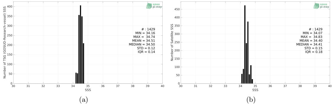
Figure 2: Histograms of SSS from TSG (GOSUD-Research-vessel) (a) and SMOS SSS L3 v7 - 9 Days (CATDS-CECOS-LOCEAN) (b) considering all match-up pairs per bins of 0.1 over the SPURS 2 Pi-MEP region and for the full satellite product period.
