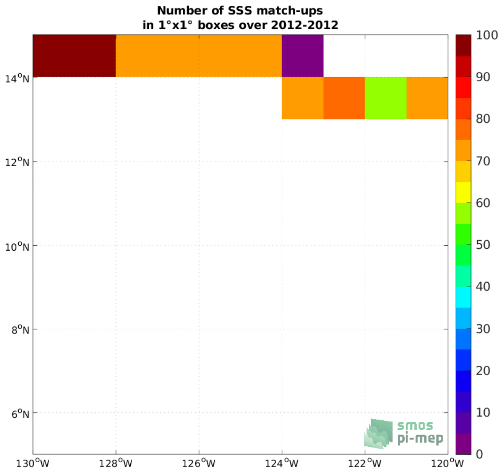
Figure 4: Number of SSS match-ups between TSG (GOSUD-Research-vessel) SSS and the SMOS SSS L3 v7 - 9 Days (CATDS-CECOS-LOCEAN) SSS product for the SPURS 2 Pi-MEP region over 1^\circ \times 1^\circ boxes and for the full satellite product period.
