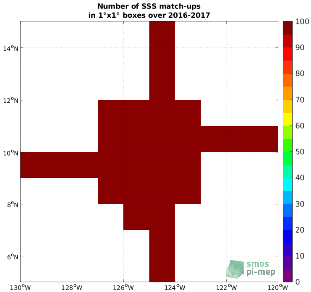
Figure 4: Number of SSS match-ups between Salinity Snake SSS and the SMOS SSS L3 v7 - 9 Days (CATDS-CECOS-LOCEAN) SSS product for the SPURS 2 Pi-MEP region over 1°x1° boxes and for the full satellite product period.
