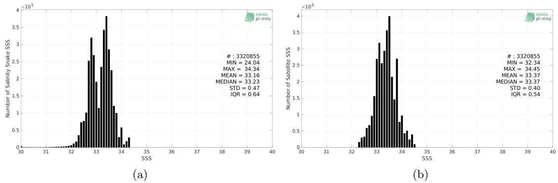
Figure 2: Histograms of SSS from Salinity Snake (a) and SMOS SSS L3 v7 - 9 Days (CATDS-CECOS-LOCEAN) (b) considering all match-up pairs per bins of 0.1 over the SPURS 2 Pi-MEP region and for the full satellite product period.
