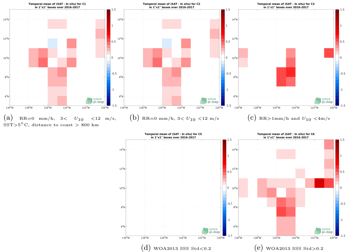
Figure 12: Temporal mean gridded over spatial boxes of size 1^\circ \times 1^\circ of \Delta SSS (SMOS SSS L3 v7 - 9 Days (CATDS-CECOS-LOCEAN) - Salinity Snake) for 5 different subdatasets corresponding to:RR=0 mm/h, 3 < U_{10} < 12 m/s, SST >5^\circ C, distance to coast > 800 km (a), RR=0 mm/h, 3 < U_{10} < 12 m/s (b), RR >1 mm/h and U_{10} < 4 m/s (c), WOA2013 SSS Std <0.2 (d), WOA2013 SSS Std >0.2 (e).
