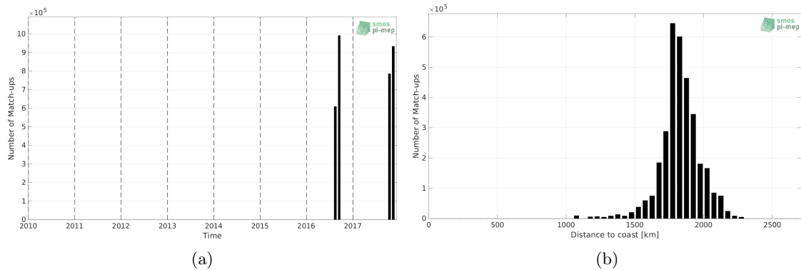
Figure 1: Number of match-ups between Salinity Snake and SMOS SSS L3 v7 - 9 Days (CATDS-CECOS-LOCEAN) SSS as a function of time (a) and as function of the distance to coast (b) over the SPURS 2 Pi-MEP region and for the full satellite product period.
