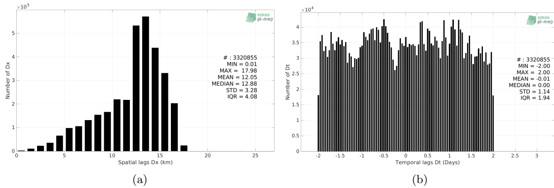
Figure 5: Histograms of the spatial (a) and temporal (b) lags between the location/time of the Salinity Snake measurement and the date of the corresponding SMOS SSS L3 v7 - 9 Days (CATDS-CECOS-LOCEAN) SSS pixel.
