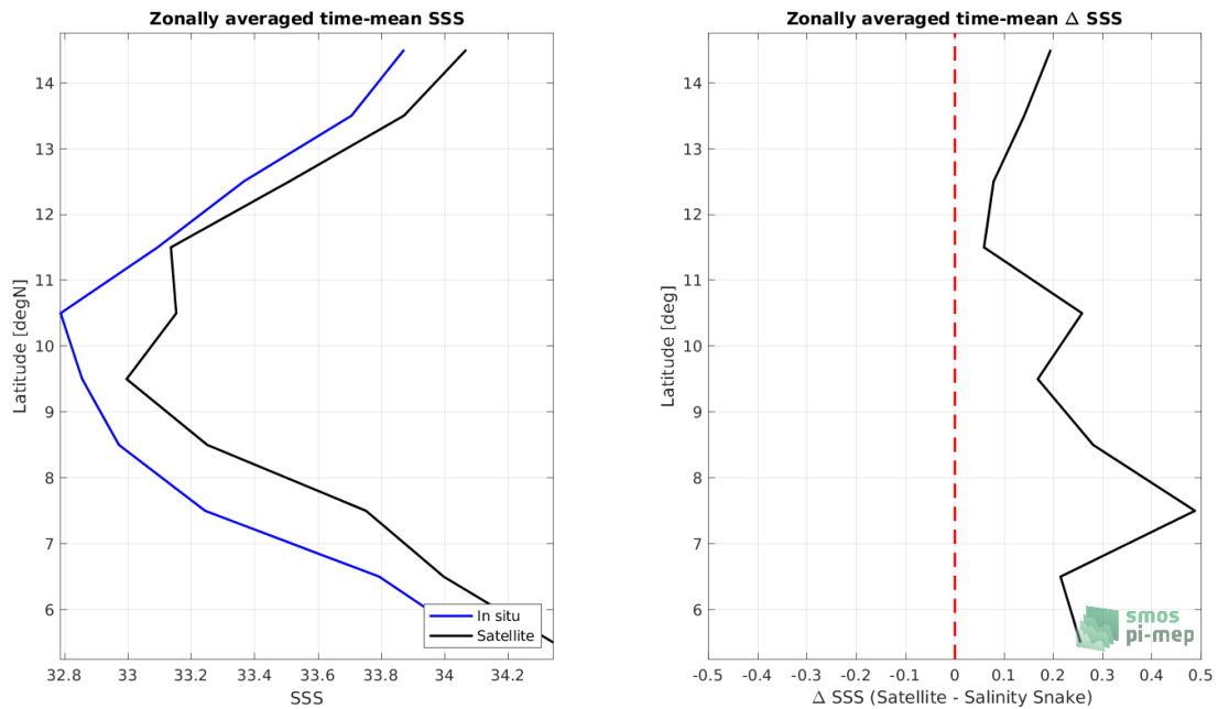
Figure 8: Left panel: Zonal mean SSS from SMOS SSS L3 v7 - 9 Days (CATDS-CECOS-LOCEAN) satellite product (black) and from Salinity Snake (blue). Right panel: Zonal mean of \Delta SSS (Satellite - Salinity Snake) for all the collected Pi-MEP match-up pairs estimated over the full satellite product period.
