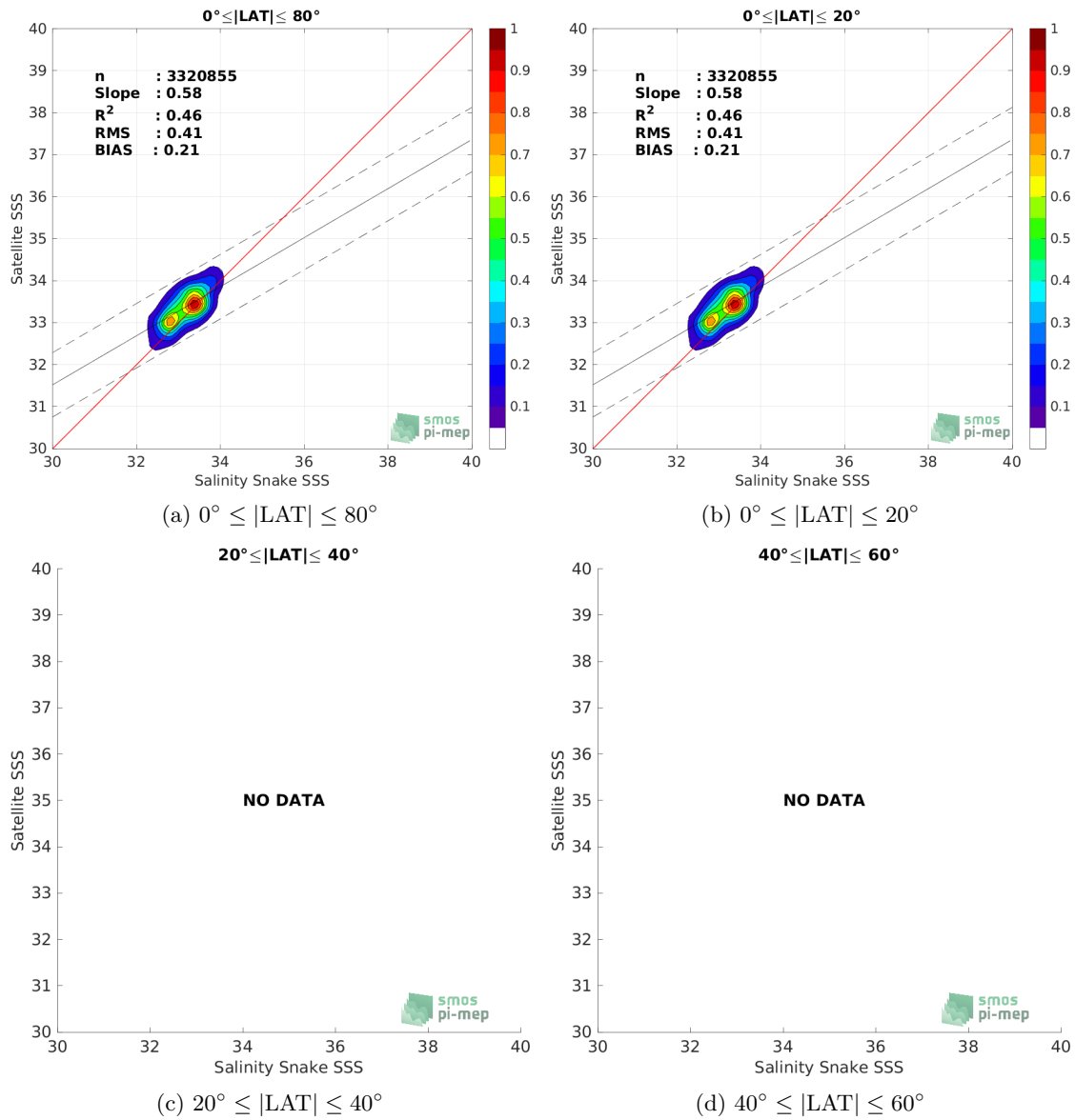
Figure 9: Contour maps of the concentration of SMOS SSS L3 v7 - 9 Days (CATDS-CECOS-LOCEAN) SSS (y-axis) versus Salinity Snake SSS (x-axis) at match-up pairs for different latitude bands. For each plot, the red line shows x=y . The black thin and dashed lines indicate a linear fit through the data cloud and the \pm 95\% confidence levels, respectively. The number match-up pairs n , the slope and R^2 coefficient of the linear fit, the root mean square (RMS) and the mean bias between satellite and in situ data are indicated for each latitude band in each plots.
