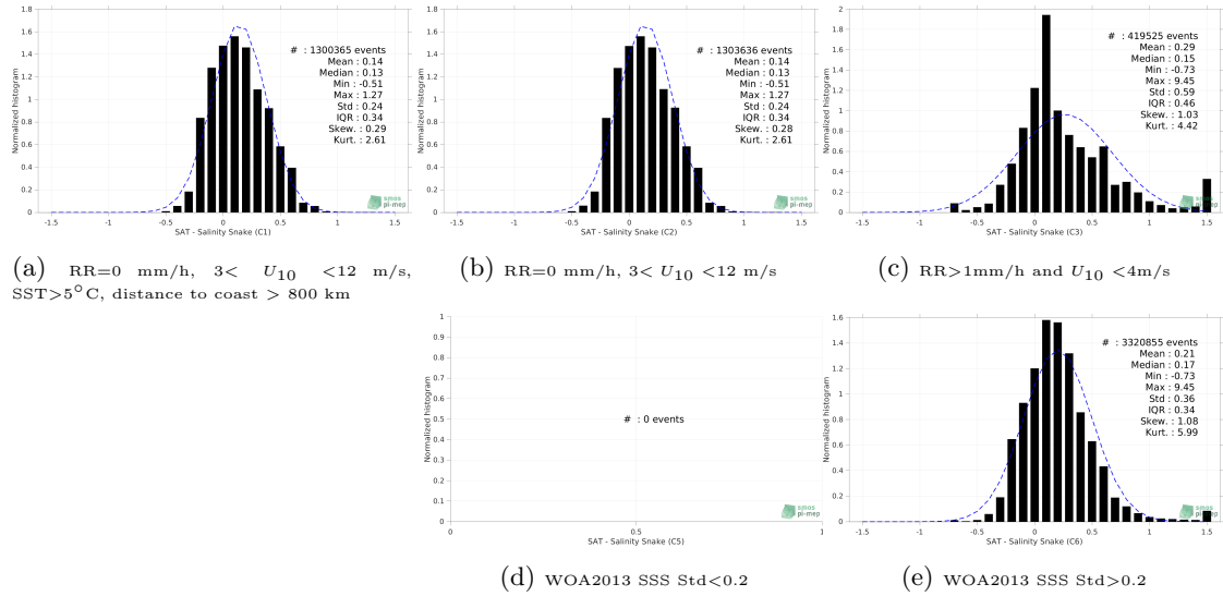
Figure 13: Normalized histogram of \Delta SSS (SMOS SSS L3 v7 - 9 Days (CATDS-CECOS-LOCEAN) - Salinity Snake) for 5 different subdatasets corresponding to: RR=0 mm/h, 3 < U_{10} < 12 m/s, SST > 5°C, distance to coast > 800 km (a), RR=0 mm/h, 3 < U_{10} < 12 m/s (b), RR > 1mm/h and U_{10} < 4 m/s (c), WOA2013 SSS Std < 0.2 (d), WOA2013 SSS Std > 0.2 (e).
