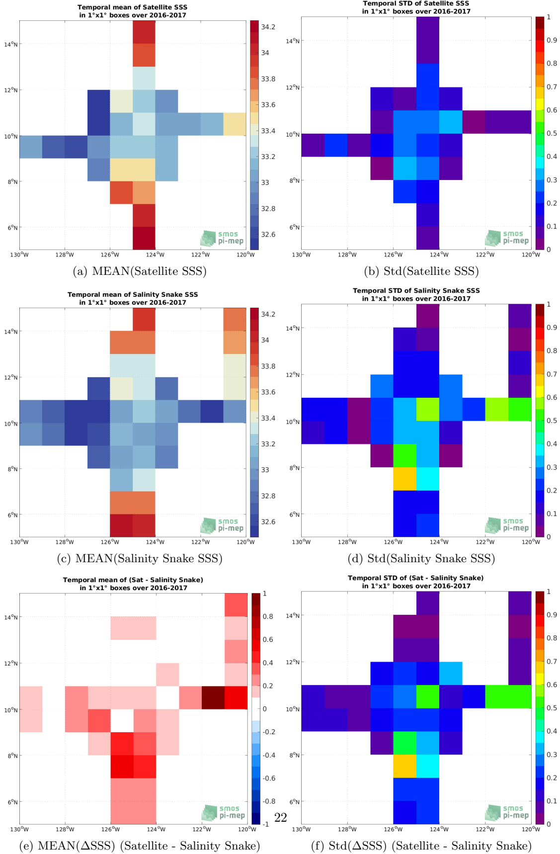
Figure 6: Temporal mean (left) and Std (right) of SSS from SMOS SSS L3 v7 - 9 Days (CATDS-CECOS-LOCEAN) (top), Salinity Snake (middle), and of \Delta SSS (Satellite - Salinity Snake). Only match-up pairs are used to generate these maps.
