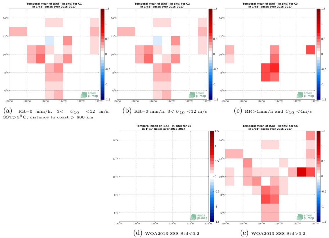
Figure 11: Temporal mean gridded over spatial boxes of size 1^\circ \times 1^\circ of \Delta SSS (SMOS SSS L3 v7 - 9 Days (CATDS-CECOS-LOCEAN) - Salinity Snake) for 5 different subdatasets corresponding to:RR=0 mm/h, 3 < U_{10} < 12 m/s, SST >5^\circ\text{C} , distance to coast > 800 km (a), RR=0 mm/h, 3 < U_{10} < 12 m/s (b), RR >1 mm/h and U_{10} < 4 m/s (c), WOA2013 SSS Std <0.2 (d), WOA2013 SSS Std >0.2 (e).
