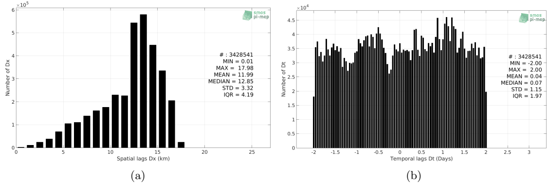
Figure 4: Histograms of the spatial (a) and temporal (b) lags between the location/time of the Salinity Snake measurement and the date of the corresponding SMOS SSS L3 v7 - 9 Days (CATDS-CECOS-LOCEAN) SSS pixel.
