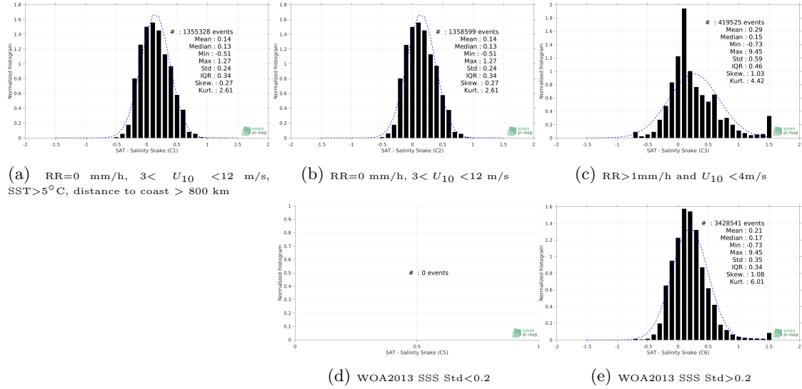
Figure 12: Normalized histogram of \Delta SSS (SMOS SSS L3 v7 - 9 Days (CATDS-CECOS-LOCEAN) - Salinity Snake) for 5 different subdatasets corresponding to: RR=0 mm/h, 3 < U_{10} < 12 m/s, SST > 5°C, distance to coast > 800 km (a), RR=0 mm/h, 3 < U_{10} < 12 m/s (b), RR > 1mm/h and U_{10} < 4 m/s (c), WOA2013 SSS Std < 0.2 (d), WOA2013 SSS Std > 0.2 (e).
