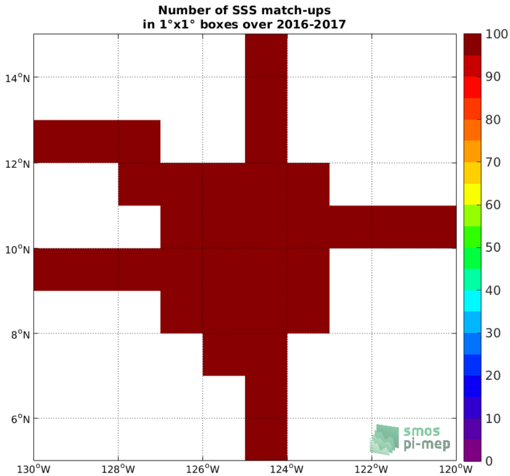
Figure 3: Number of SSS match-ups between Salinity Snake SSS and the SMOS SSS L3 v7 - 9 Days (CATDS-CECOS-LOCEAN) SSS product for the SPURS 2 Pi-MEP region over 1°x1° boxes and for the full satellite product period.
