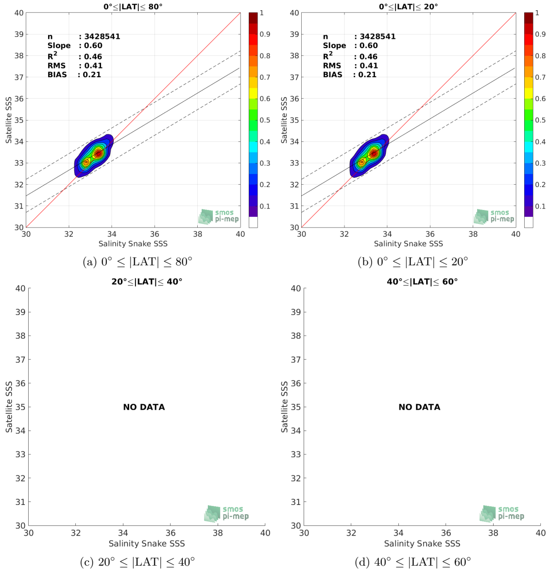
Figure 8: Contour maps of the concentration of SMOS SSS L3 v7 - 9 Days (CATDS-CECOS-LOCEAN) SSS (y-axis) versus Salinity Snake SSS (x-axis) at match-up pairs for different latitude bands. For each plot, the red line shows x=y . The black thin and dashed lines indicate a linear fit through the data cloud and the \pm 95\% confidence levels, respectively. The number match-up pairs n , the slope and R^2 coefficient of the linear fit, the root mean square (RMS) and the mean bias between satellite and in situ data are indicated for each latitude band in each plots.
