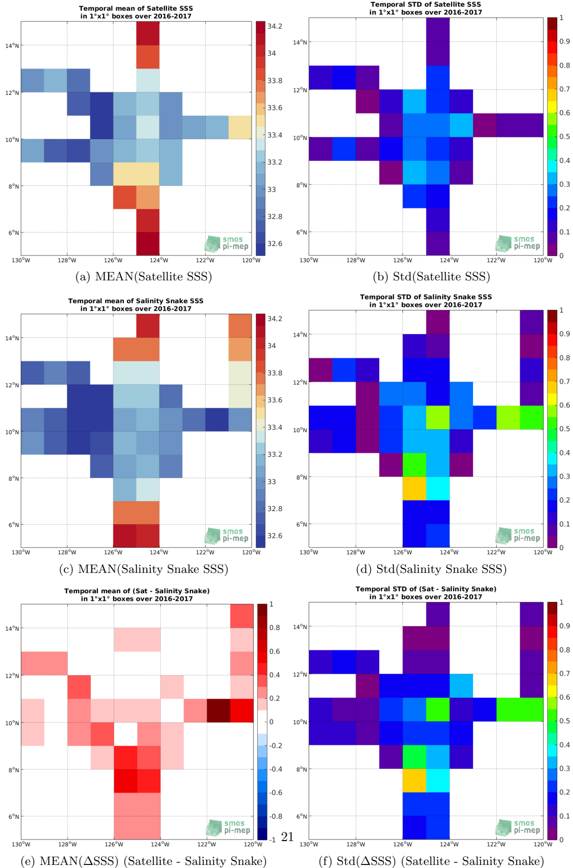
Figure 5: Temporal mean (left) and Std (right) of SSS from SMOS SSS L3 v7 - 9 Days (CATDS-CECOS-LOCEAN) (top), Salinity Snake (middle), and of \Delta SSS (Satellite - Salinity Snake). Only match-up pairs are used to generate these maps.
