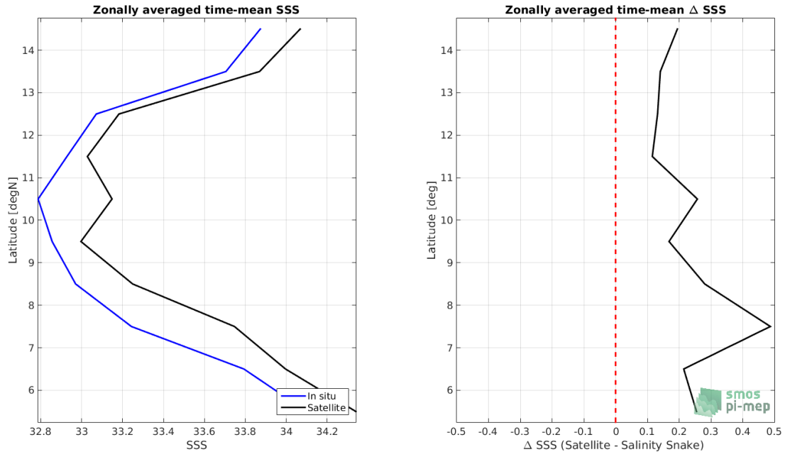
Figure 7: Left panel: Zonal mean SSS from SMOS SSS L3 v7 - 9 Days (CATDS-CECOS-LOCEAN) satellite product (black) and from Salinity Snake (blue). Right panel: Zonal mean of \Delta SSS (Satellite - Salinity Snake) for all the collected Pi-MEP match-up pairs estimated over the full satellite product period.
