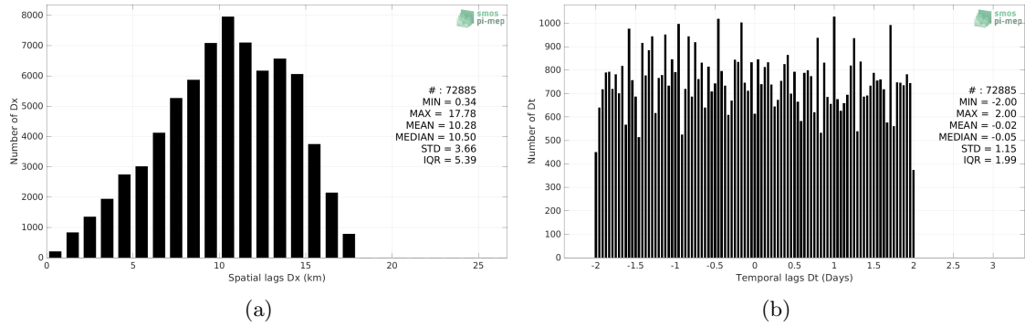
Figure 5: Histograms of the spatial (a) and temporal (b) lags between the location/time of the Seaglider measurement and the date of the corresponding SMOS SSS L3 v7 - 9 Days (CATDS-CECOS-LOCEAN) SSS pixel.
