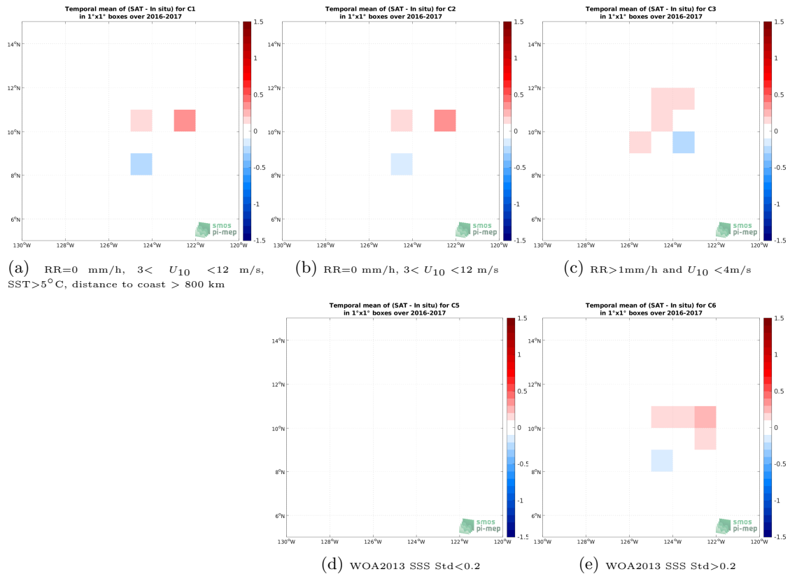
Figure 12: Temporal mean gridded over spatial boxes of size 1^\circ \times 1^\circ of \Delta SSS (SMOS SSS L3 v7 - 9 Days (CATDS-CECOS-LOCEAN) - Seaglider) for 5 different subdatasets corresponding to:RR=0 mm/h, 3 < U_{10} < 12 m/s, SST >5^\circ\text{C} , distance to coast > 800 km (a), RR=0 mm/h, 3 < U_{10} < 12 m/s (b), RR >1 mm/h and U_{10} < 4 m/s (c), WOA2013 SSS Std <0.2 (d), WOA2013 SSS Std >0.2 (e).
