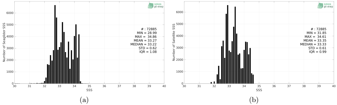
Figure 2: Histograms of SSS from Seaglider (a) and SMOS SSS L3 v7 - 9 Days (CATDS-CECOS-LOCEAN) (b) considering all match-up pairs per bins of 0.1 over the SPURS 2 Pi-MEP region and for the full satellite product period.
