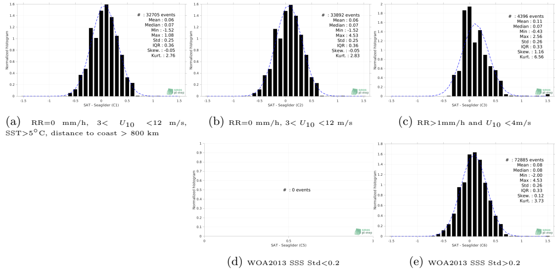
Figure 13: Normalized histogram of \Delta SSS (SMOS SSS L3 v7 - 9 Days (CATDS-CECOS-LOCEAN) - Seaglider) for 5 different subdatasets corresponding to: RR=0 mm/h, 3 < U_{10} < 12 m/s, SST>5°C, distance to coast > 800 km (a), RR=0 mm/h, 3 < U_{10} < 12 m/s (b), RR>1mm/h and U_{10} < 4 m/s (c), WOA2013 SSS Std<0.2 (d), WOA2013 SSS Std>0.2 (e).
