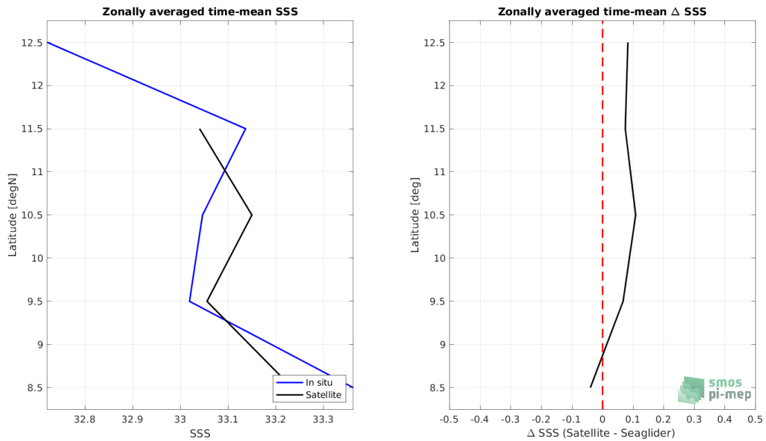
Figure 8: Left panel: Zonal mean SSS from SMOS SSS L3 v7 - 9 Days (CATDS-CECOS-LOCEAN) satellite product (black) and from Seaglider (blue). Right panel: Zonal mean of \Delta SSS (Satellite - Seaglider) for all the collected Pi-MEP match-up pairs estimated over the full satellite product period.
