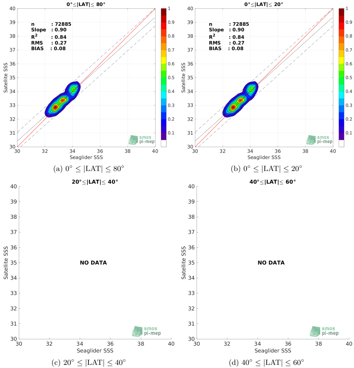
Figure 9: Contour maps of the concentration of SMOS SSS L3 v7 - 9 Days (CATDS-CECOS-LOCEAN) SSS (y-axis) versus Seaglider SSS (x-axis) at match-up pairs for different latitude bands. For each plot, the red line shows x=y . The black thin and dashed lines indicate a linear fit through the data cloud and the \pm 95\% confidence levels, respectively. The number match-up pairs n , the slope and R^2 coefficient of the linear fit, the root mean square (RMS) and the mean bias between satellite and in situ data are indicated for each latitude band in each plots.
