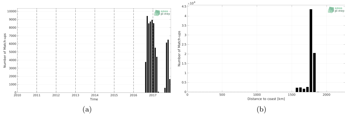
Figure 1: Number of match-ups between Seaglider and SMOS SSS L3 v7 - 9 Days (CATDS-CECOS-LOCEAN) SSS as a function of time (a) and as function of the distance to coast (b) over the SPURS 2 Pi-MEP region and for the full satellite product period.
