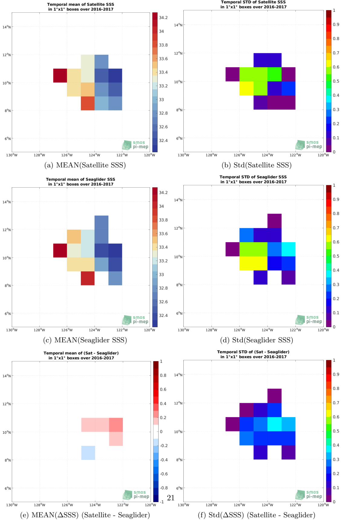
Figure 6: Temporal mean (left) and Std (right) of SSS from SMOS SSS L3 v7 - 9 Days (CATDS-CECOS-LOCEAN) (top), Seaglider (middle), and of \Delta SSS (Satellite - Seaglider). Only match-up pairs are used to generate these maps.
