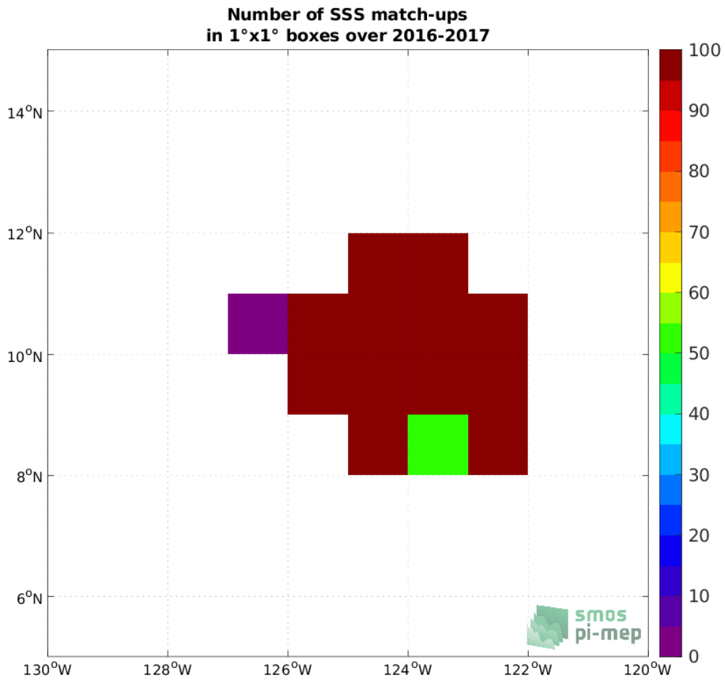
Figure 3: Number of SSS match-ups between Seaglider SSS and the SMOS SSS L3 v7 - 9 Days (CATDS-CECOS-LOCEAN) SSS product for the SPURS 2 Pi-MEP region over 1°x1° boxes and for the full satellite product period.
