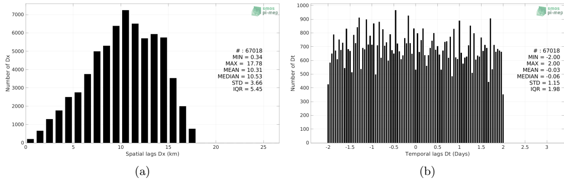
Figure 4: Histograms of the spatial (a) and temporal (b) lags between the location/time of the Seaglider measurement and the date of the corresponding SMOS SSS L3 v7 - 9 Days (CATDS-CECOS-LOCEAN) SSS pixel.
