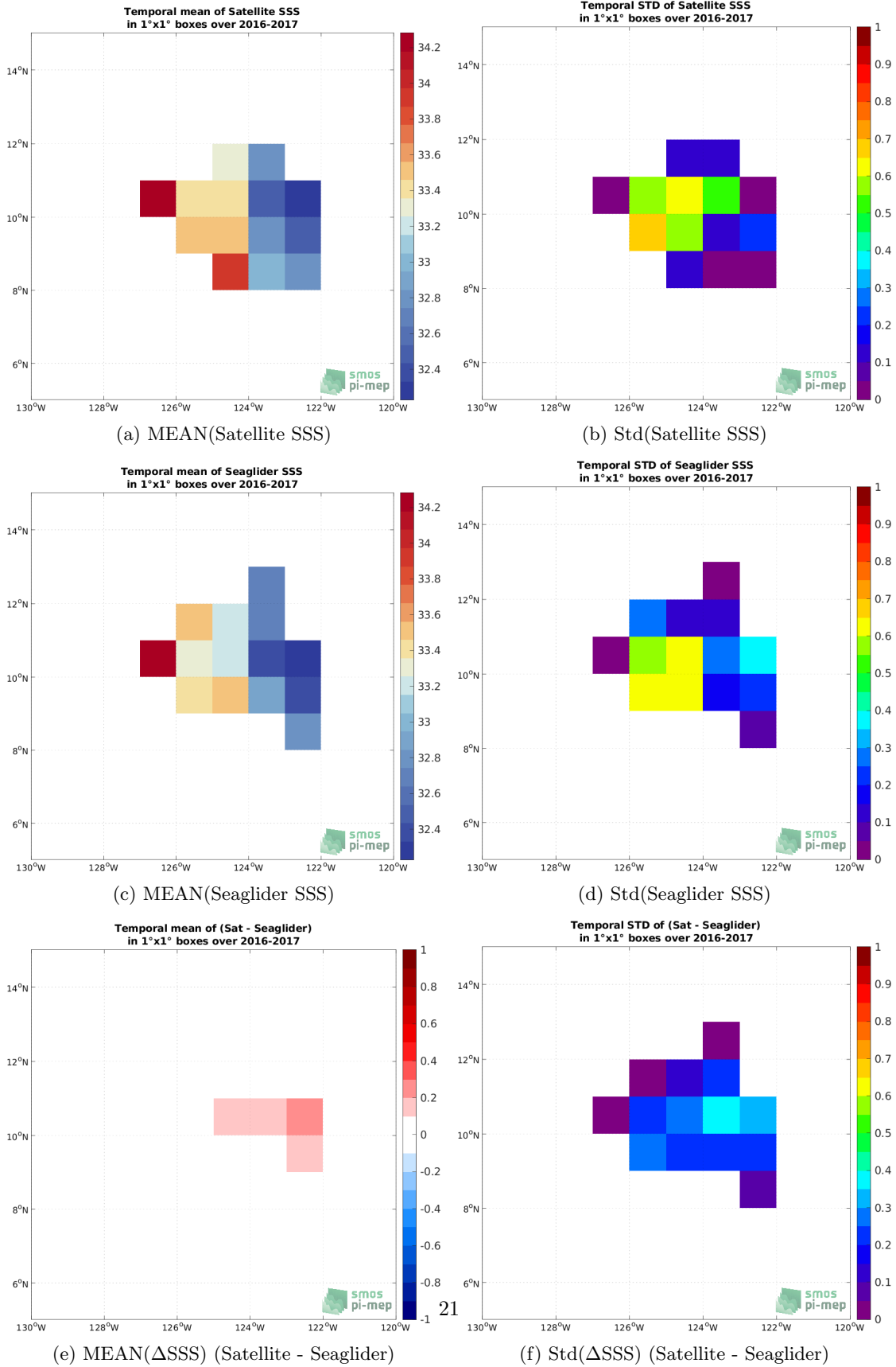
Figure 5: Temporal mean (left) and Std (right) of SSS from SMOS SSS L3 v7 - 9 Days (CATDS-CECOS-LOCEAN) (top), Seaglider (middle), and of \Delta SSS (Satellite - Seaglider). Only match-up pairs are used to generate these maps.
