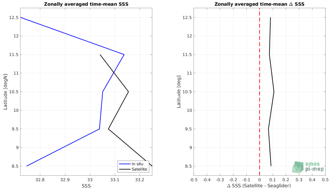
Figure 7: Left panel: Zonal mean SSS from SMOS SSS L3 v7 - 9 Days (CATDS-CECOS-LOCEAN) satellite product (black) and from Seaglider (blue). Right panel: Zonal mean of \Delta SSS (Satellite - Seaglider) for all the collected Pi-MEP match-up pairs estimated over the full satellite product period.
