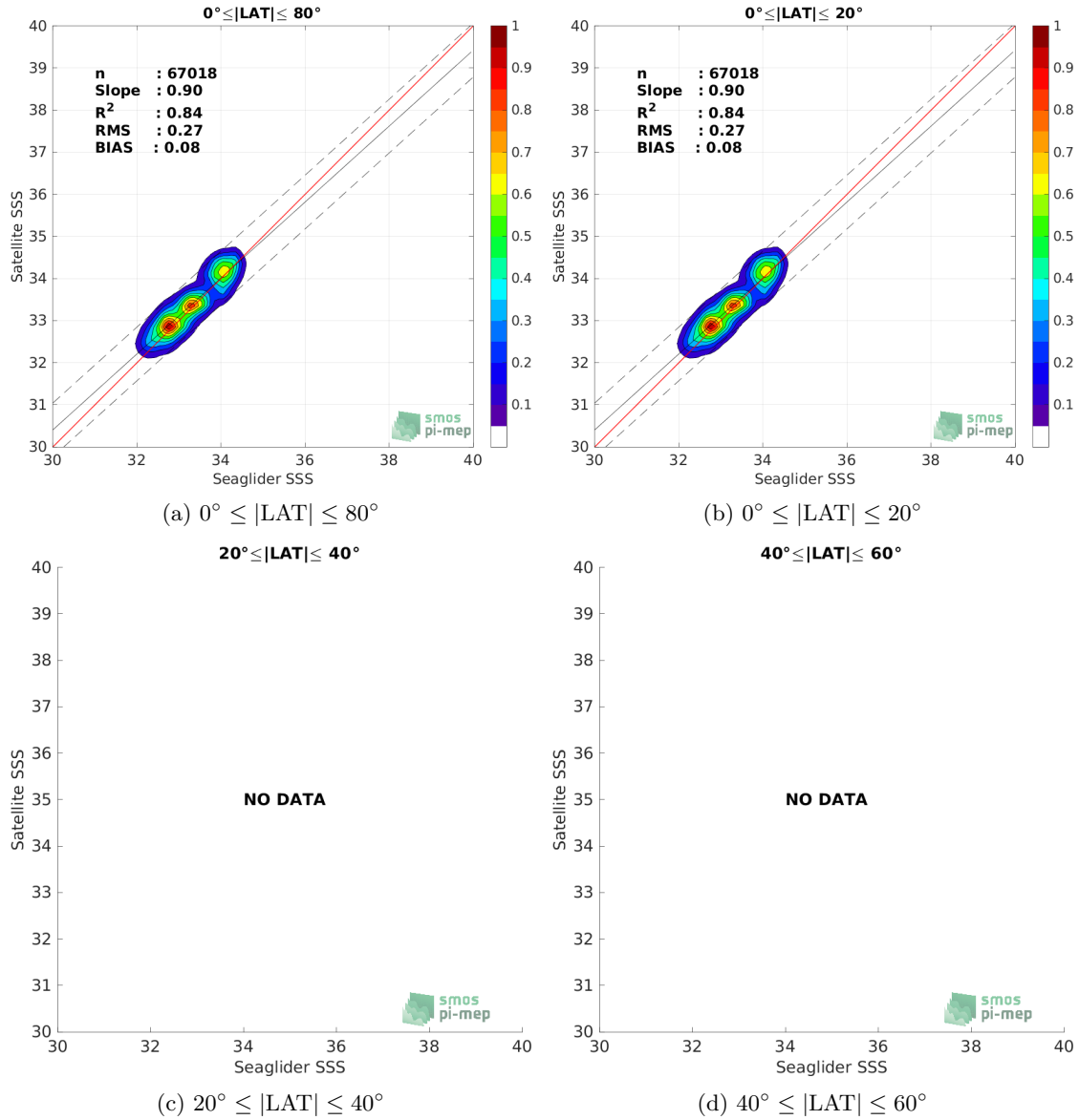
Figure 8: Contour maps of the concentration of SMOS SSS L3 v7 - 9 Days (CATDS-CECOS-LOCEAN) SSS (y-axis) versus Seaglider SSS (x-axis) at match-up pairs for different latitude bands. For each plot, the red line shows x=y . The black thin and dashed lines indicate a linear fit through the data cloud and the \pm 95\% confidence levels, respectively. The number match-up pairs n , the slope and R^2 coefficient of the linear fit, the root mean square (RMS) and the mean bias between satellite and in situ data are indicated for each latitude band in each plots.
