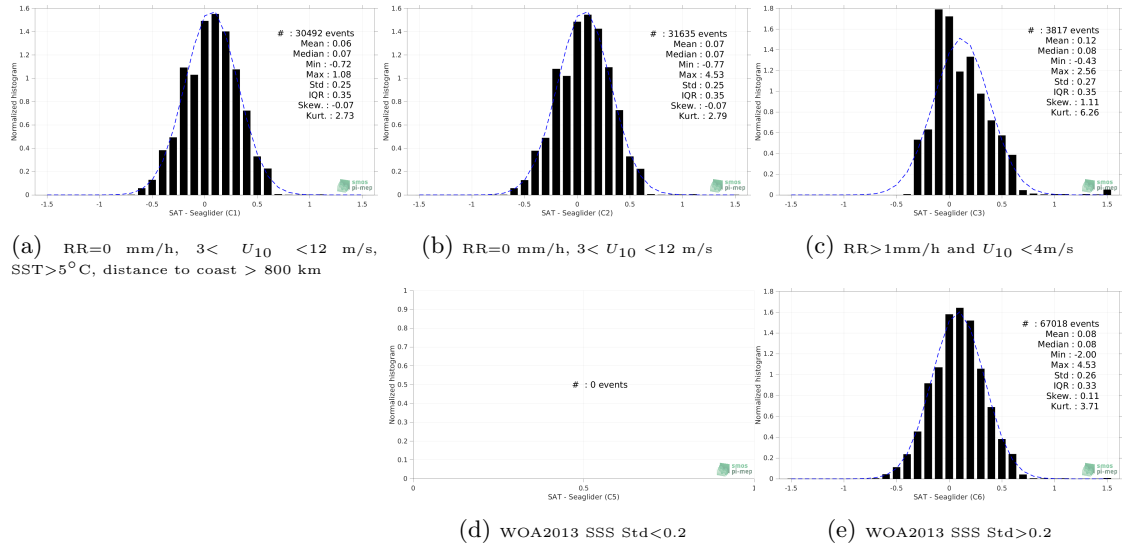
Figure 12: Normalized histogram of \Delta SSS (SMOS SSS L3 v7 - 9 Days (CATDS-CECOS-LOCEAN) - Seaglider) for 5 different subdatasets corresponding to: RR=0 mm/h, 3 < U_{10} < 12 m/s, SST>5°C, distance to coast > 800 km (a), RR=0 mm/h, 3 < U_{10} < 12 m/s (b), RR>1mm/h and U_{10} < 4 m/s (c), WOA2013 SSS Std<0.2 (d), WOA2013 SSS Std>0.2 (e).
