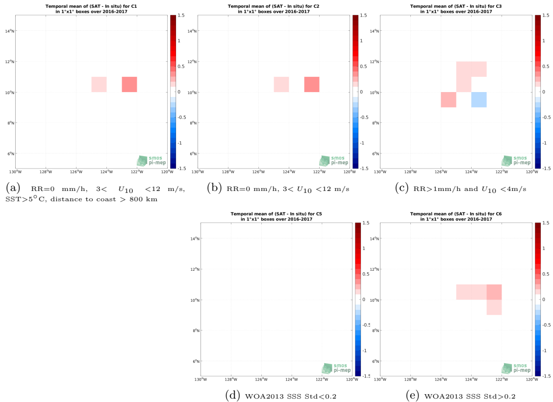
Figure 11: Temporal mean gridded over spatial boxes of size 1^\circ \times 1^\circ of \Delta SSS (SMOS SSS L3 v7 - 9 Days (CATDS-CECOS-LOCEAN) - Seaglider) for 5 different subdatasets corresponding to:RR=0 mm/h, 3 < U_{10} < 12 m/s, SST >5^\circ\text{C} , distance to coast > 800 km (a), RR=0 mm/h, 3 < U_{10} < 12 m/s (b), RR >1 mm/h and U_{10} < 4 m/s (c), WOA2013 SSS Std <0.2 (d), WOA2013 SSS Std >0.2 (e).
