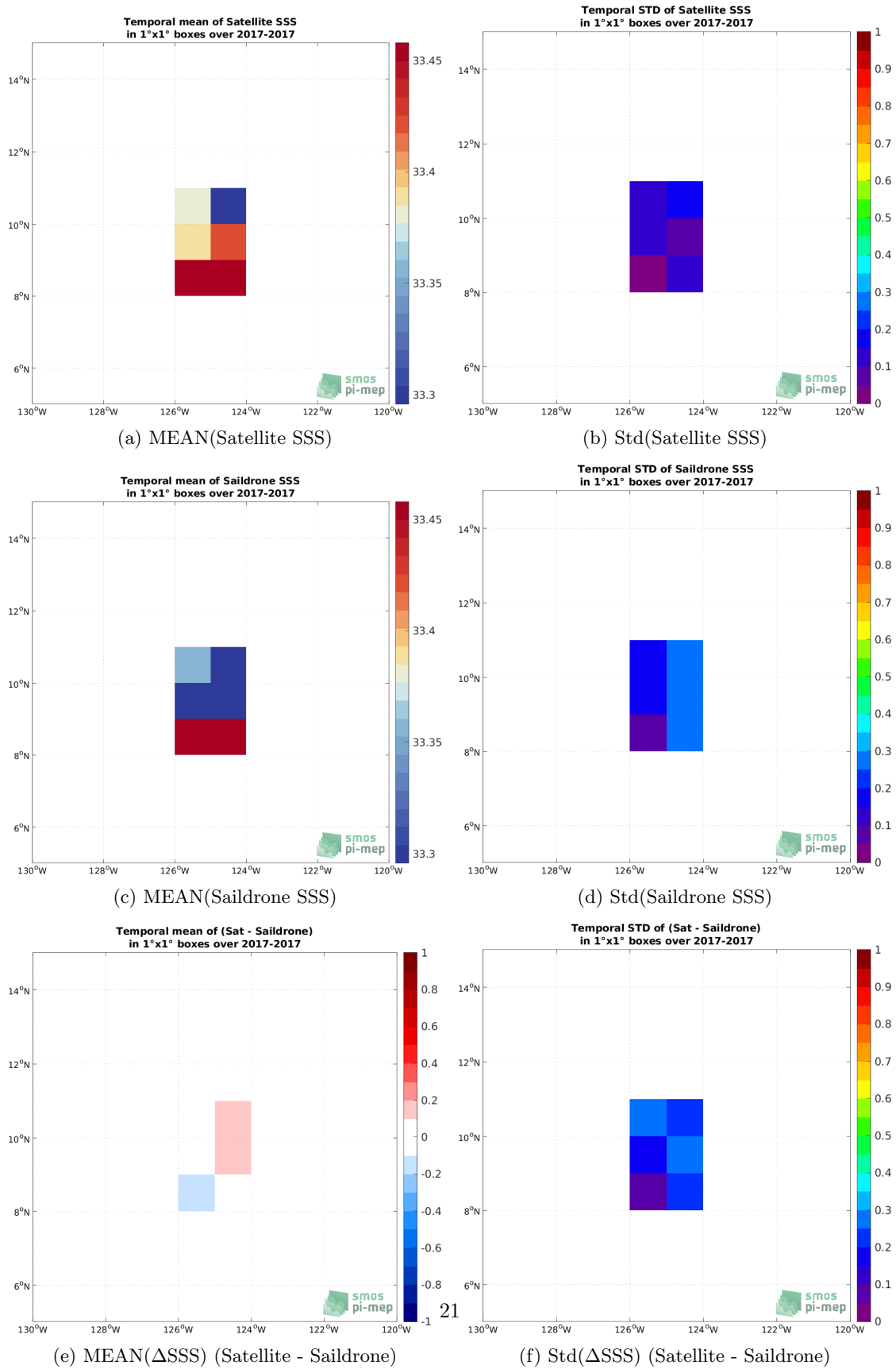
Figure 6: Temporal mean (left) and Std (right) of SSS from SMOS SSS L3 v7 - 9 Days (CATDS-CECOS-LOCEAN) (top), Saildrone (middle), and of \Delta SSS (Satellite - Saildrone). Only match-pairs are used to generate these maps.
