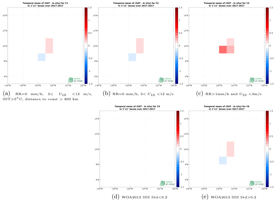
Figure 12: Temporal mean gridded over spatial boxes of size 1^\circ \times 1^\circ of \Delta SSS (SMOS SSS L3 v7 - 9 Days (CATDS-CECOS-LOCEAN) - Saildrone) for 5 different subdatasets corresponding to:RR=0 mm/h, 3 < U_{10} < 12 m/s, SST >5^\circ C, distance to coast > 800 km (a), RR=0 mm/h, 3 < U_{10} < 12 m/s (b), RR >1 mm/h and U_{10} < 4 m/s (c), WOA2013 SSS Std <0.2 (d), WOA2013 SSS Std >0.2 (e).
