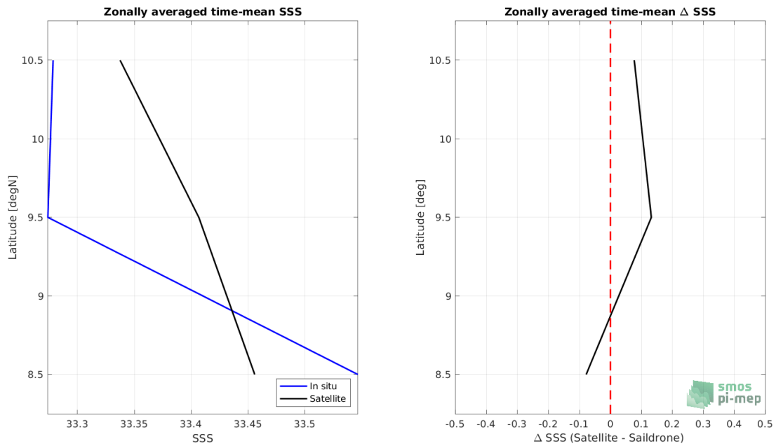
Figure 8: Left panel: Zonal mean SSS from SMOS SSS L3 v7 - 9 Days (CATDS-CECOS-LOCEAN) satellite product (black) and from Sairdrone (blue). Right panel: Zonal mean of \Delta SSS (Satellite - Sairdrone) for all the collected Pi-MEP match-up pairs estimated over the full satellite product period.
