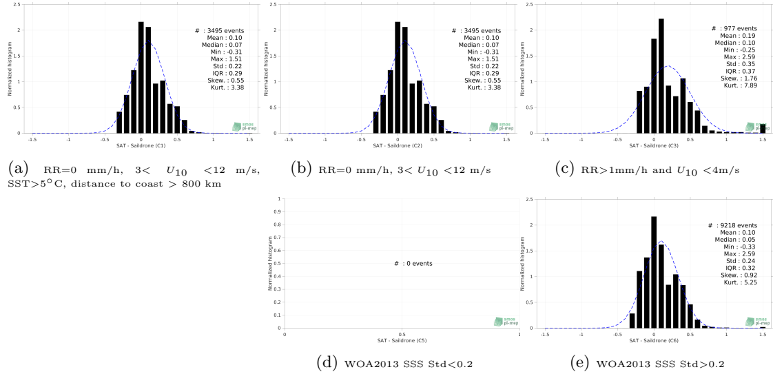
Figure 13: Normalized histogram of \Delta SSS (SMOS SSS L3 v7 - 9 Days (CATDS-CECOS-LOCEAN) - Saildrone) for 5 different subdatasets corresponding to: RR=0 mm/h, 3 < U_{10} < 12 m/s, SST > 5°C, distance to coast > 800 km (a), RR=0 mm/h, 3 < U_{10} < 12 m/s (b), RR > 1mm/h and U_{10} < 4 m/s (c), WOA2013 SSS Std < 0.2 (d), WOA2013 SSS Std > 0.2 (e).
