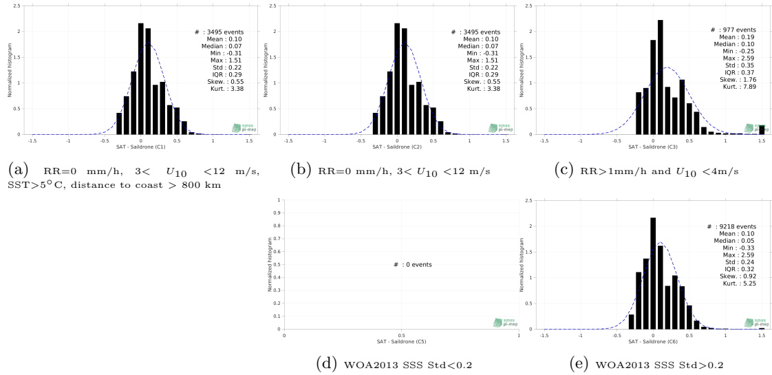
Figure 12: Normalized histogram of \Delta SSS (SMOS SSS L3 v7 - 9 Days (CATDS-CECOS-LOCEAN) - Saildrone) for 5 different subdatasets corresponding to: RR=0 mm/h, 3 < U_{10} < 12 m/s, SST > 5°C, distance to coast > 800 km (a), RR=0 mm/h, 3 < U_{10} < 12 m/s (b), RR > 1mm/h and U_{10} < 4 m/s (c), WOA2013 SSS Std < 0.2 (d), WOA2013 SSS Std > 0.2 (e).
