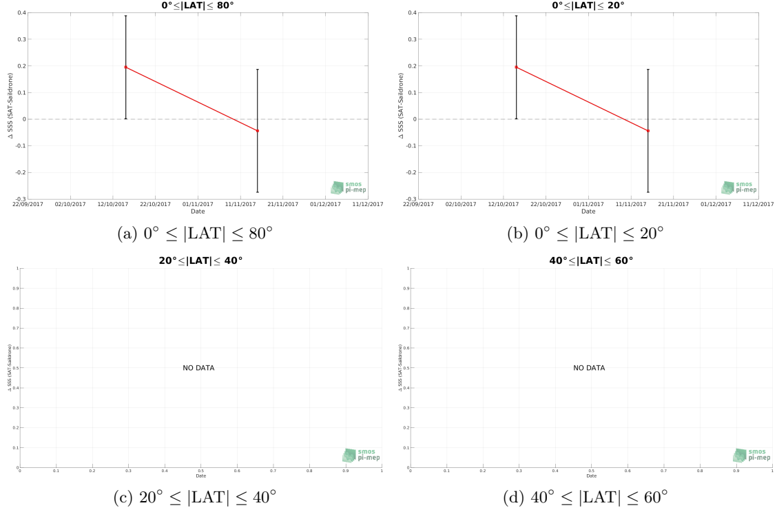
Figure 9: Monthly median (red curves) of \Delta SSS (Satellite - Saildrone) and \pm 1 Std (black vertical thick bars) as function of time for all the collected Pi-MEP match-up pairs estimated over the SPURS 2 Pi-MEP region and for the full satellite product period are shown for different latitude bands: (a) 80°S-80°N, (b) 20°S-20°N, (c) 40°S-20°S and 20°N-40°N and (d) 60°S-40°S and 40°N-60°N.
