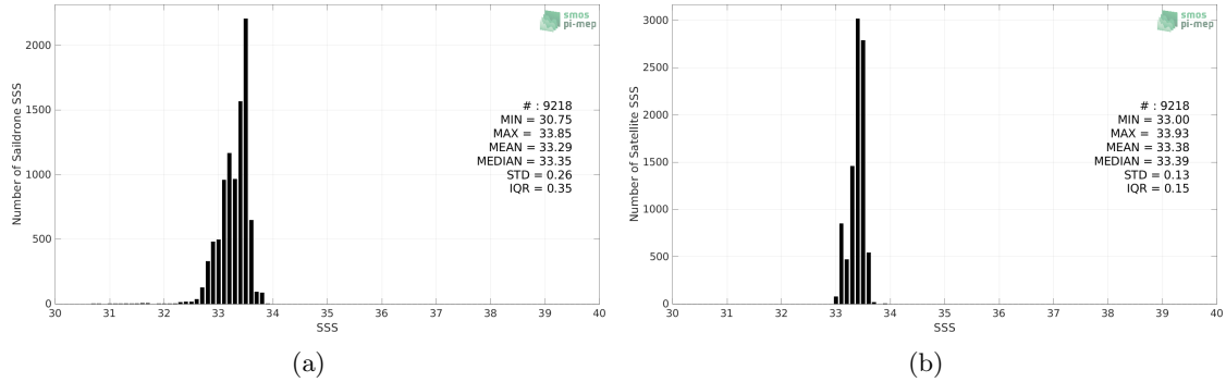
Figure 2: Histograms of SSS from Saildrone (a) and SMOS SSS L3 v7 - 9 Days (CATDS-CECOS-LOCEAN) (b) considering all match-up pairs per bins of 0.1 over the SPURS 2 Pi-MEP region and for the full satellite product period.
