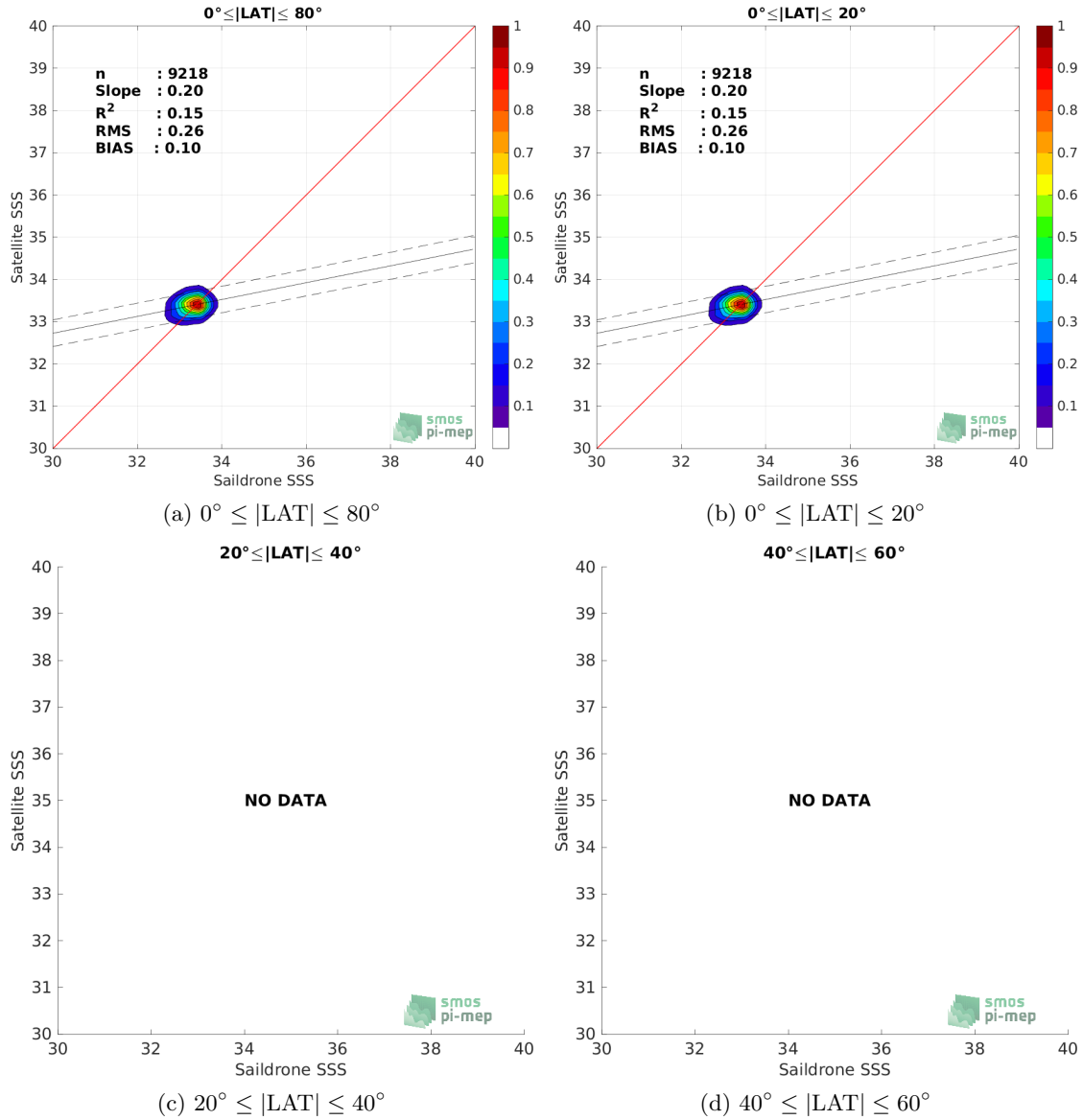
Figure 8: Contour maps of the concentration of SMOS SSS L3 v7 - 9 Days (CATDS-CECOS-LOCEAN) SSS (y-axis) versus SAILDRONE SSS (x-axis) at match-up pairs for different latitude bands. For each plot, the red line shows x=y . The black thin and dashed lines indicate a linear fit through the data cloud and the \pm 95\% confidence levels, respectively. The number match-up pairs n , the slope and R^2 coefficient of the linear fit, the root mean square (RMS) and the mean bias between satellite and in situ data are indicated for each latitude band in each plots.
