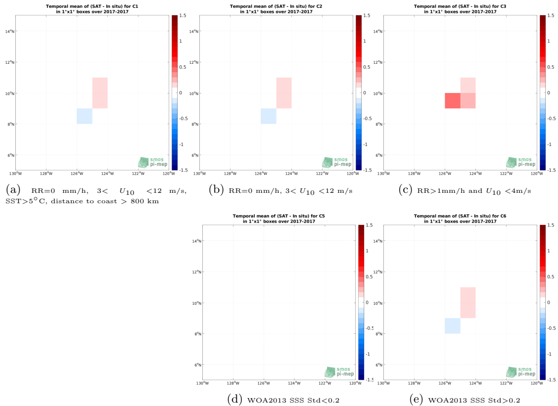
Figure 11: Temporal mean gridded over spatial boxes of size 1^\circ \times 1^\circ of \Delta SSS (SMOS SSS L3 v7 - 9 Days (CATDS-CECOS-LOCEAN) - Saildrone) for 5 different subdatasets corresponding to:RR=0 mm/h, 3 < U_{10} < 12 m/s, SST >5^\circ C, distance to coast > 800 km (a), RR=0 mm/h, 3 < U_{10} < 12 m/s (b), RR >1 mm/h and U_{10} < 4 m/s (c), WOA2013 SSS Std <0.2 (d), WOA2013 SSS Std >0.2 (e).
