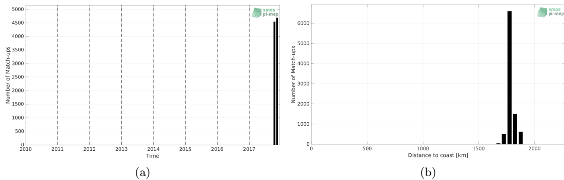
Figure 1: Number of match-ups between Saildrone and SMOS SSS L3 v7 - 9 Days (CATDS-CECOS-LOCEAN) SSS as a function of time (a) and as function of the distance to coast (b) over the SPURS 2 Pi-MEP region and for the full satellite product period.
