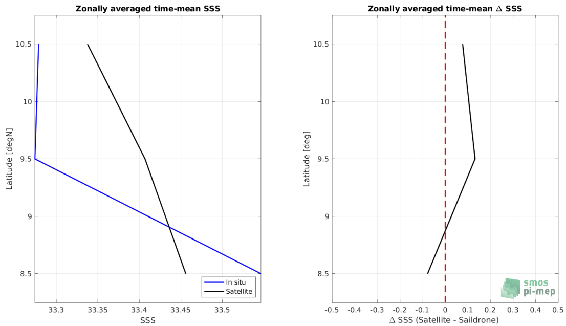
Figure 7: Left panel: Zonal mean SSS from SMOS SSS L3 v7 - 9 Days (CATDS-CECOS-LOCEAN) satellite product (black) and from Sairdrone (blue). Right panel: Zonal mean of \Delta SSS (Satellite - Sairdrone) for all the collected Pi-MEP match-up pairs estimated over the full satellite product period.
