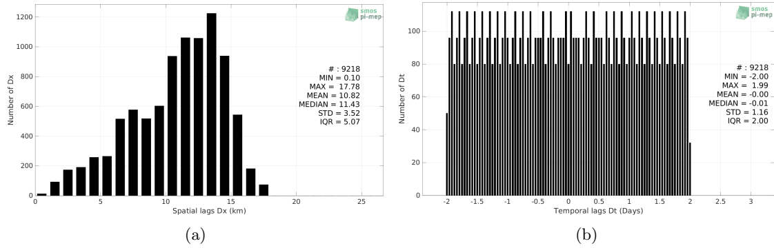
Figure 4: Histograms of the spatial (a) and temporal (b) lags between the location/time of the Saildrone measurement and the date of the corresponding SMOS SSS L3 v7 - 9 Days (CATDS-CECOS-LOCEAN) SSS pixel.
