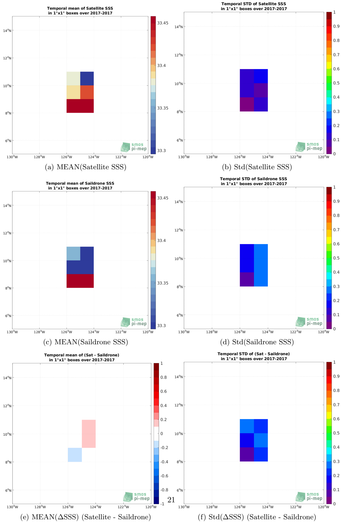
Figure 5: Temporal mean (left) and Std (right) of SSS from SMOS SSS L3 v7 - 9 Days (CATDS-CECOS-LOCEAN) (top), Saildrone (middle), and of \Delta SSS (Satellite - Saildrone). Only match-pairs are used to generate these maps.
