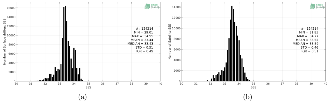
Figure 2: Histograms of SSS from Surface drifters (a) and SMOS SSS L3 v7 - 9 Days (CATDS-CECOS-LOCEAN) (b) considering all match-up pairs per bins of 0.1 over the SPURS 2 Pi-MEP region and for the full satellite product period.
