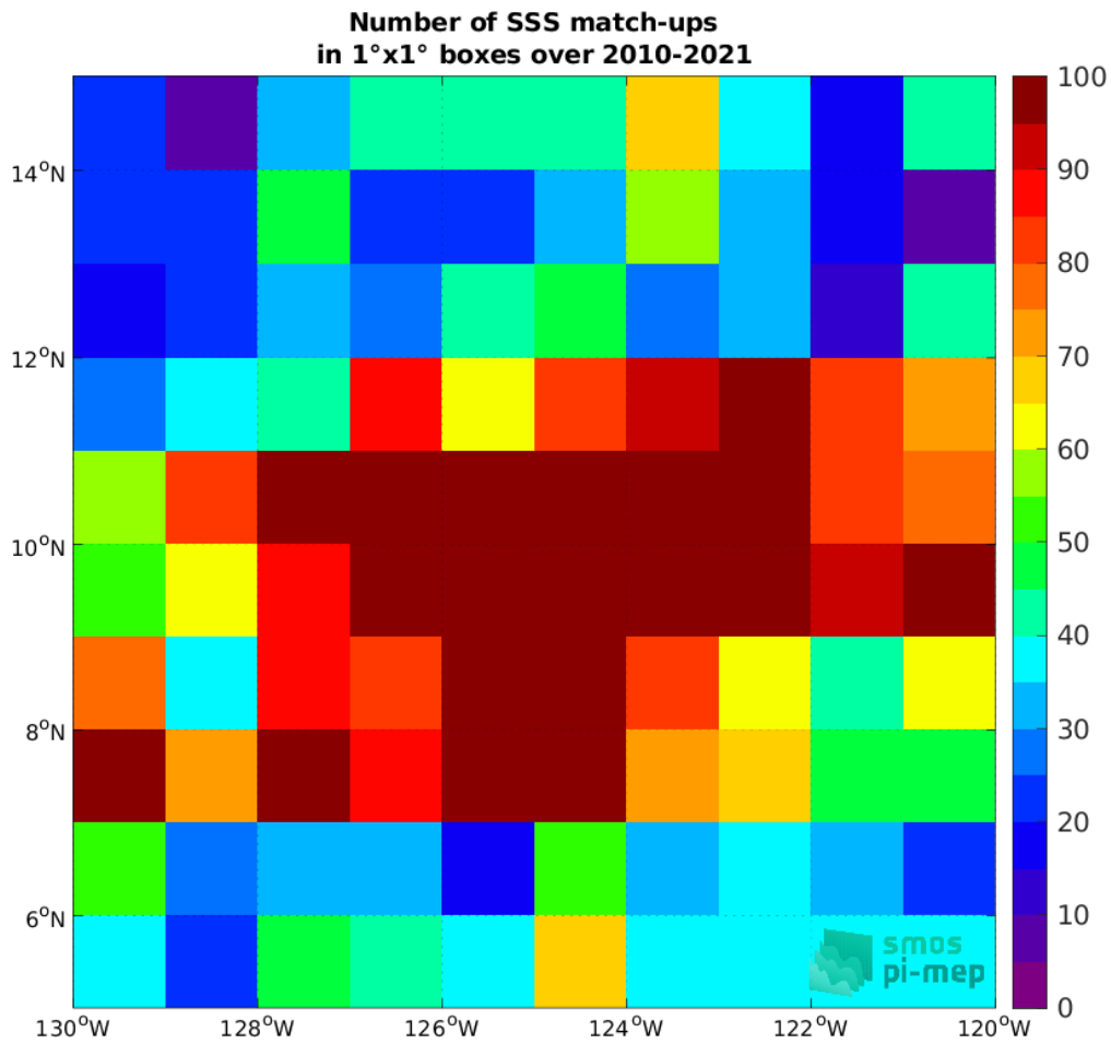
Figure 4: Number of SSS match-ups between Argo SSS and the SMOS SSS L3 v7 - 9 Days (CATDS-CECOS-LOCEAN) SSS product for the SPURS 2 Pi-MEP region over 1°x1° boxes and for the full satellite product period.
