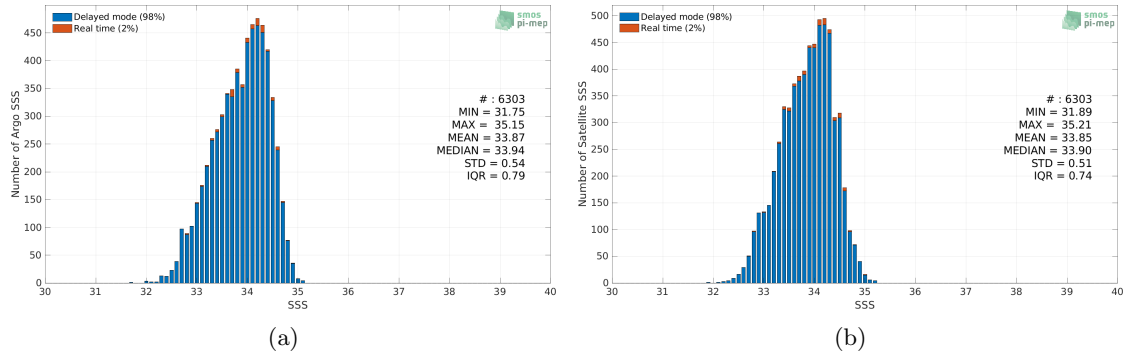
Figure 2: Histograms of SSS from Argo (a) and SMOS SSS L3 v7 - 9 Days (CATDS-CECOS-LOCEAN) (b) considering all match-up pairs per bins of 0.1 over the SPURS 2 Pi-MEP region and for the full satellite product period.
