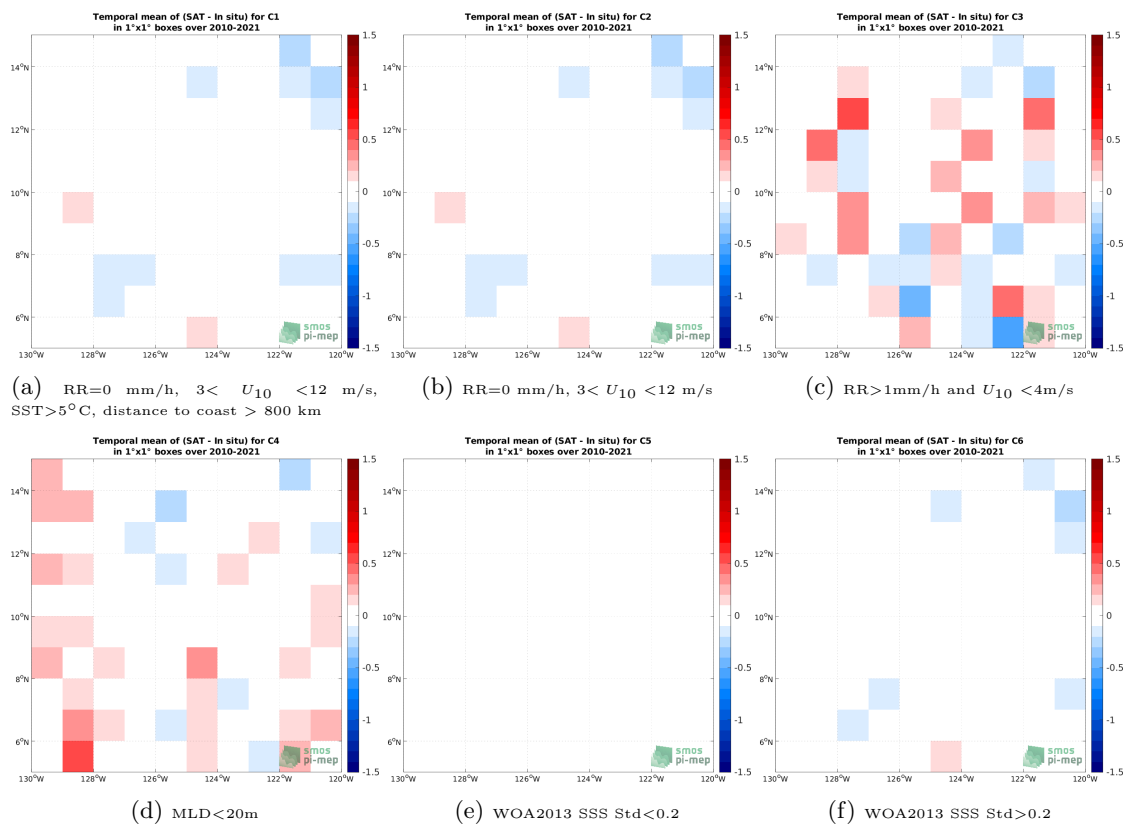
Figure 12: Temporal mean gridded over spatial boxes of size 1^\circ \times 1^\circ of \Delta SSS (SMOS SSS L3 v7 - 9 Days (CATDS-CECOS-LOCEAN) - Argo) for 6 different subdatasets corresponding to:RR=0 mm/h, 3 < U_{10} < 12 m/s, SST >5^\circ C, distance to coast > 800 km (a), RR=0 mm/h, 3 < U_{10} < 12 m/s (b), RR >1 mm/h and U_{10} < 4 m/s (c),MLD <20 m (d),WOA2013 SSS Std <0.2 (e),WOA2013 SSS Std >0.2 (f).
