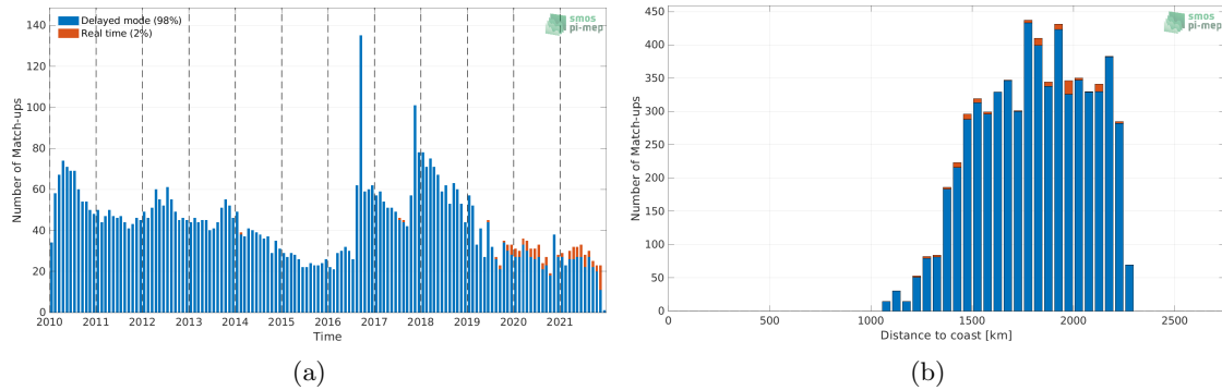
Figure 1: Number of match-ups between Argo and SMOS SSS L3 v7 - 9 Days (CATDS-CECOS-LOCEAN) SSS as a function of time (a) and as function of the distance to coast (b) over the SPURS 2 Pi-MEP region and for the full satellite product period.
