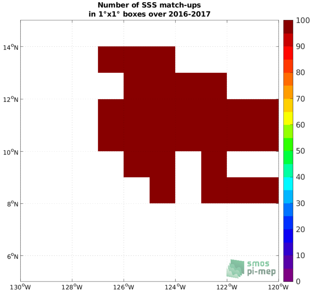
Figure 4: Number of SSS match-ups between Waveglider SSS and the SMOS SSS L3 v7 - 18 Days (CATDS-CECOS-LOCEAN) SSS product for the SPURS 2 Pi-MEP region over 1^\circ \times 1^\circ boxes and for the full satellite product period.
