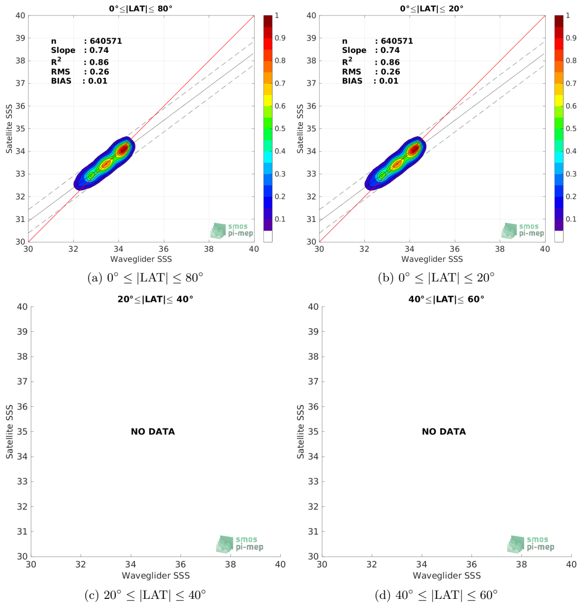
Figure 9: Contour maps of the concentration of SMOS SSS L3 v7 - 18 Days (CATDS-CECOS-LOCEAN) SSS (y-axis) versus Waveglider SSS (x-axis) at match-up pairs for different latitude bands. For each plot, the red line shows x=y . The black thin and dashed lines indicate a linear fit through the data cloud and the \pm 95\% confidence levels, respectively. The number match-up pairs n , the slope and R^2 coefficient of the linear fit, the root mean square (RMS) and the mean bias between satellite and in situ data are indicated for each latitude band in each plots.
