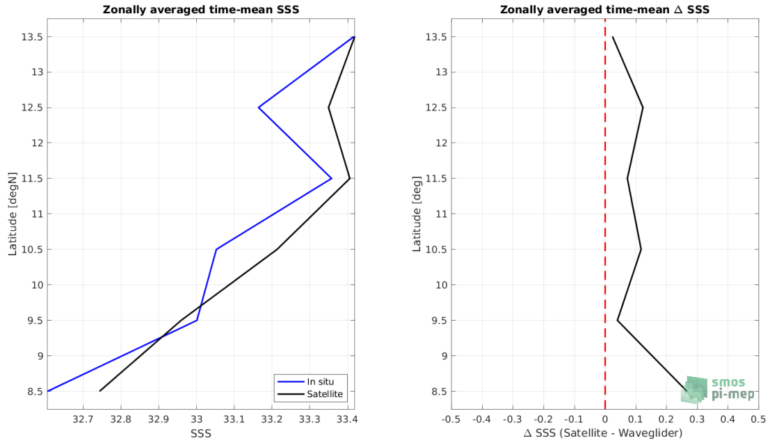
Figure 8: Left panel: Zonal mean SSS from SMOS SSS L3 v7 - 18 Days (CATDS-CECOS-LOCEAN) satellite product (black) and from Waveglider (blue). Right panel: Zonal mean of \Delta SSS (Satellite - Waveglider) for all the collected Pi-MEP match-up pairs estimated over the full satellite product period.
