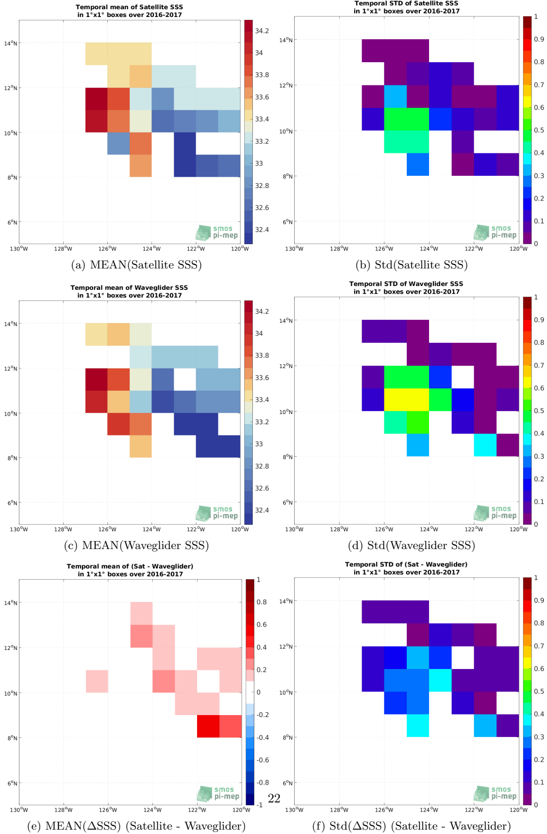
Figure 6: Temporal mean (left) and Std (right) of SSS from SMOS SSS L3 v7 - 18 Days (CATDS-CECOS-LOCEAN) (top), Waveglider (middle), and of \Delta SSS (Satellite - Waveglider). Only match-up pairs are used to generate these maps.
