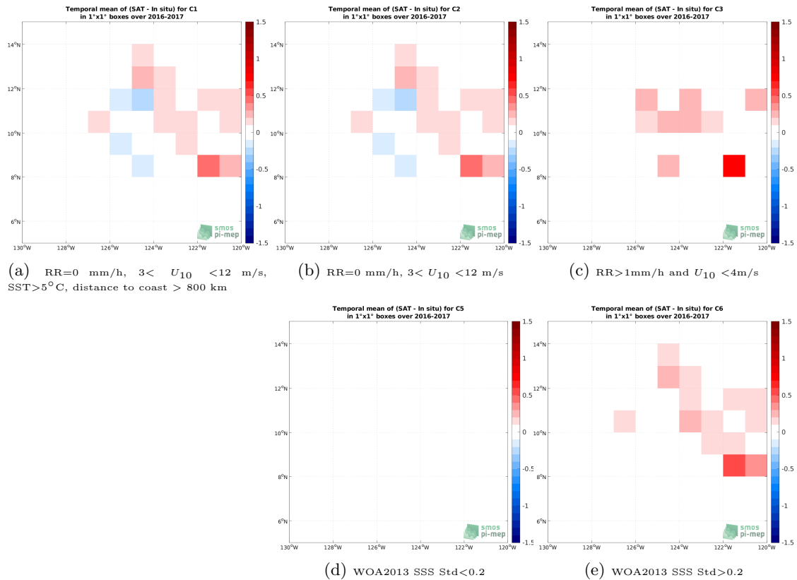
Figure 12: Temporal mean gridded over spatial boxes of size 1^\circ \times 1^\circ of \Delta SSS (SMOS SSS L3 v7 - 18 Days (CATDS-CECOS-LOCEAN) - Waveglider) for 5 different subdatasets corresponding to:RR=0 mm/h, 3 < U_{10} < 12 m/s, SST >5^\circ C, distance to coast > 800 km (a), RR=0 mm/h, 3 < U_{10} < 12 m/s (b), RR >1 mm/h and U_{10} < 4 m/s (c), WOA2013 SSS Std <0.2 (d), WOA2013 SSS Std >0.2 (e).
