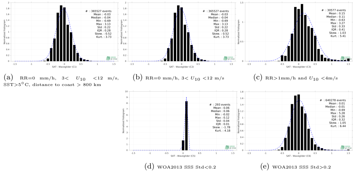
Figure 13: Normalized histogram of \Delta SSS (SMOS SSS L3 v7 - 18 Days (CATDS-CECOS-LOCEAN) - Waveglider) for 5 different subdatasets corresponding to: RR=0 mm/h, 3 < U_{10} < 12 m/s, SST > 5°C, distance to coast > 800 km (a), RR=0 mm/h, 3 < U_{10} < 12 m/s (b), RR > 1mm/h and U_{10} < 4 m/s (c), WOA2013 SSS Std < 0.2 (d), WOA2013 SSS Std > 0.2 (e).
