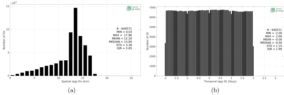
Figure 5: Histograms of the spatial (a) and temporal (b) lags between the location/time of the Waveglider measurement and the date of the corresponding SMOS SSS L3 v7 - 18 Days (CATDS-CECOS-LOCEAN) SSS pixel.
