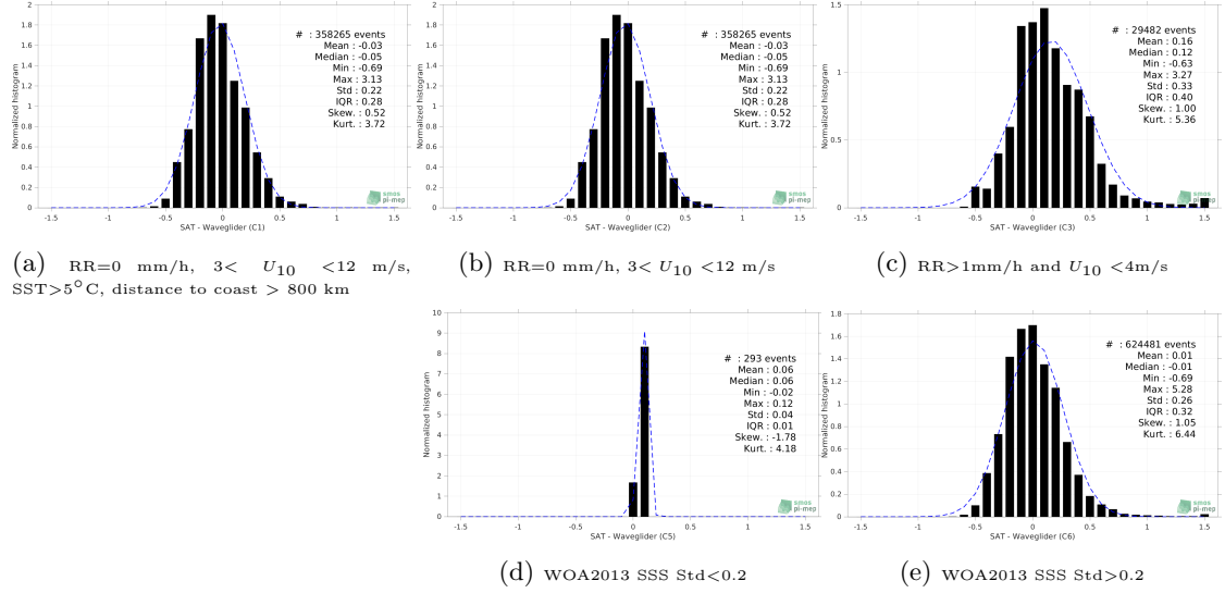
Figure 12: Normalized histogram of \Delta SSS (SMOS SSS L3 v7 - 18 Days (CATDS-CECOS-LOCEAN) - Waveglider) for 5 different subdatasets corresponding to: RR=0 mm/h, 3 < U_{10} < 12 m/s, SST > 5°C, distance to coast > 800 km (a), RR=0 mm/h, 3 < U_{10} < 12 m/s (b), RR > 1mm/h and U_{10} < 4 m/s (c), WOA2013 SSS Std < 0.2 (d), WOA2013 SSS Std > 0.2 (e).
