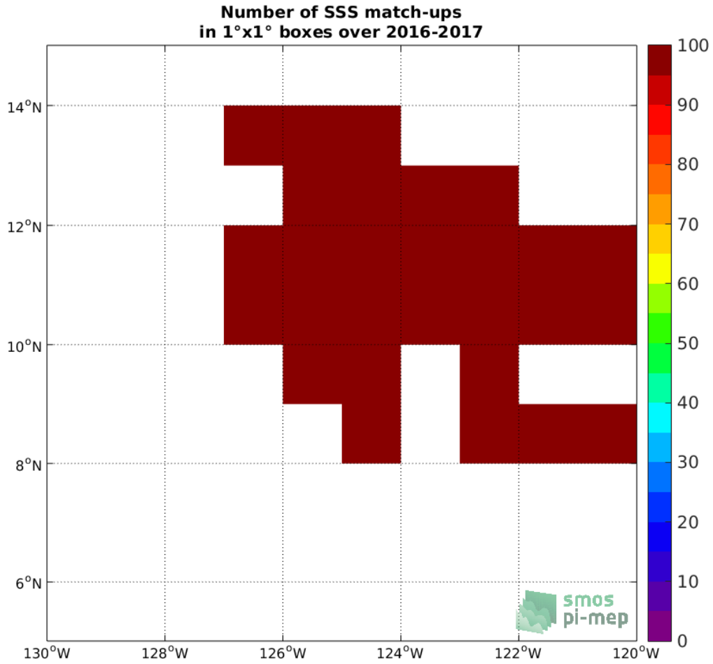
Figure 3: Number of SSS match-ups between Waveglider SSS and the SMOS SSS L3 v7 - 18 Days (CATDS-CECOS-LOCEAN) SSS product for the SPURS 2 Pi-MEP region over 1°x1° boxes and for the full satellite product period.
