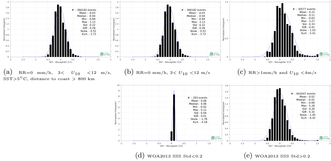
Figure 12: Normalized histogram of \Delta SSS (SMOS SSS L3 v7 - 18 Days (CATDS-CECOS-LOCEAN) - Waveglider) for 5 different subdatasets corresponding to: RR=0 mm/h, 3 < U_{10} < 12 m/s, SST > 5°C, distance to coast > 800 km (a), RR=0 mm/h, 3 < U_{10} < 12 m/s (b), RR > 1mm/h and U_{10} < 4 m/s (c), WOA2013 SSS Std < 0.2 (d), WOA2013 SSS Std > 0.2 (e).
