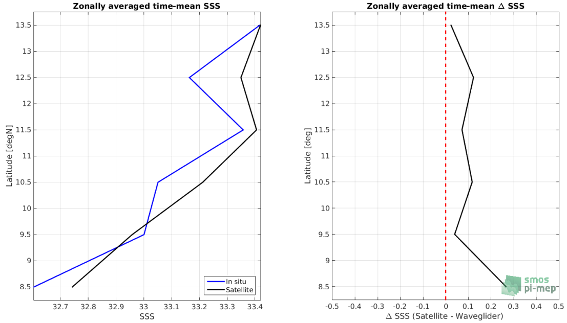
Figure 7: Left panel: Zonal mean SSS from SMOS SSS L3 v7 - 18 Days (CATDS-CECOS-LOCEAN) satellite product (black) and from Waveglider (blue). Right panel: Zonal mean of \Delta SSS (Satellite - Waveglider) for all the collected Pi-MEP match-up pairs estimated over the full satellite product period.
