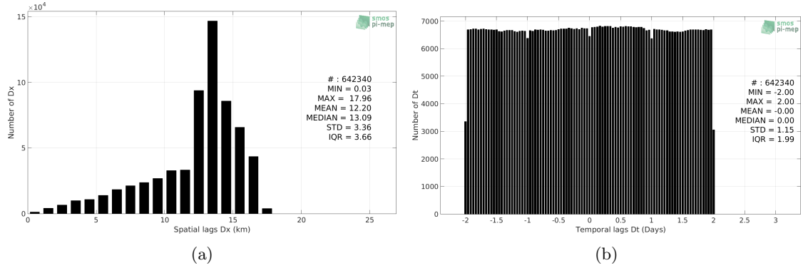
Figure 4: Histograms of the spatial (a) and temporal (b) lags between the location/time of the Waveglider measurement and the date of the corresponding SMOS SSS L3 v7 - 18 Days (CATDS-CECOS-LOCEAN) SSS pixel.
