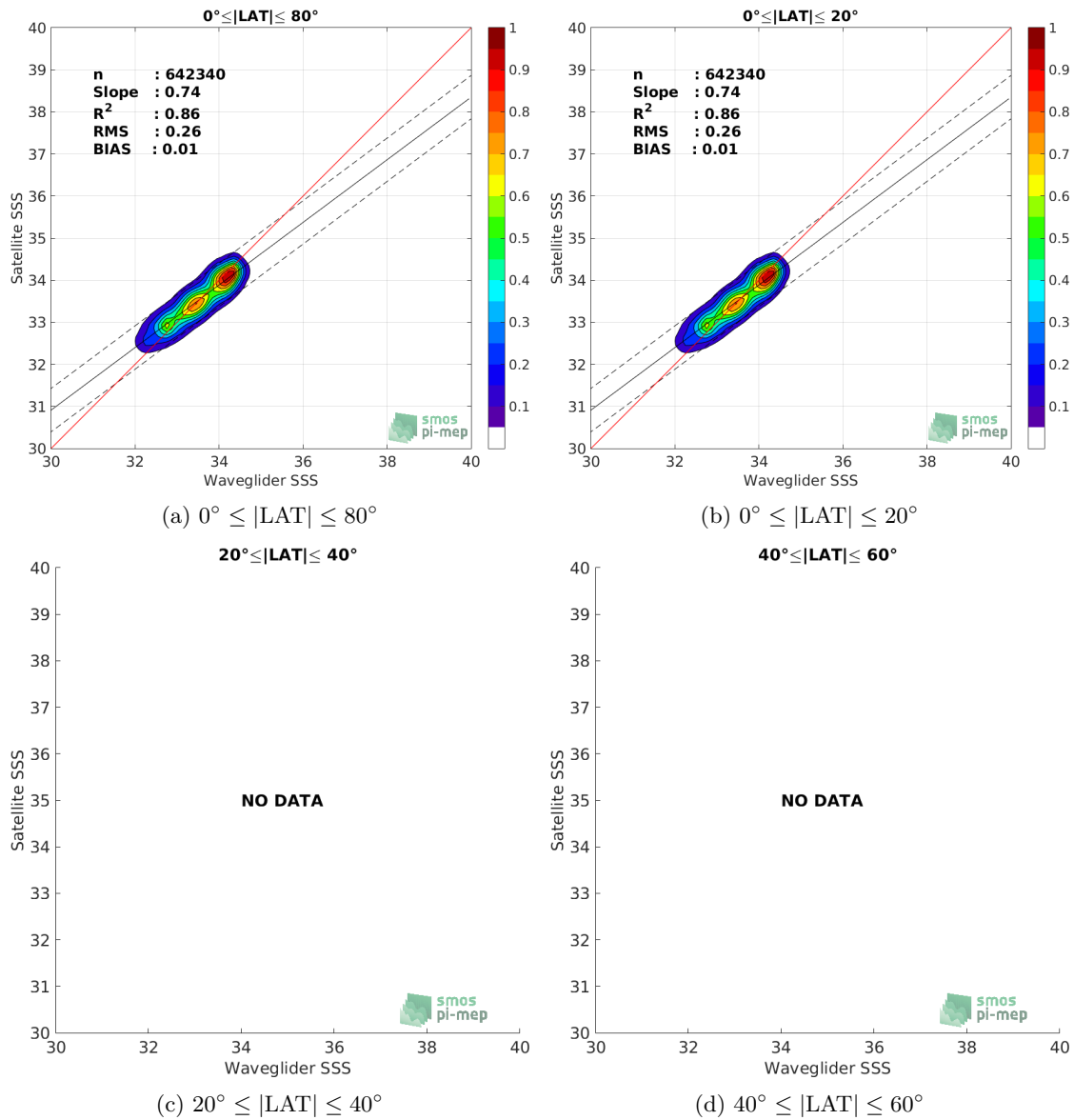
Figure 8: Contour maps of the concentration of SMOS SSS L3 v7 - 18 Days (CATDS-CECOS-LOCEAN) SSS (y-axis) versus Waveglider SSS (x-axis) at match-up pairs for different latitude bands. For each plot, the red line shows x=y . The black thin and dashed lines indicate a linear fit through the data cloud and the \pm 95\% confidence levels, respectively. The number match-up pairs n , the slope and R^2 coefficient of the linear fit, the root mean square (RMS) and the mean bias between satellite and in situ data are indicated for each latitude band in each plots.
