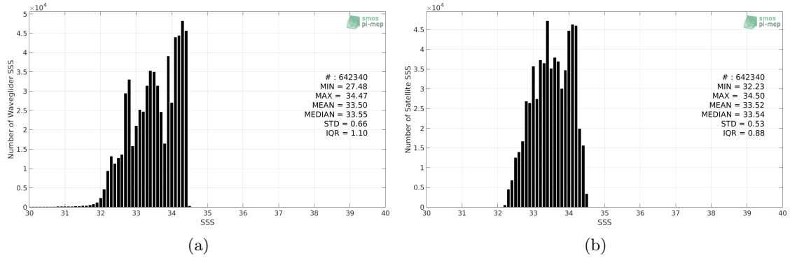
Figure 2: Histograms of SSS from Waveglider (a) and SMOS SSS L3 v7 - 18 Days (CATDS-CECOS-LOCEAN) (b) considering all match-up pairs per bins of 0.1 over the SPURS 2 Pi-MEP region and for the full satellite product period.
