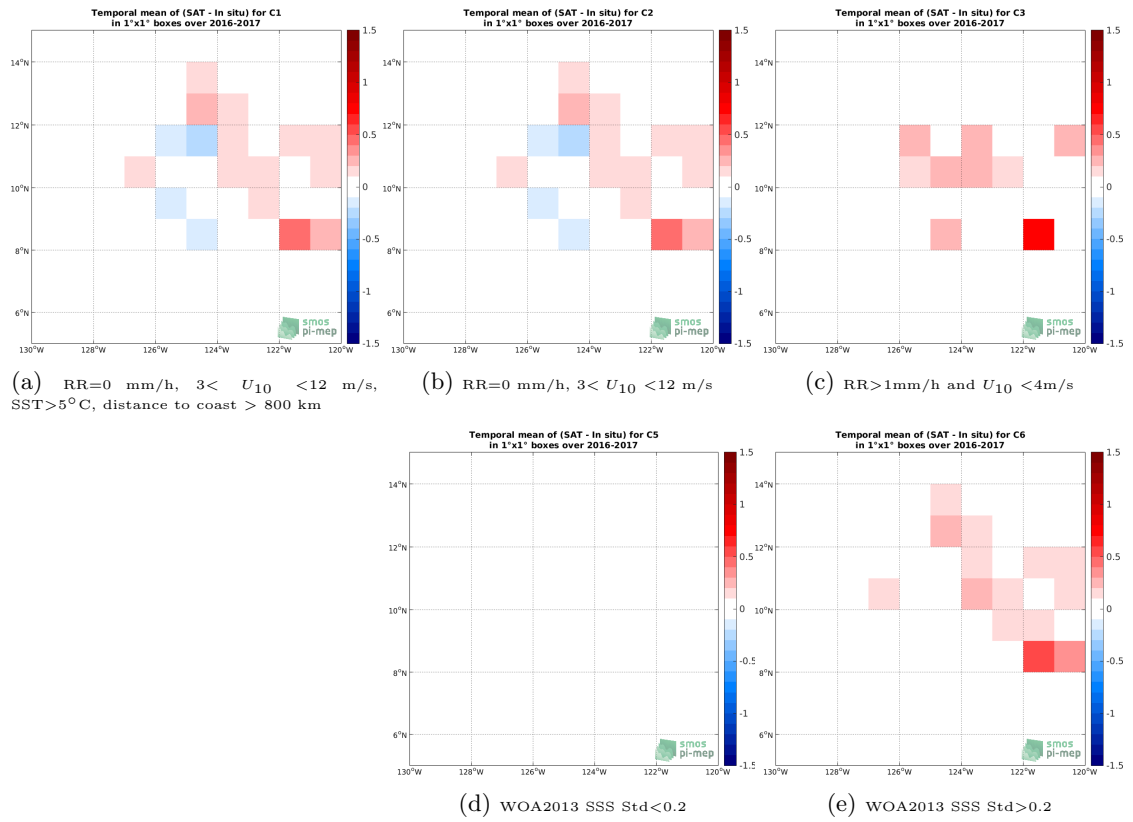
Figure 11: Temporal mean gridded over spatial boxes of size 1^\circ \times 1^\circ of \Delta SSS (SMOS SSS L3 v7 - 18 Days (CATDS-CECOS-LOCEAN) - Waveglider) for 5 different subdatasets corresponding to:RR=0 mm/h, 3 < U_{10} < 12 m/s, SST >5^\circ C, distance to coast > 800 km (a), RR=0 mm/h, 3 < U_{10} < 12 m/s (b), RR >1 mm/h and U_{10} < 4 m/s (c), WOA2013 SSS Std <0.2 (d), WOA2013 SSS Std >0.2 (e).
