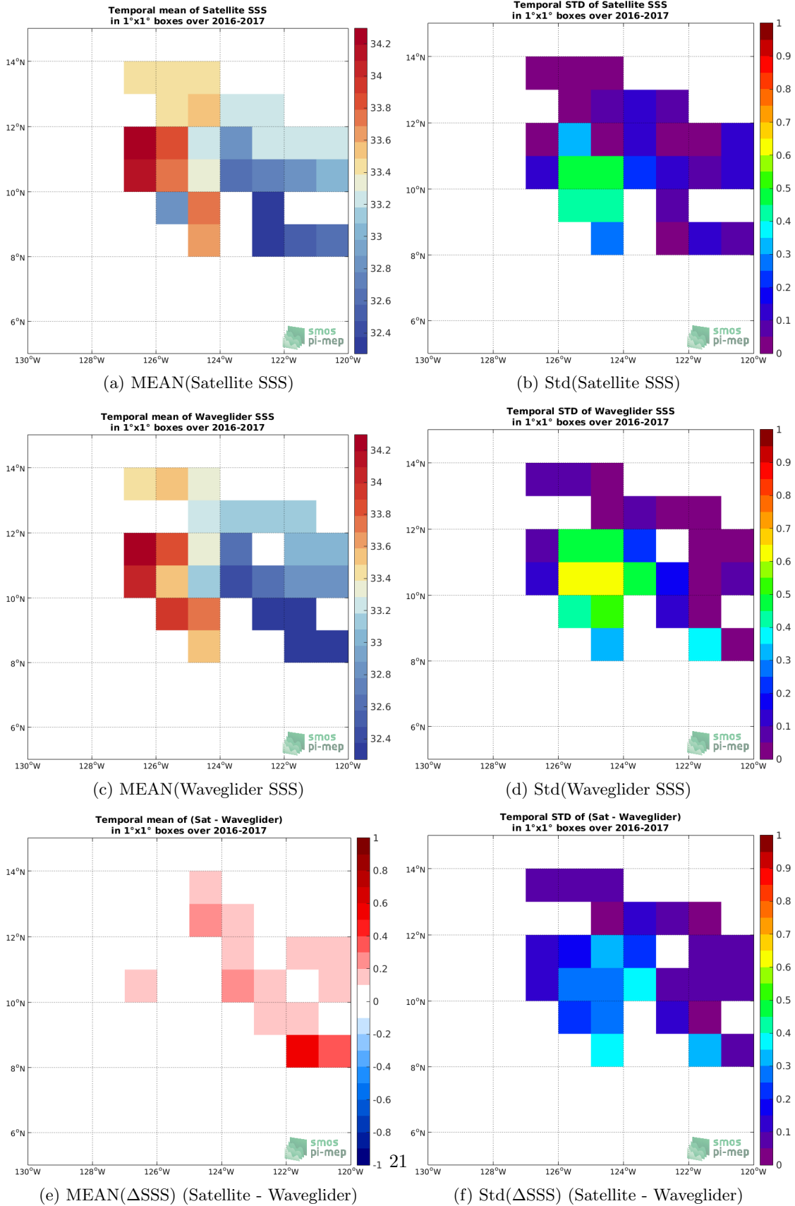
Figure 5: Temporal mean (left) and Std (right) of SSS from SMOS SSS L3 v7 - 18 Days (CATDS-CECOS-LOCEAN) (top), Waveglider (middle), and of \Delta SSS (Satellite - Waveglider). Only match-up pairs are used to generate these maps.
