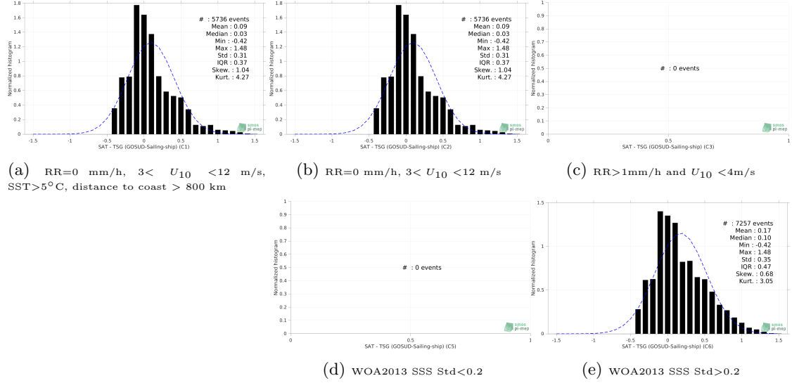
Figure 13: Normalized histogram of \Delta\text{SSS} (SMOS SSS L3 v7 - 18 Days (CATDS-CECOS-LOCEAN) - TSG (GOSUD-Sailing-ship)) for 5 different subdatasets corresponding to: RR=0 mm/h, 3 < U_{10} < 12 m/s, SST > 5^{\circ}\text{C} , distance to coast > 800 km (a), RR=0 mm/h, 3 < U_{10} < 12 m/s (b), RR > 1\text{mm/h} and U_{10} < 4\text{m/s} (c), WOA2013 SSS Std < 0.2 (d), WOA2013 SSS Std > 0.2 (e).
