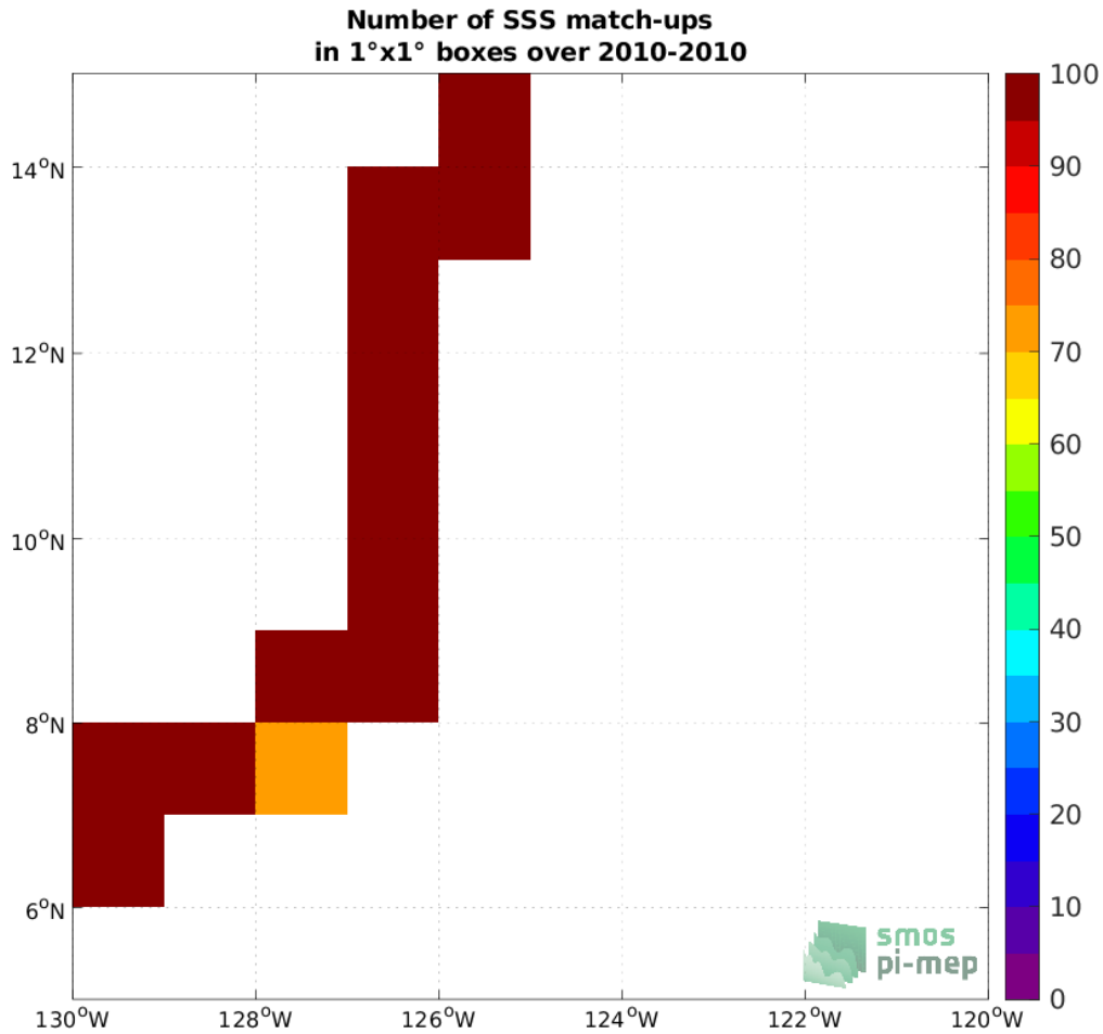
Figure 4: Number of SSS match-ups between TSG (GOSUD-Sailing-ship) SSS and the SMOS SSS L3 v7 - 18 Days (CATDS-CECOS-LOCEAN) SSS product for the SPURS 2 Pi-MEP region over 1^\circ \times 1^\circ boxes and for the full satellite product period.
