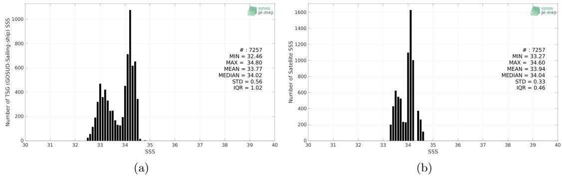
Figure 2: Histograms of SSS from TSG (GOSUD-Sailing-ship) (a) and SMOS SSS L3 v7 - 18 Days (CATDS-CECOS-LOCEAN) (b) considering all match-up pairs per bins of 0.1 over the SPURS 2 Pi-MEP region and for the full satellite product period.
