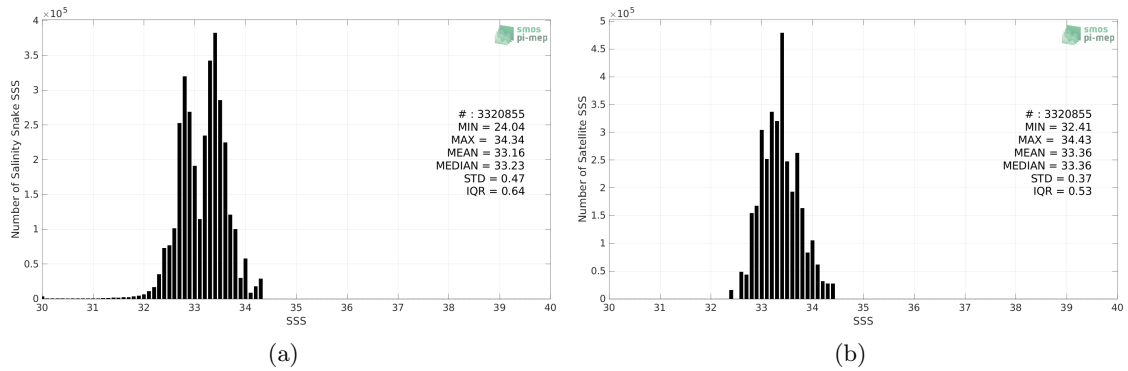
Figure 2: Histograms of SSS from Salinity Snake (a) and SMOS SSS L3 v7 - 18 Days (CATDS-CECOS-LOCEAN) (b) considering all match-up pairs per bins of 0.1 over the SPURS 2 Pi-MEP region and for the full satellite product period.
