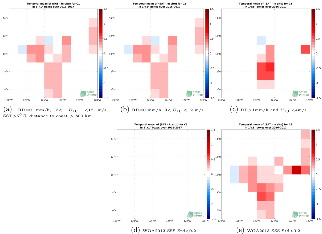
Figure 12: Temporal mean gridded over spatial boxes of size 1^\circ \times 1^\circ of \Delta SSS (SMOS SSS L3 v7 - 18 Days (CATDS-CECOS-LOCEAN) - Salinity Snake) for 5 different subdatasets corresponding to:RR=0 mm/h, 3 < U_{10} < 12 m/s, SST >5^\circ C, distance to coast > 800 km (a), RR=0 mm/h, 3 < U_{10} < 12 m/s (b), RR >1 mm/h and U_{10} < 4 m/s (c), WOA2013 SSS Std <0.2 (d), WOA2013 SSS Std >0.2 (e).
