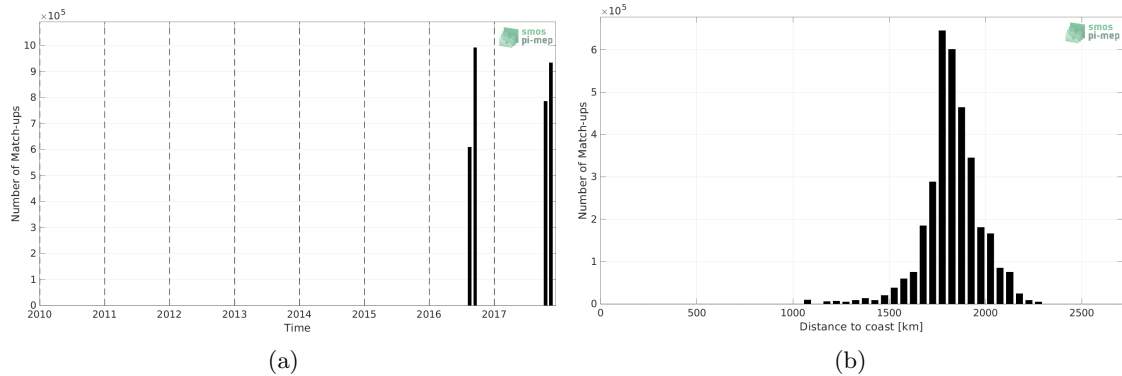
Figure 1: Number of match-ups between Salinity Snake and SMOS SSS L3 v7 - 18 Days (CATDS-CECOS-LOCEAN) SSS as a function of time (a) and as function of the distance to coast (b) over the SPURS 2 Pi-MEP region and for the full satellite product period.
