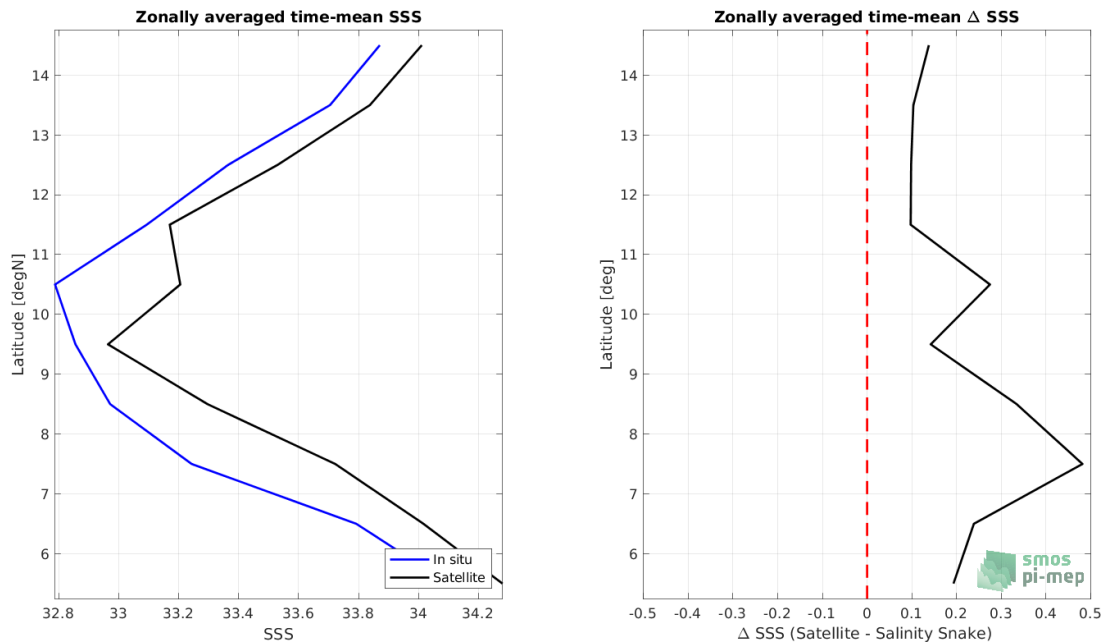
Figure 8: Left panel: Zonal mean SSS from SMOS SSS L3 v7 - 18 Days (CATDS-CECOS-LOCEAN) satellite product (black) and from Salinity Snake (blue). Right panel: Zonal mean of \Delta SSS (Satellite - Salinity Snake) for all the collected Pi-MEP match-up pairs estimated over the full satellite product period.
