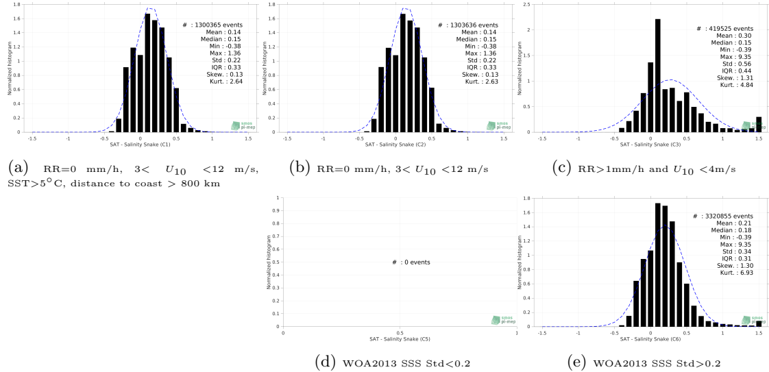
Figure 13: Normalized histogram of \Delta SSS (SMOS SSS L3 v7 - 18 Days (CATDS-CECOS-LOCEAN) - Salinity Snake) for 5 different subdatasets corresponding to: RR=0 mm/h, 3 < U_{10} < 12 m/s, SST > 5°C, distance to coast > 800 km (a), RR=0 mm/h, 3 < U_{10} < 12 m/s (b), RR > 1mm/h and U_{10} < 4 m/s (c), WOA2013 SSS Std < 0.2 (d), WOA2013 SSS Std > 0.2 (e).
