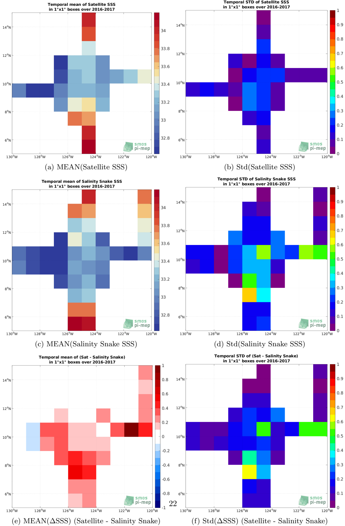
Figure 6: Temporal mean (left) and Std (right) of SSS from SMOS SSS L3 v7 - 18 Days (CATDS-CECOS-LOCEAN) (top), Salinity Snake (middle), and of \Delta SSS (Satellite - Salinity Snake). Only match-up pairs are used to generate these maps.
