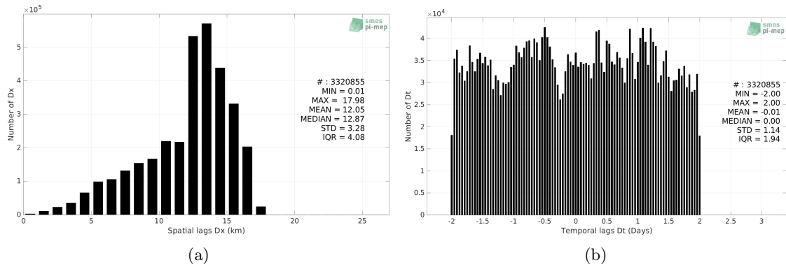
Figure 5: Histograms of the spatial (a) and temporal (b) lags between the location/time of the Salinity Snake measurement and the date of the corresponding SMOS SSS L3 v7 - 18 Days (CATDS-CECOS-LOCEAN) SSS pixel.
