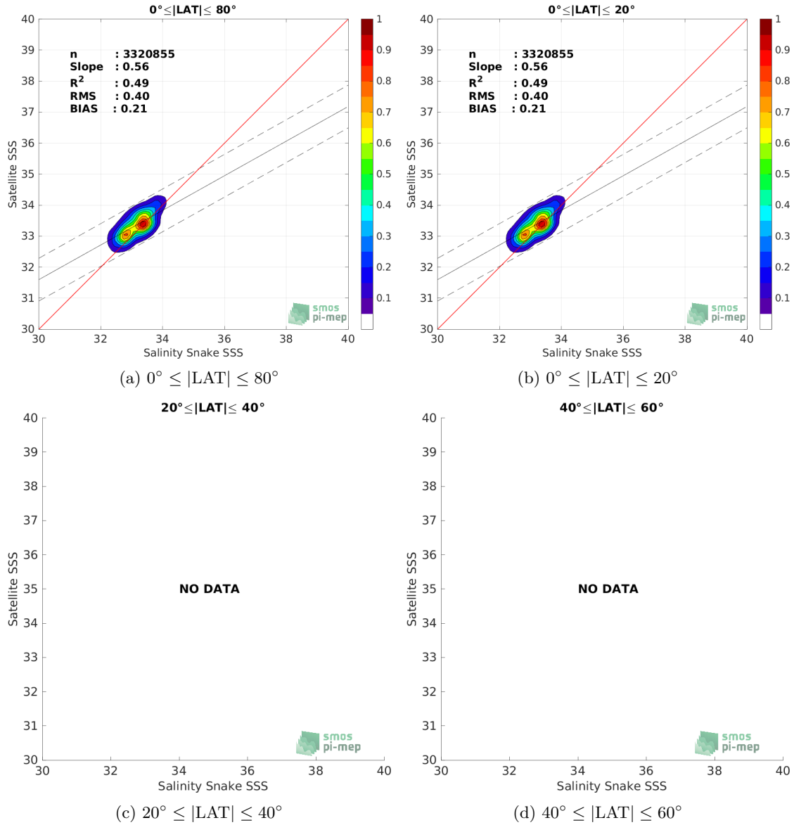
Figure 9: Contour maps of the concentration of SMOS SSS L3 v7 - 18 Days (CATDS-CECOS-LOCEAN) SSS (y-axis) versus Salinity Snake SSS (x-axis) at match-up pairs for different latitude bands. For each plot, the red line shows x=y . The black thin and dashed lines indicate a linear fit through the data cloud and the \pm 95\% confidence levels, respectively. The number match-up pairs n , the slope and R^2 coefficient of the linear fit, the root mean square (RMS) and the mean bias between satellite and in situ data are indicated for each latitude band in each plots.
