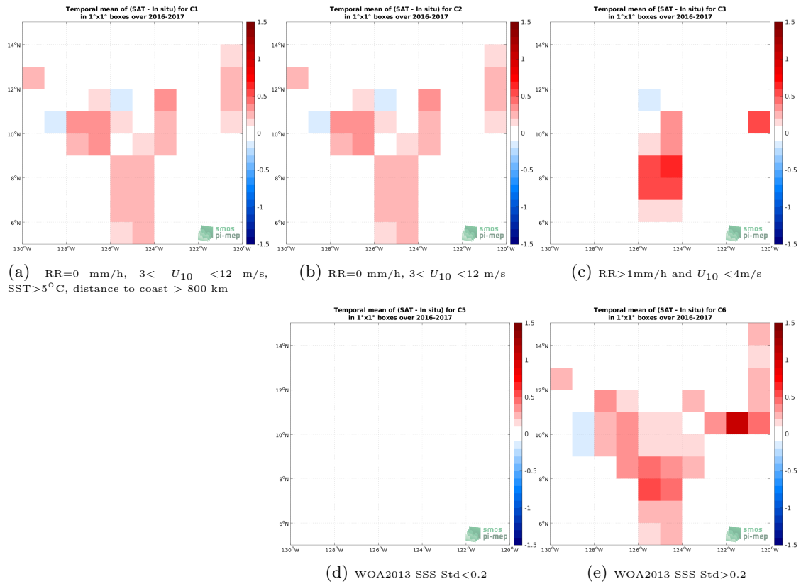
Figure 11: Temporal mean gridded over spatial boxes of size 1^\circ \times 1^\circ of \Delta SSS (SMOS SSS L3 v7 - 18 Days (CATDS-CECOS-LOCEAN) - Salinity Snake) for 5 different subdatasets corresponding to:RR=0 mm/h, 3 < U_{10} < 12 m/s, SST >5^\circ\text{C} , distance to coast > 800 km (a), RR=0 mm/h, 3 < U_{10} < 12 m/s (b), RR >1 mm/h and U_{10} < 4 m/s (c), WOA2013 SSS Std <0.2 (d), WOA2013 SSS Std >0.2 (e).
