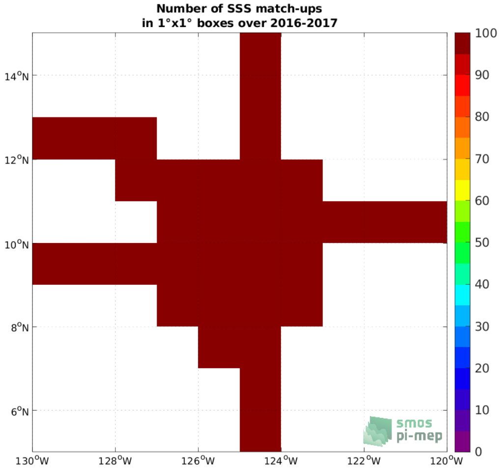
Figure 3: Number of SSS match-ups between Salinity Snake SSS and the SMOS SSS L3 v7 - 18 Days (CATDS-CECOS-LOCEAN) SSS product for the SPURS 2 Pi-MEP region over 1°x1° boxes and for the full satellite product period.
