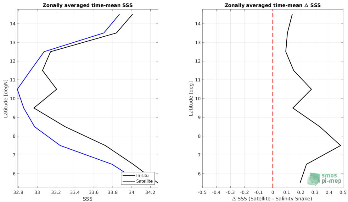
Figure 7: Left panel: Zonal mean SSS from SMOS SSS L3 v7 - 18 Days (CATDS-CECOS-LOCEAN) satellite product (black) and from Salinity Snake (blue). Right panel: Zonal mean of \Delta SSS (Satellite - Salinity Snake) for all the collected Pi-MEP match-up pairs estimated over the full satellite product period.
