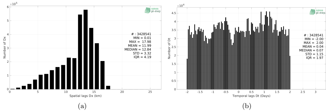
Figure 4: Histograms of the spatial (a) and temporal (b) lags between the location/time of the Salinity Snake measurement and the date of the corresponding SMOS SSS L3 v7 - 18 Days (CATDS-CECOS-LOCEAN) SSS pixel.
