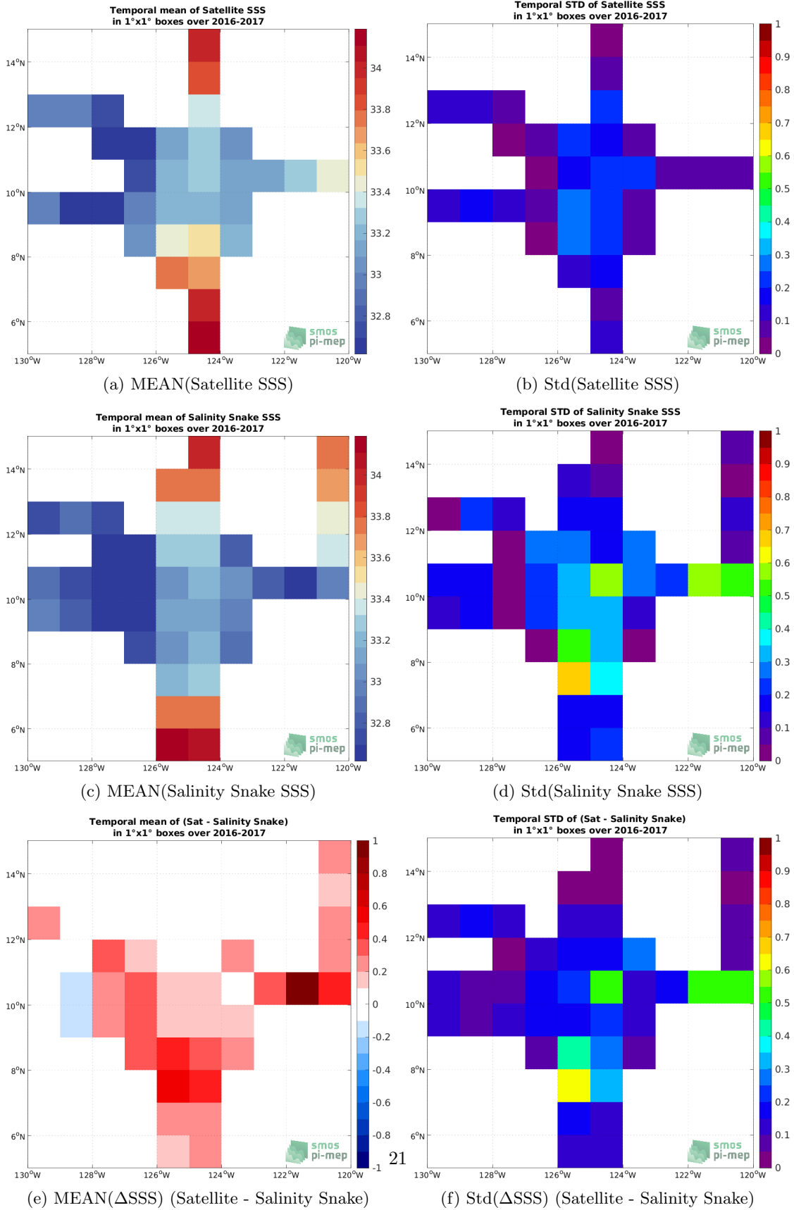
Figure 5: Temporal mean (left) and Std (right) of SSS from SMOS SSS L3 v7 - 18 Days (CATDS-CECOS-LOCEAN) (top), Salinity Snake (middle), and of \Delta SSS (Satellite - Salinity Snake). Only match-up pairs are used to generate these maps.
