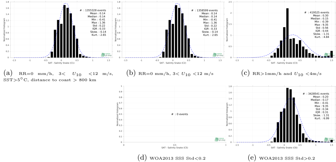
Figure 12: Normalized histogram of \Delta SSS (SMOS SSS L3 v7 - 18 Days (CATDS-CECOS-LOCEAN) - Salinity Snake) for 5 different subdatasets corresponding to: RR=0 mm/h, 3 < U_{10} < 12 m/s, SST>5°C, distance to coast > 800 km (a), RR=0 mm/h, 3 < U_{10} < 12 m/s (b), RR>1mm/h and U_{10} < 4 m/s (c), WOA2013 SSS Std<0.2 (d), WOA2013 SSS Std>0.2 (e).
