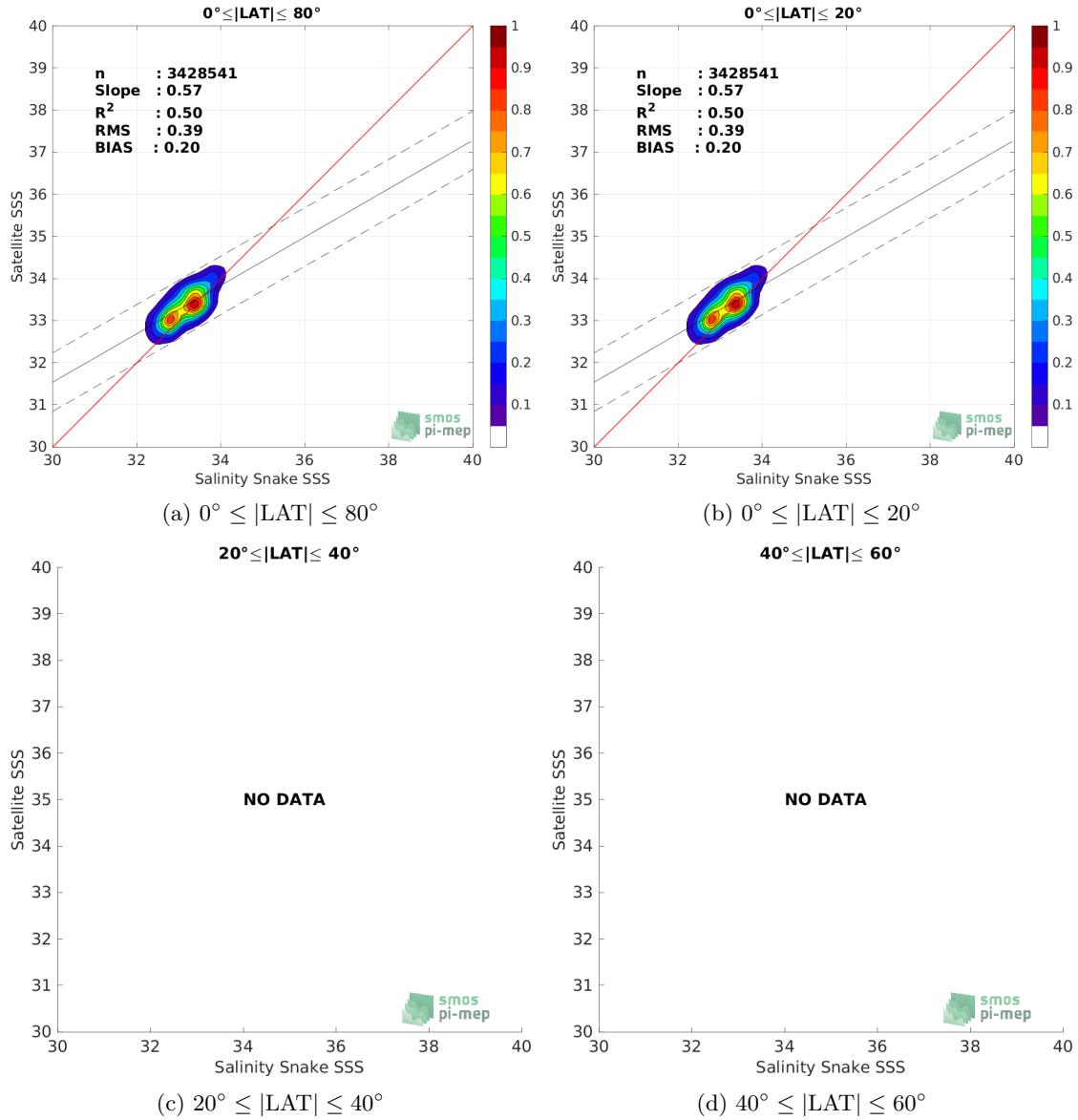
Figure 8: Contour maps of the concentration of SMOS SSS L3 v7 - 18 Days (CATDS-CECOS-LOCEAN) SSS (y-axis) versus Salinity Snake SSS (x-axis) at match-up pairs for different latitude bands. For each plot, the red line shows x=y . The black thin and dashed lines indicate a linear fit through the data cloud and the \pm 95\% confidence levels, respectively. The number match-up pairs n , the slope and R^2 coefficient of the linear fit, the root mean square (RMS) and the mean bias between satellite and in situ data are indicated for each latitude band in each plots.
