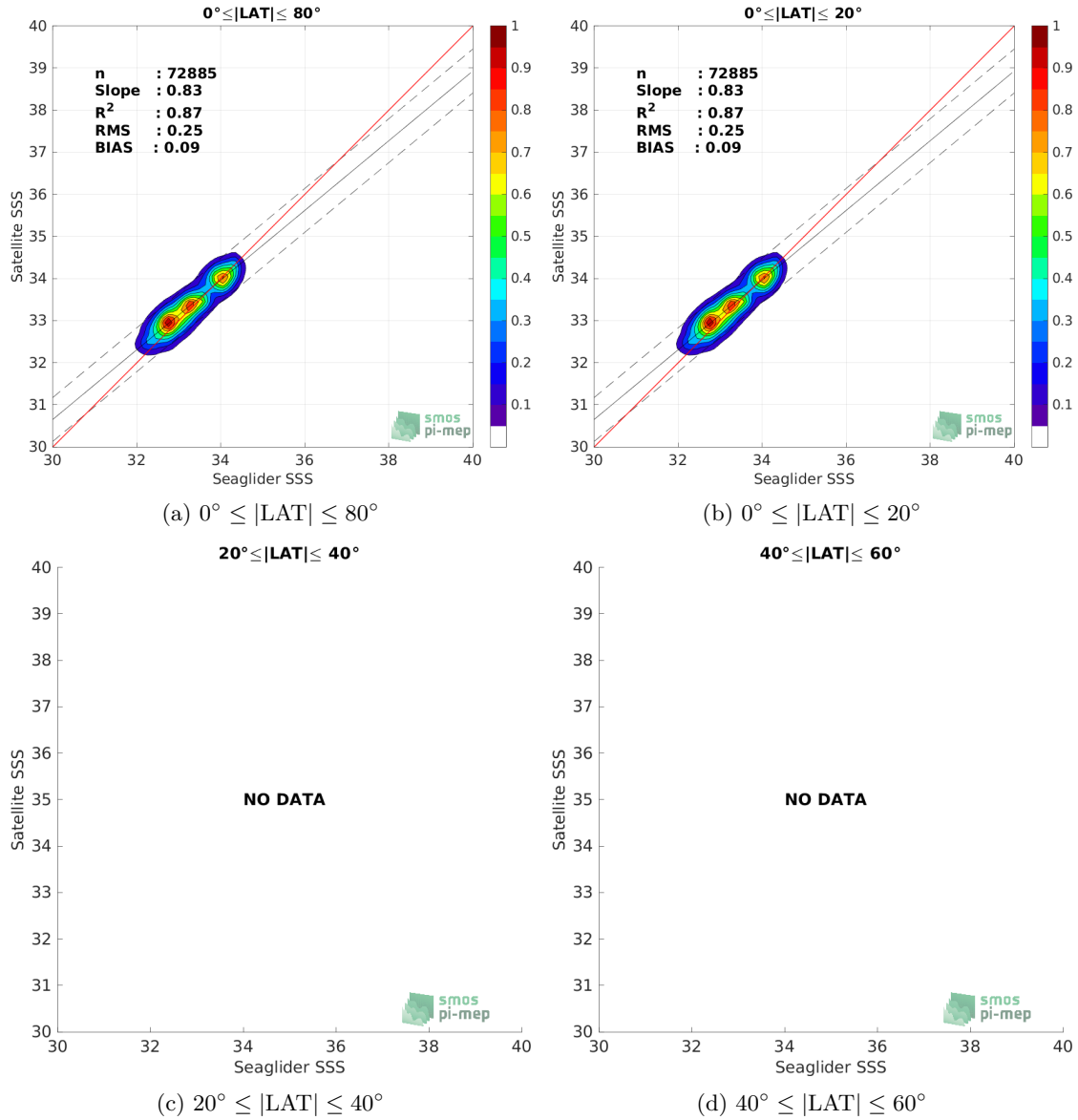
Figure 9: Contour maps of the concentration of SMOS SSS L3 v7 - 18 Days (CATDS-CECOS-LOCEAN) SSS (y-axis) versus Seaglider SSS (x-axis) at match-up pairs for different latitude bands. For each plot, the red line shows x=y . The black thin and dashed lines indicate a linear fit through the data cloud and the \pm 95\% confidence levels, respectively. The number match-up pairs n , the slope and R^2 coefficient of the linear fit, the root mean square (RMS) and the mean bias between satellite and in situ data are indicated for each latitude band in each plots.
