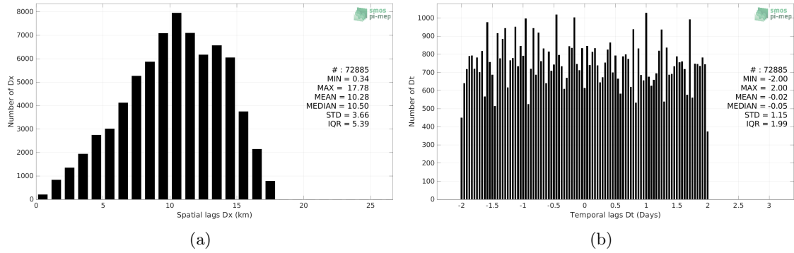
Figure 5: Histograms of the spatial (a) and temporal (b) lags between the location/time of the Seaglider measurement and the date of the corresponding SMOS SSS L3 v7 - 18 Days (CATDS-CECOS-LOCEAN) SSS pixel.
