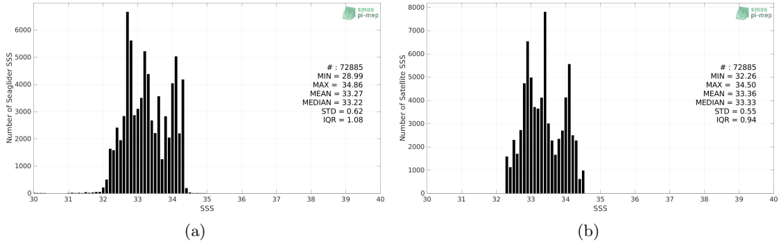
Figure 2: Histograms of SSS from Seaglider (a) and SMOS SSS L3 v7 - 18 Days (CATDS-CECOS-LOCEAN) (b) considering all match-up pairs per bins of 0.1 over the SPURS 2 Pi-MEP region and for the full satellite product period.
