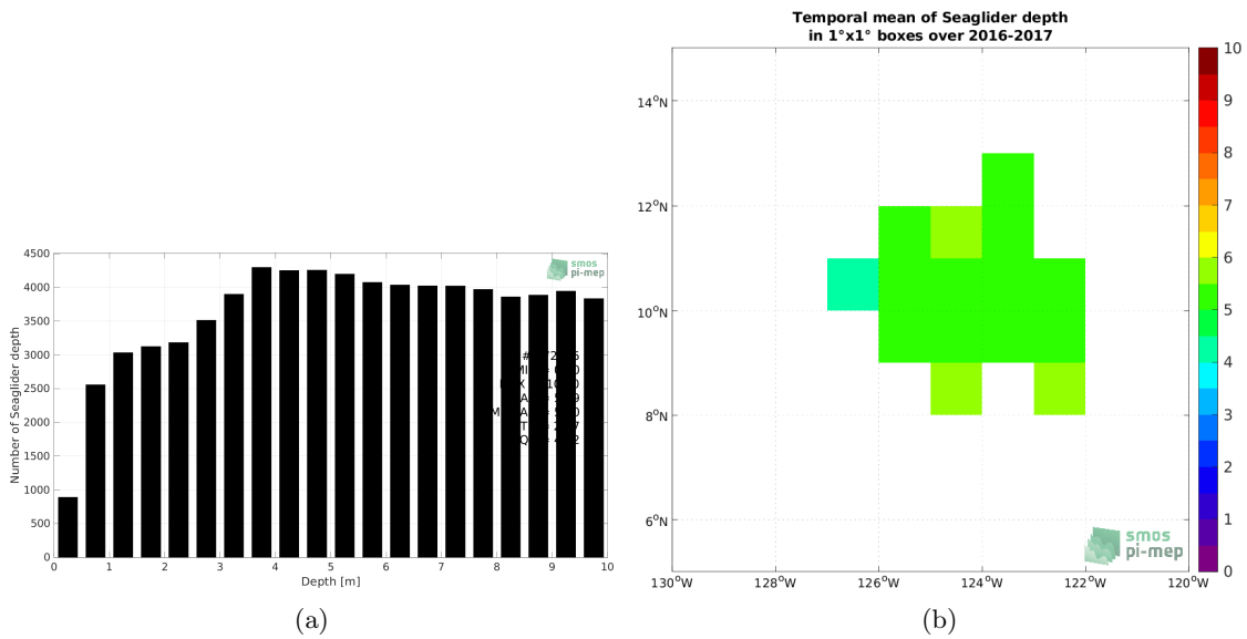
Figure 3: Histograms of the depth of the upper level SSS measurements from Seaglider in the Match-up DataBase for the SPURS 2 Pi-MEP region (a) and temporal mean spatial distribution of pressure of the in situ SSS data over 1^\circ \times 1^\circ boxes and for the full satellite product period (b).
