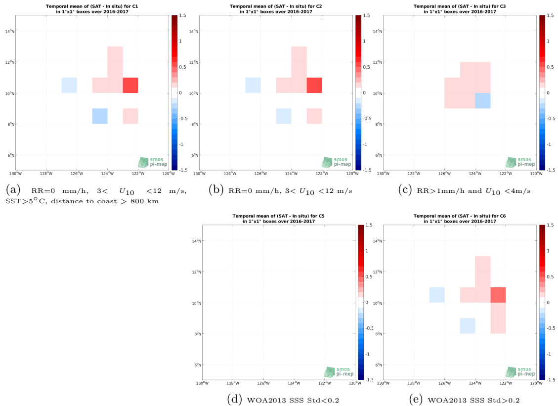
Figure 12: Temporal mean gridded over spatial boxes of size 1^\circ \times 1^\circ of \Delta SSS (SMOS SSS L3 v7 - 18 Days (CATDS-CECOS-LOCEAN) - Seaglider) for 5 different subdatasets corresponding to:RR=0 mm/h, 3 < U_{10} < 12 m/s, SST >5^\circ C, distance to coast > 800 km (a), RR=0 mm/h, 3 < U_{10} < 12 m/s (b), RR >1 mm/h and U_{10} < 4 m/s (c), WOA2013 SSS Std <0.2 (d), WOA2013 SSS Std >0.2 (e).
