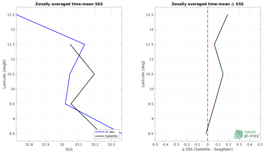
Figure 8: Left panel: Zonal mean SSS from SMOS SSS L3 v7 - 18 Days (CATDS-CECOS-LOCEAN) satellite product (black) and from Seaglider (blue). Right panel: Zonal mean of \Delta SSS (Satellite - Seaglider) for all the collected Pi-MEP match-up pairs estimated over the full satellite product period.
