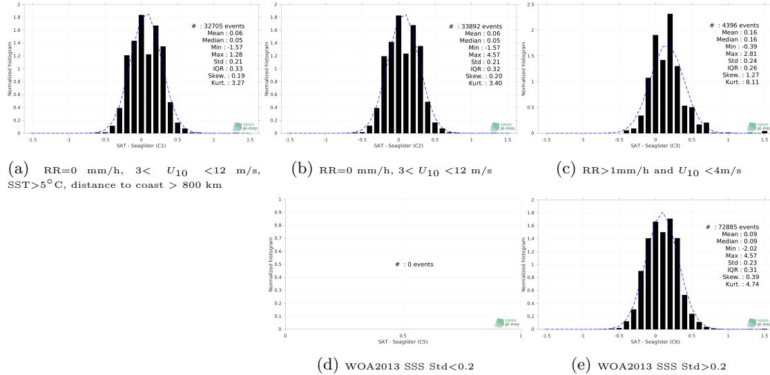
Figure 13: Normalized histogram of \Delta SSS (SMOS SSS L3 v7 - 18 Days (CATDS-CECOS-LOCEAN) - Seaglider) for 5 different subdatasets corresponding to: RR=0 mm/h, 3 < U_{10} < 12 m/s, SST>5°C, distance to coast > 800 km (a), RR=0 mm/h, 3 < U_{10} < 12 m/s (b), RR>1mm/h and U_{10} < 4 m/s (c), WOA2013 SSS Std<0.2 (d), WOA2013 SSS Std>0.2 (e).
