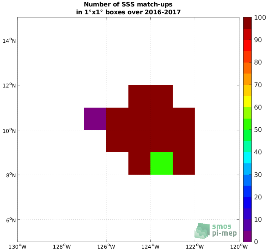
Figure 4: Number of SSS match-ups between Seaglider SSS and the SMOS SSS L3 v7 - 18 Days (CATDS-CECOS-LOCEAN) SSS product for the SPURS 2 Pi-MEP region over 1^\circ \times 1^\circ boxes and for the full satellite product period.
