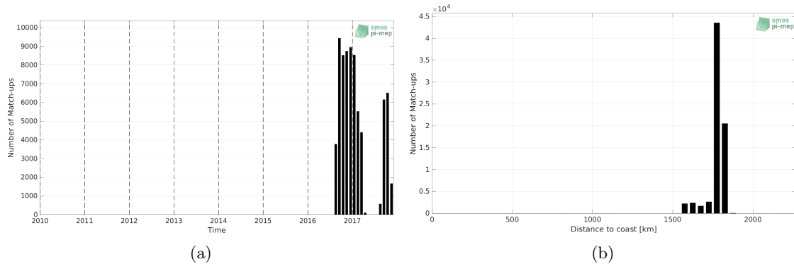
Figure 1: Number of match-ups between Seaglider and SMOS SSS L3 v7 - 18 Days (CATDS-CECOS-LOCEAN) SSS as a function of time (a) and as function of the distance to coast (b) over the SPURS 2 Pi-MEP region and for the full satellite product period.
