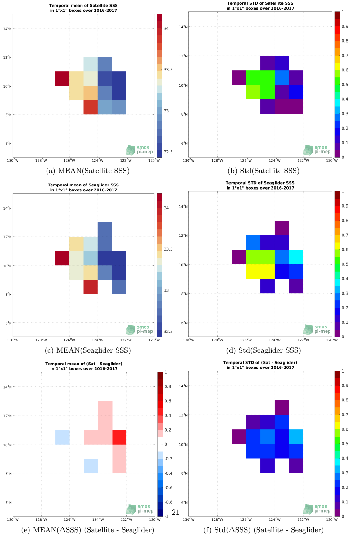
Figure 6: Temporal mean (left) and Std (right) of SSS from SMOS SSS L3 v7 - 18 Days (CATDS-CECOS-LOCEAN) (top), Seaglider (middle), and of \Delta SSS (Satellite - Seaglider). Only match-up pairs are used to generate these maps.
