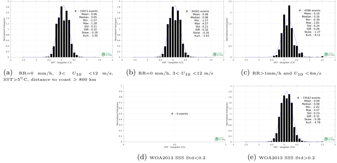
Figure 12: Normalized histogram of \Delta SSS (SMOS SSS L3 v7 - 18 Days (CATDS-CECOS-LOCEAN) - Seaglider) for 5 different subdatasets corresponding to: RR=0 mm/h, 3 < U_{10} < 12 m/s, SST>5°C, distance to coast > 800 km (a), RR=0 mm/h, 3 < U_{10} < 12 m/s (b), RR>1mm/h and U_{10} < 4 m/s (c), WOA2013 SSS Std<0.2 (d), WOA2013 SSS Std>0.2 (e).
