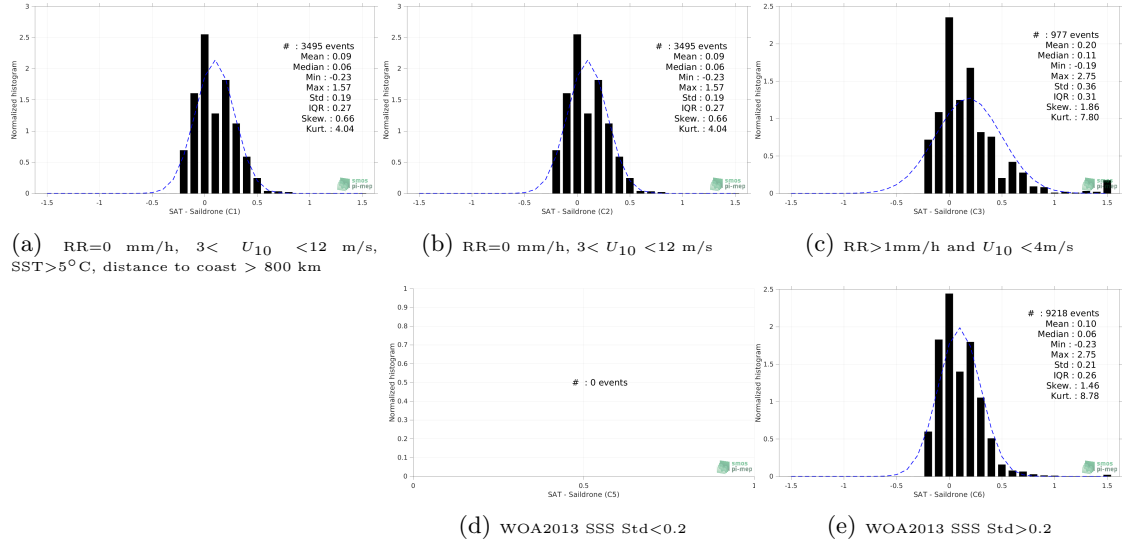
Figure 13: Normalized histogram of \Delta SSS (SMOS SSS L3 v7 - 18 Days (CATDS-CECOS-LOCEAN) - Saildrone) for 5 different subdatasets corresponding to: RR=0 mm/h, 3 < U_{10} < 12 m/s, SST > 5°C, distance to coast > 800 km (a), RR=0 mm/h, 3 < U_{10} < 12 m/s (b), RR > 1mm/h and U_{10} < 4 m/s (c), WOA2013 SSS Std < 0.2 (d), WOA2013 SSS Std > 0.2 (e).
