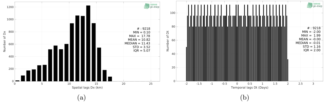
Figure 5: Histograms of the spatial (a) and temporal (b) lags between the location/time of the Saildrone measurement and the date of the corresponding SMOS SSS L3 v7 - 18 Days (CATDS-CECOS-LOCEAN) SSS pixel.
