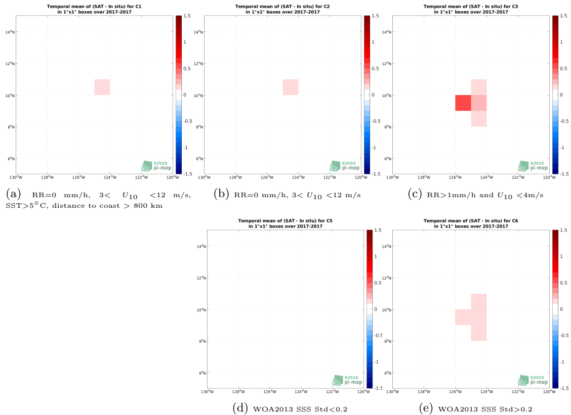
Figure 12: Temporal mean gridded over spatial boxes of size 1^\circ \times 1^\circ of \Delta SSS (SMOS SSS L3 v7 - 18 Days (CATDS-CECOS-LOCEAN) - Saildrone) for 5 different subdatasets corresponding to:RR=0 mm/h, 3 < U_{10} < 12 m/s, SST >5^\circ C, distance to coast > 800 km (a), RR=0 mm/h, 3 < U_{10} < 12 m/s (b), RR >1 mm/h and U_{10} < 4 m/s (c), WOA2013 SSS Std <0.2 (d), WOA2013 SSS Std >0.2 (e).
