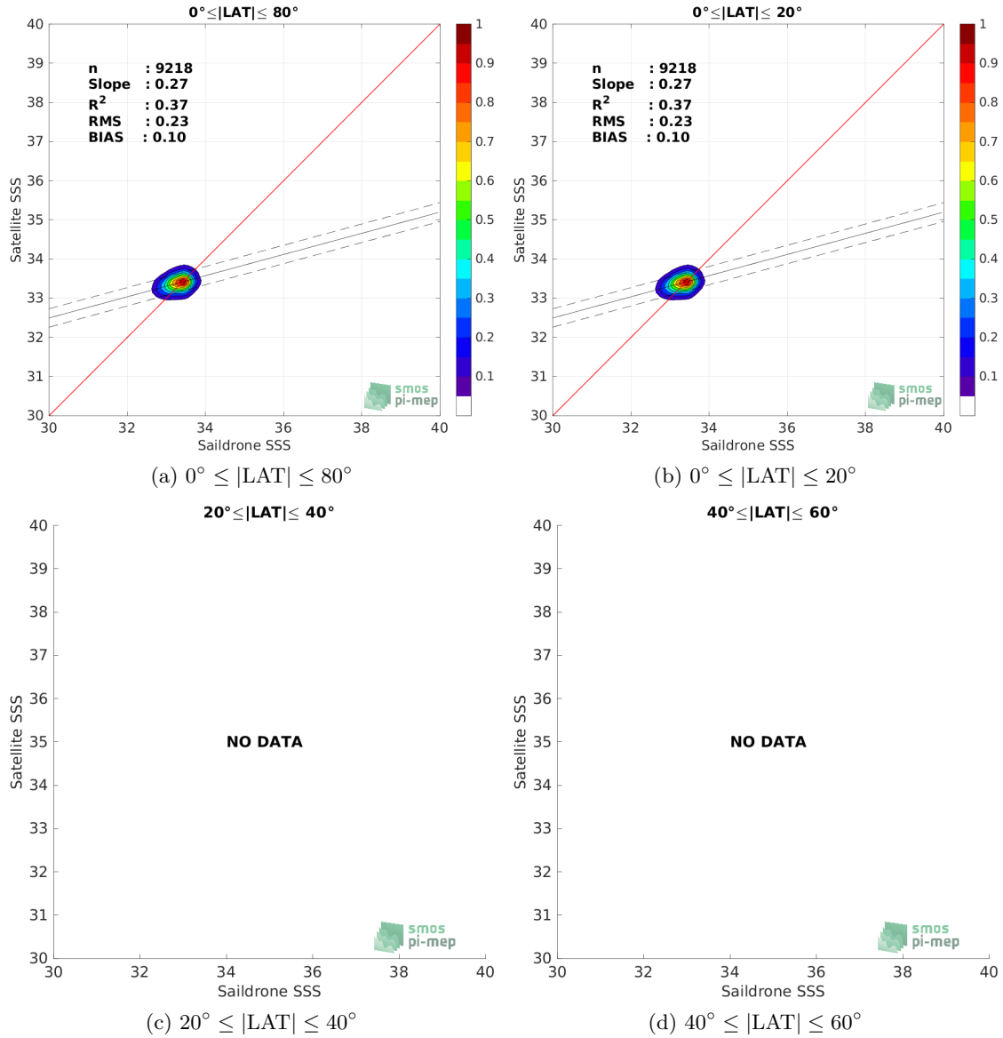
Figure 9: Contour maps of the concentration of SMOS SSS L3 v7 - 18 Days (CATDS-CECOS-LOCEAN) SSS (y-axis) versus Saildrone SSS (x-axis) at match-up pairs for different latitude bands. For each plot, the red line shows x=y . The black thin and dashed lines indicate a linear fit through the data cloud and the \pm 95\% confidence levels, respectively. The number match-up pairs n , the slope and R^2 coefficient of the linear fit, the root mean square (RMS) and the mean bias between satellite and in situ data are indicated for each latitude band in each plots.
