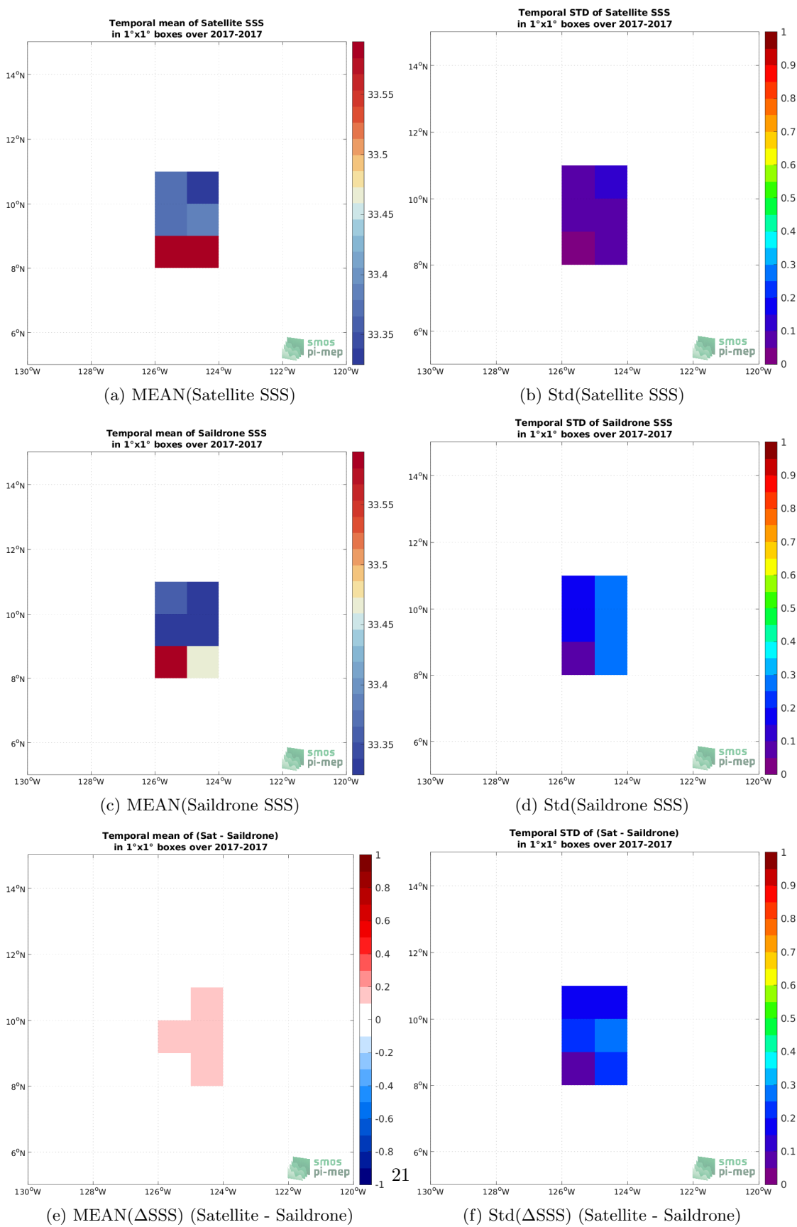
Figure 6: Temporal mean (left) and Std (right) of SSS from SMOS SSS L3 v7 - 18 Days (CATDS-CECOS-LOCEAN) (top), Saildrone (middle), and of \Delta SSS (Satellite - Saildrone). Only match-pairs are used to generate these maps.
