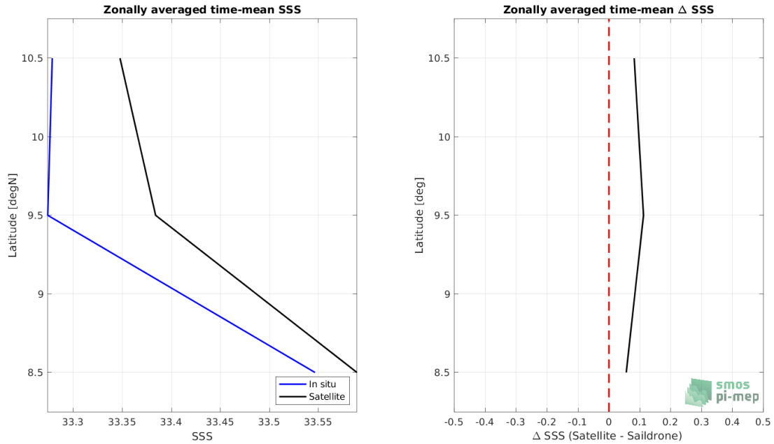
Figure 8: Left panel: Zonal mean SSS from SMOS SSS L3 v7 - 18 Days (CATDS-CECOS-LOCEAN) satellite product (black) and from Sairdrone (blue). Right panel: Zonal mean of \Delta SSS (Satellite - Sairdrone) for all the collected Pi-MEP match-up pairs estimated over the full satellite product period.
