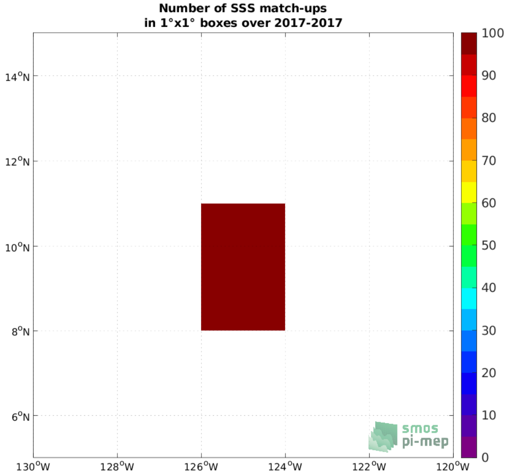
Figure 4: Number of SSS match-ups between Saildrone SSS and the SMOS SSS L3 v7 - 18 Days (CATDS-CECOS-LOCEAN) SSS product for the SPURS 2 Pi-MEP region over 1^\circ \times 1^\circ boxes and for the full satellite product period.
