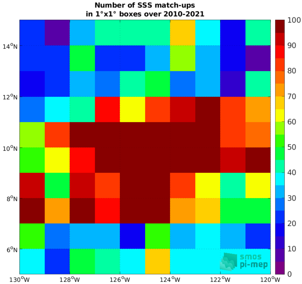
Figure 4: Number of SSS match-ups between Argo SSS and the SMOS SSS L3 v7 - 18 Days (CATDS-CECOS-LOCEAN) SSS product for the SPURS 2 Pi-MEP region over 1°x1° boxes and for the full satellite product period.
