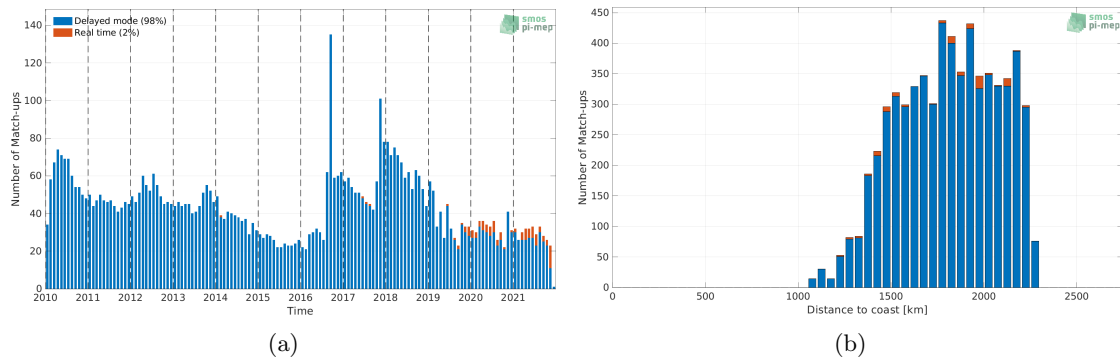
Figure 1: Number of match-ups between Argo and SMOS SSS L3 v7 - 18 Days (CATDS-CECOS-LOCEAN) SSS as a function of time (a) and as function of the distance to coast (b) over the SPURS 2 Pi-MEP region and for the full satellite product period.
