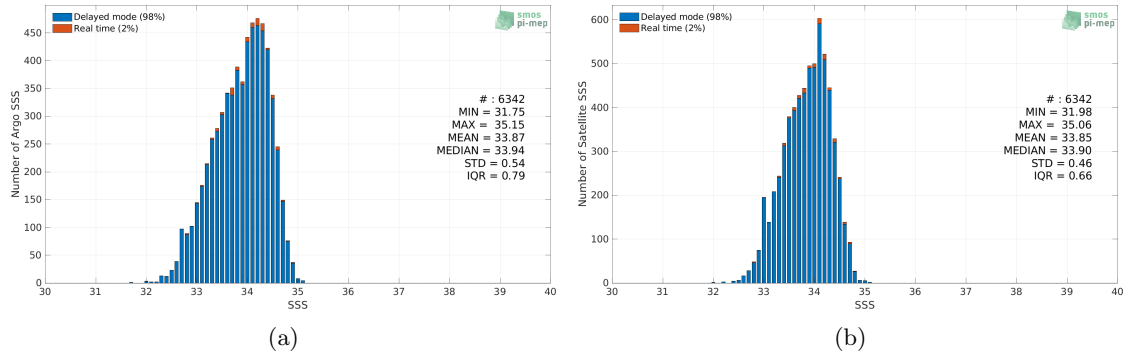
Figure 2: Histograms of SSS from Argo (a) and SMOS SSS L3 v7 - 18 Days (CATDS-CECOS-LOCEAN) (b) considering all match-up pairs per bins of 0.1 over the SPURS 2 Pi-MEP region and for the full satellite product period.
