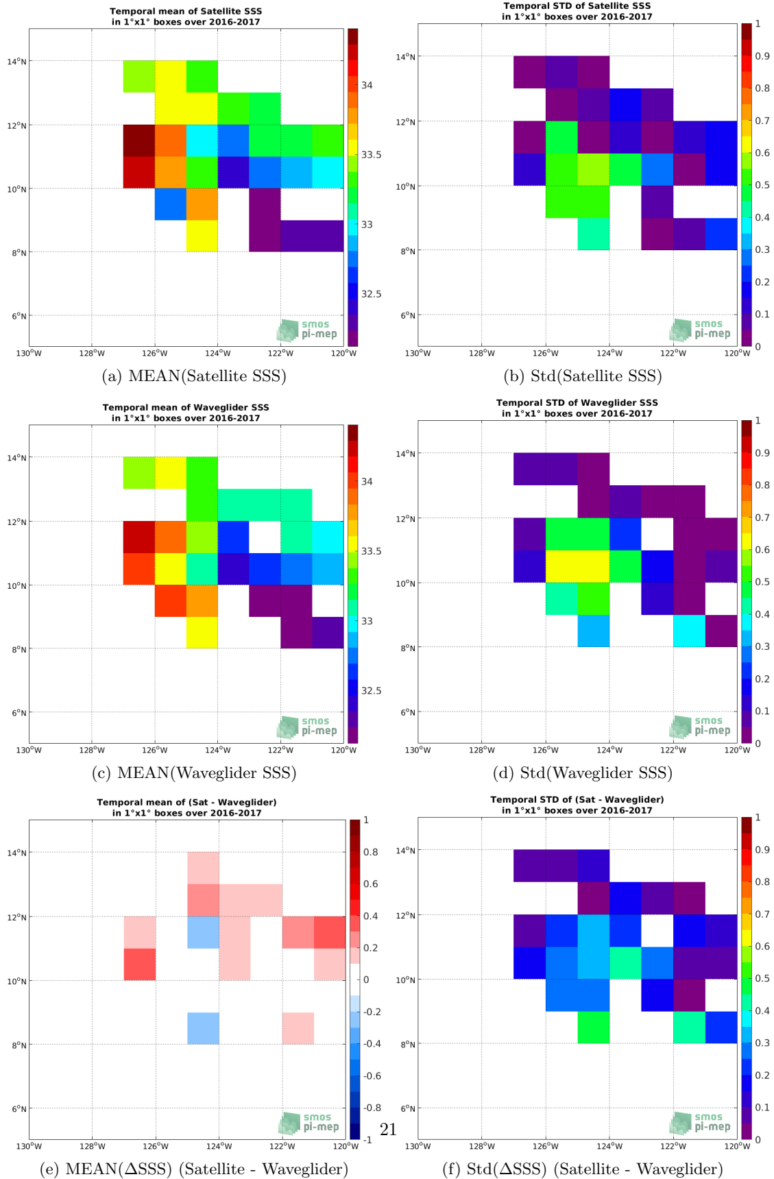
Figure 5: Temporal mean (left) and Std (right) of SSS from SMOS SSS L3 v5 - 9 Days (CATDS-CECOS-LOCEAN) (top), Waveglider (middle), and of \Delta SSS (Satellite - Waveglider). Only match-up pairs are used to generate these maps.
