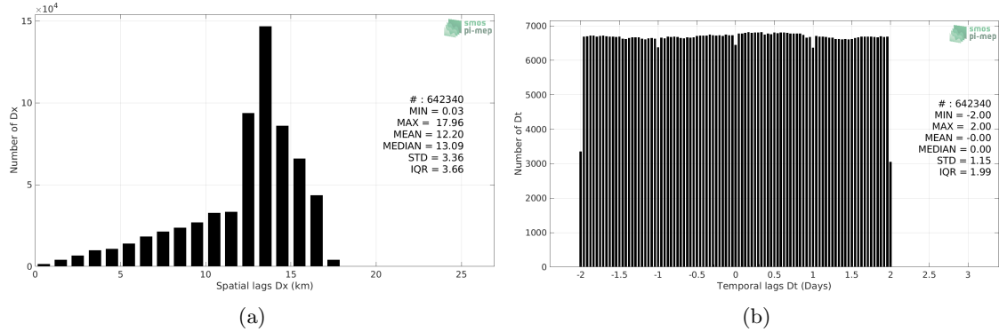
Figure 4: Histograms of the spatial (a) and temporal (b) lags between the location/time of the Waveglider measurement and the date of the corresponding SMOS SSS L3 v5 - 9 Days (CATDS-CECOS-LOCEAN) SSS pixel.
