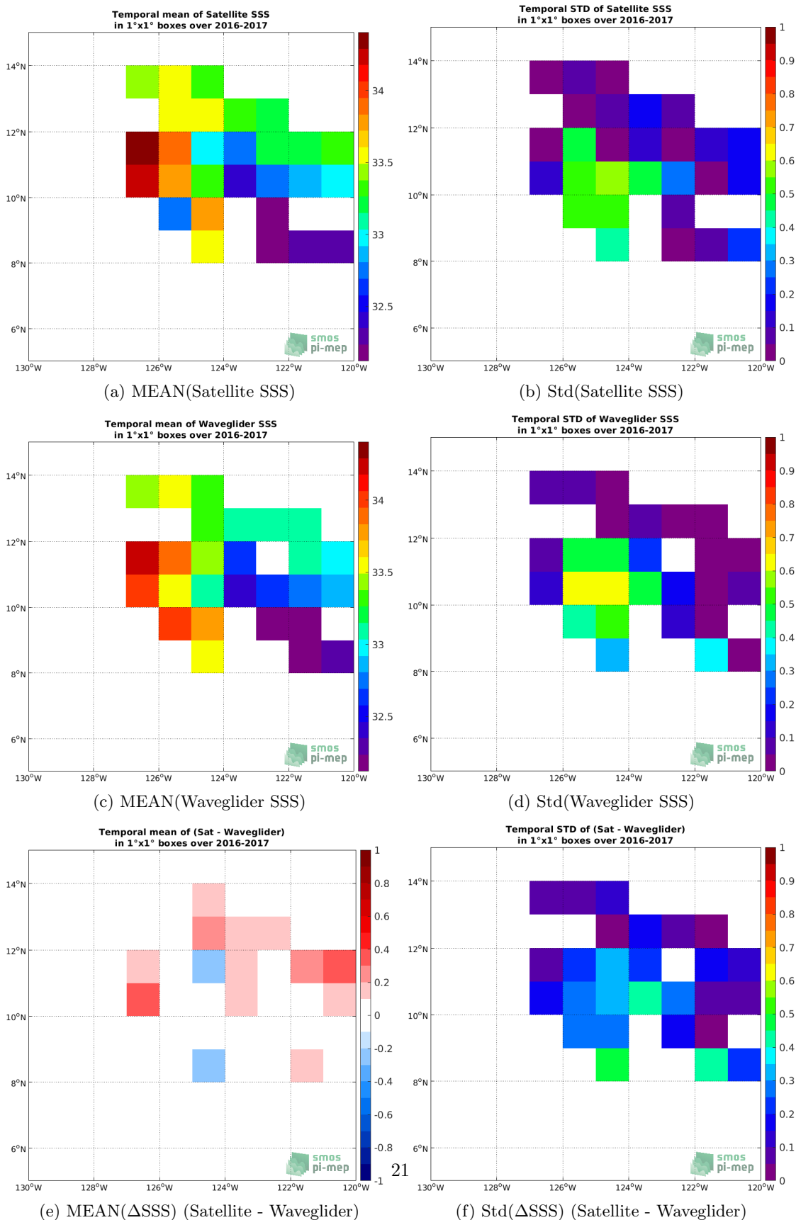
Figure 5: Temporal mean (left) and Std (right) of SSS from SMOS SSS L3 v5 - 9 Days (CATDS-CECOS-LOCEAN) (top), Waveglider (middle), and of \Delta SSS (Satellite - Waveglider). Only match-up pairs are used to generate these maps.
