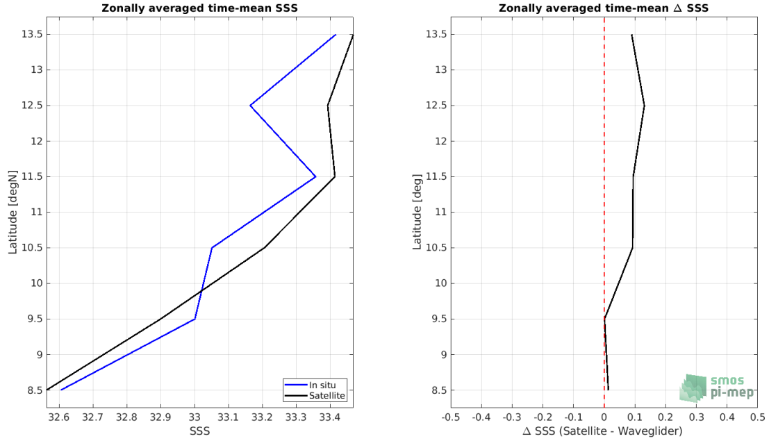
Figure 7: Left panel: Zonal mean SSS from SMOS SSS L3 v5 - 9 Days (CATDS-CECOS-LOCEAN) satellite product (black) and from Waveglider (blue). Right panel: Zonal mean of \Delta SSS (Satellite - Waveglider) for all the collected Pi-MEP match-up pairs estimated over the full satellite product period.
