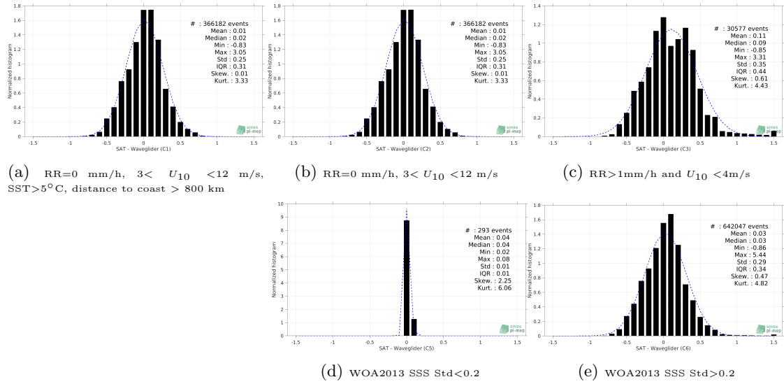
Figure 12: Normalized histogram of \Delta SSS (SMOS SSS L3 v5 - 9 Days (CATDS-CECOS-LOCEAN) - Waveglider) for 5 different subdatasets corresponding to: RR=0 mm/h, 3 < U_{10} < 12 m/s, SST > 5°C, distance to coast > 800 km (a), RR=0 mm/h, 3 < U_{10} < 12 m/s (b), RR > 1mm/h and U_{10} < 4 m/s (c), WOA2013 SSS Std < 0.2 (d), WOA2013 SSS Std > 0.2 (e).
