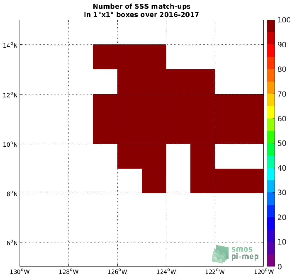
Figure 3: Number of SSS match-ups between Waveglider SSS and the SMOS SSS L3 v5 - 9 Days (CATDS-CECOS-LOCEAN) SSS product for the SPURS 2 Pi-MEP region over 1°x1° boxes and for the full satellite product period.
