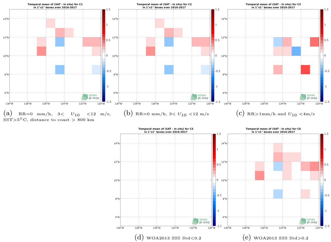
Figure 11: Temporal mean gridded over spatial boxes of size 1^\circ \times 1^\circ of \Delta SSS (SMOS SSS L3 v5 - 9 Days (CATDS-CECOS-LOCEAN) - Waveglider) for 5 different subdatasets corresponding to:RR=0 mm/h, 3 < U_{10} < 12 m/s, SST >5^\circ\text{C} , distance to coast > 800 km (a), RR=0 mm/h, 3 < U_{10} < 12 m/s (b), RR >1 mm/h and U_{10} < 4 m/s (c), WOA2013 SSS Std <0.2 (d), WOA2013 SSS Std >0.2 (e).
