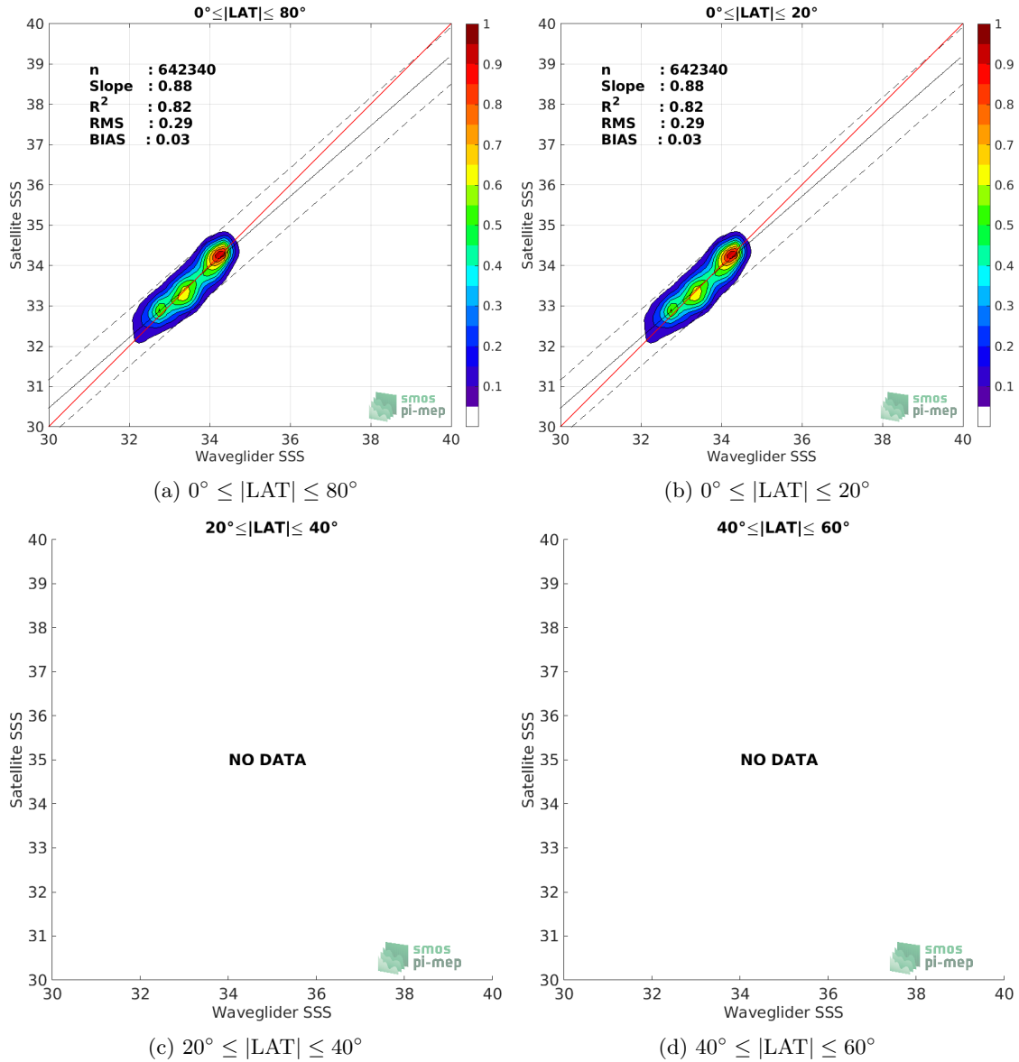
Figure 8: Contour maps of the concentration of SMOS SSS L3 v5 - 9 Days (CATDS-CECOS-LOCEAN) SSS (y-axis) versus Waveglider SSS (x-axis) at match-up pairs for different latitude bands. For each plot, the red line shows x=y . The black thin and dashed lines indicate a linear fit through the data cloud and the \pm 95\% confidence levels, respectively. The number match-up pairs n , the slope and R^2 coefficient of the linear fit, the root mean square (RMS) and the mean bias between satellite and in situ data are indicated for each latitude band in each plots.
