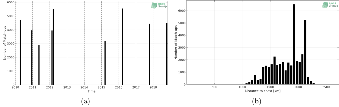
Figure 1: Number of match-ups between TSG (SAMOS) and SMOS SSS L3 v5 - 9 Days (CATDS-CECOS-LOCEAN) SSS as a function of time (a) and as function of the distance to coast (b) over the SPURS 2 Pi-MEP region and for the full satellite product period.
