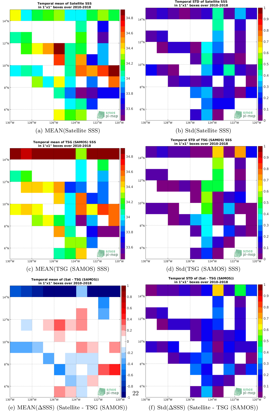
Figure 6: Temporal mean (left) and Std (right) of SSS from SMOS SSS L3 v5 - 9 Days (CATDS-CECOS-LOCEAN) (top), TSG (SAMOS) (middle), and of \Delta SSS (Satellite - TSG (SAMOS)). Only match-up pairs are used to generate these maps.
