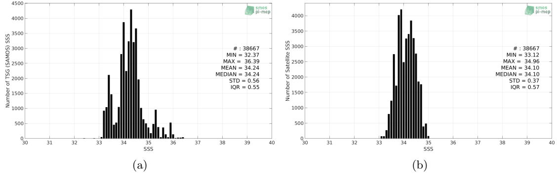
Figure 2: Histograms of SSS from TSG (SAMOS) (a) and SMOS SSS L3 v5 - 9 Days (CATDS-CECOS-LOCEAN) (b) considering all match-up pairs per bins of 0.1 over the SPURS 2 Pi-MEP region and for the full satellite product period.
