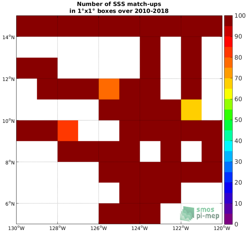
Figure 4: Number of SSS match-ups between TSG (SAMOS) SSS and the SMOS SSS L3 v5 - 9 Days (CATDS-CECOS-LOCEAN) SSS product for the SPURS 2 Pi-MEP region over 1°x1° boxes and for the full satellite product period.
