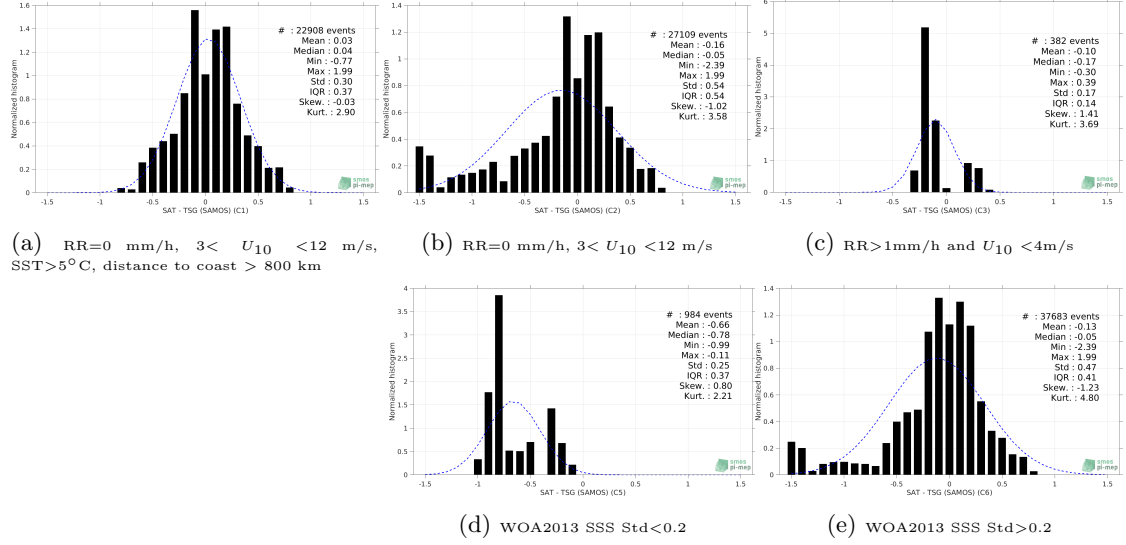
Figure 13: Normalized histogram of \Delta\text{SSS} (SMOS SSS L3 v5 - 9 Days (CATDS-CECOS-LOCEAN) - TSG (SAMOS)) for 5 different subdatasets corresponding to: RR=0 mm/h, 3 < U_{10} < 12 m/s, SST > 5^\circ\text{C} , distance to coast > 800 km (a), RR=0 mm/h, 3 < U_{10} < 12 m/s (b), RR > 1\text{mm/h} and U_{10} < 4\text{m/s} (c), WOA2013 SSS Std < 0.2 (d), WOA2013 SSS Std > 0.2 (e).
