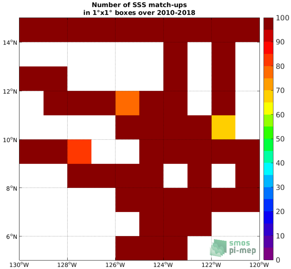
Figure 4: Number of SSS match-ups between TSG (SAMOS) SSS and the SMOS SSS L3 v5 - 9 Days (CATDS-CECOS-LOCEAN) SSS product for the SPURS 2 Pi-MEP region over 1°x1° boxes and for the full satellite product period.
