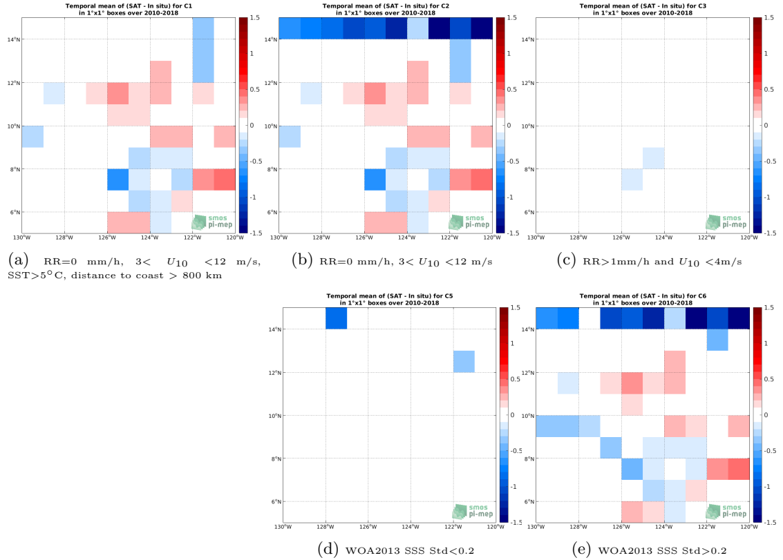
Figure 12: Temporal mean gridded over spatial boxes of size 1^{\circ}\times 1^{\circ} of \Delta\text{SSS} (SMOS SSS L3 v5 - 9 Days (CATDS-CECOS-LOCEAN) - TSG (SAMOS)) for 5 different subdatasets corresponding to: \text{RR}=0 mm/h, 3 < U_{10} < 12 m/s, \text{SST} > 5^{\circ}\text{C} , distance to coast > 800 km (a), \text{RR}=0 mm/h, 3 < U_{10} < 12 m/s (b), \text{RR} > 1 mm/h and U_{10} < 4 m/s (c), WOA2013 SSS Std < 0.2 (d), WOA2013 SSS Std > 0.2 (e).
