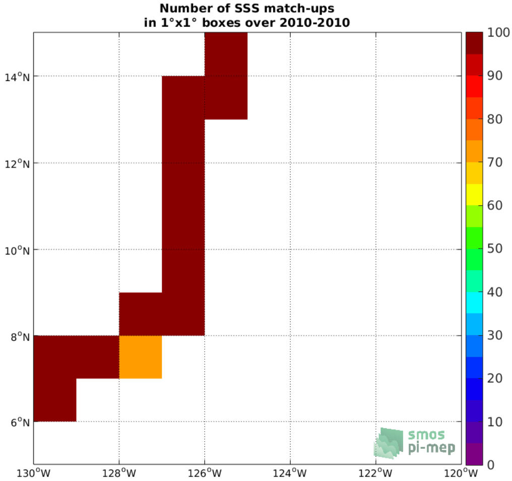
Figure 4: Number of SSS match-ups between TSG (GOSUD-Sailing-ship) SSS and the SMOS SSS L3 v5 - 9 Days (CATDS-CECOS-LOCEAN) SSS product for the SPURS 2 Pi-MEP region over 1^\circ \times 1^\circ boxes and for the full satellite product period.
