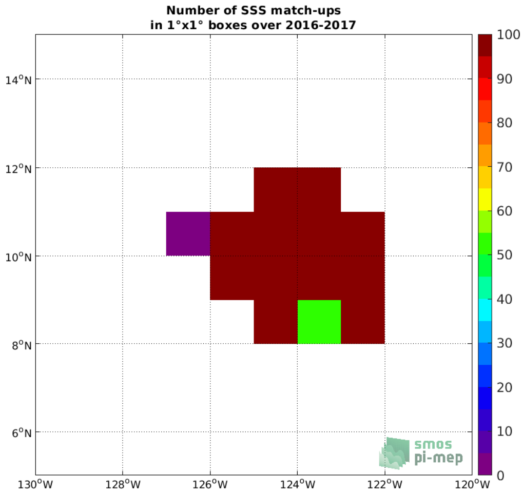
Figure 3: Number of SSS match-ups between Seaglider SSS and the SMOS SSS L3 v5 - 9 Days (CATDS-CECOS-LOCEAN) SSS product for the SPURS 2 Pi-MEP region over 1°x1° boxes and for the full satellite product period.
