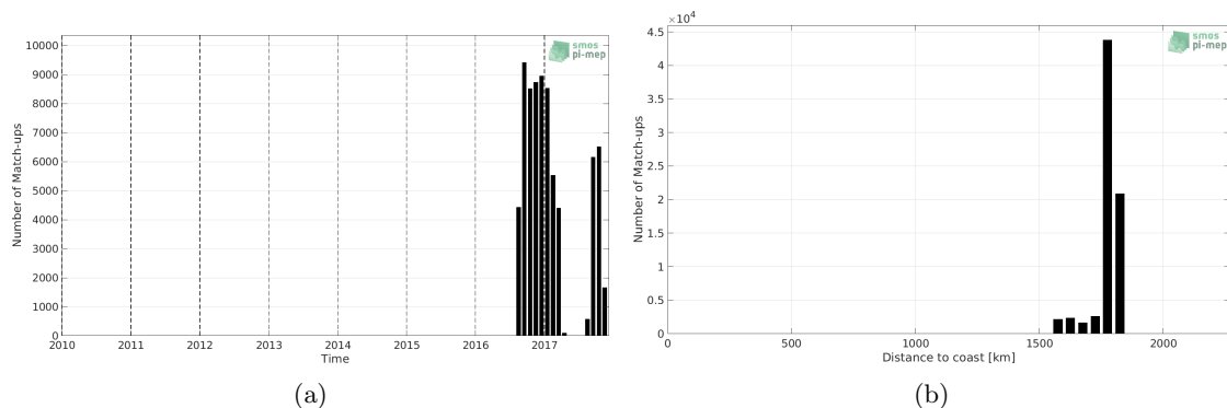
Figure 1: Number of match-ups between Seaglider and SMOS SSS L3 v5 - 9 Days (CATDS-CECOS-LOCEAN) SSS as a function of time (a) and as function of the distance to coast (b) over the SPURS 2 Pi-MEP region and for the full satellite product period.
