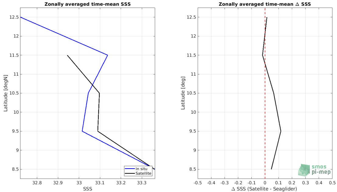
Figure 7: Left panel: Zonal mean SSS from SMOS SSS L3 v5 - 9 Days (CATDS-CECOS-LOCEAN) satellite product (black) and from Seaglider (blue). Right panel: Zonal mean of \Delta SSS (Satellite - Seaglider) for all the collected Pi-MEP match-up pairs estimated over the full satellite product period.
