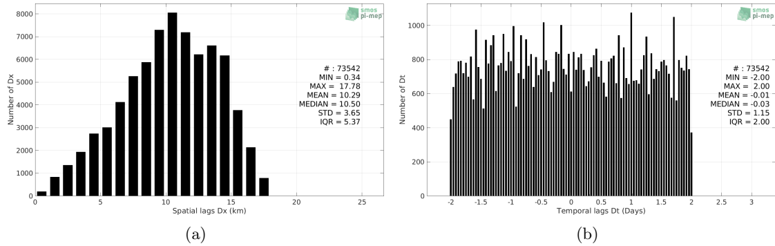
Figure 4: Histograms of the spatial (a) and temporal (b) lags between the location/time of the Seaglider measurement and the date of the corresponding SMOS SSS L3 v5 - 9 Days (CATDS-CECOS-LOCEAN) SSS pixel.
