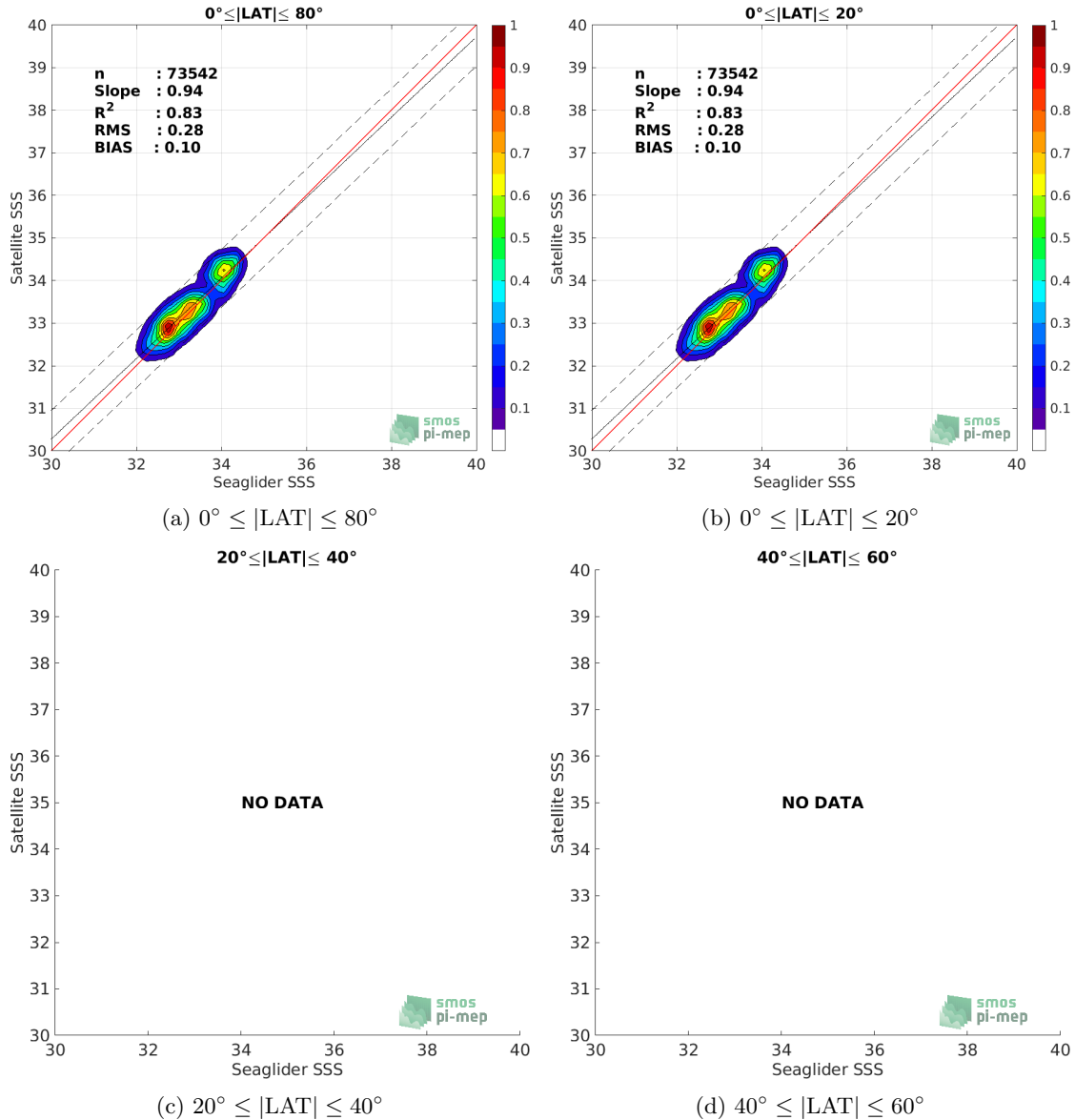
Figure 8: Contour maps of the concentration of SMOS SSS L3 v5 - 9 Days (CATDS-CECOS-LOCEAN) SSS (y-axis) versus Seaglider SSS (x-axis) at match-up pairs for different latitude bands. For each plot, the red line shows x=y . The black thin and dashed lines indicate a linear fit through the data cloud and the \pm 95\% confidence levels, respectively. The number match-up pairs n , the slope and R^2 coefficient of the linear fit, the root mean square (RMS) and the mean bias between satellite and in situ data are indicated for each latitude band in each plots.
