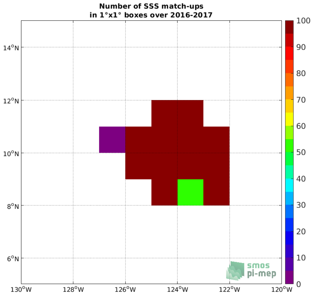
Figure 3: Number of SSS match-ups between Seagliders SSS and the SMOS SSS L3 v5 - 9 Days (CATDS-CECOS-LOCEAN) SSS product for the SPURS 2 Pi-MEP region over 1°x1° boxes and for the full satellite product period.
