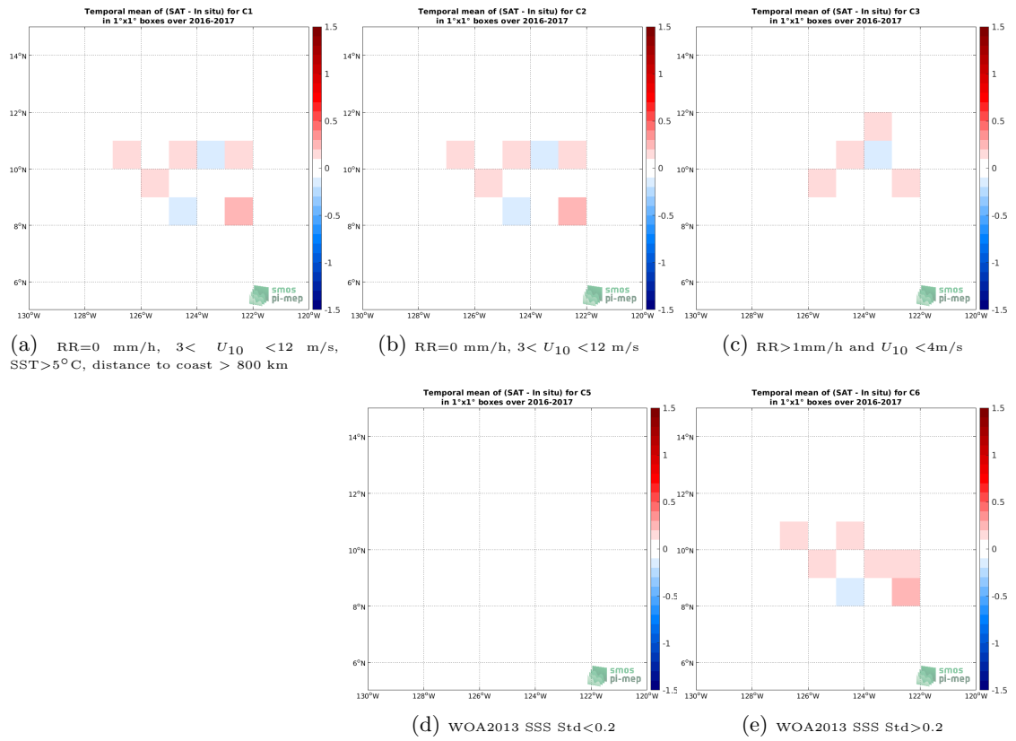
Figure 11: Temporal mean gridded over spatial boxes of size 1^\circ \times 1^\circ of \Delta SSS (SMOS SSS L3 v5 - 9 Days (CATDS-CECOS-LOCEAN) - Seaglider) for 5 different subdatasets corresponding to:RR=0 mm/h, 3 < U_{10} < 12 m/s, SST >5^\circ\text{C} , distance to coast > 800 km (a), RR=0 mm/h, 3 < U_{10} < 12 m/s (b), RR >1 mm/h and U_{10} < 4 m/s (c), WOA2013 SSS Std <0.2 (d), WOA2013 SSS Std >0.2 (e).
