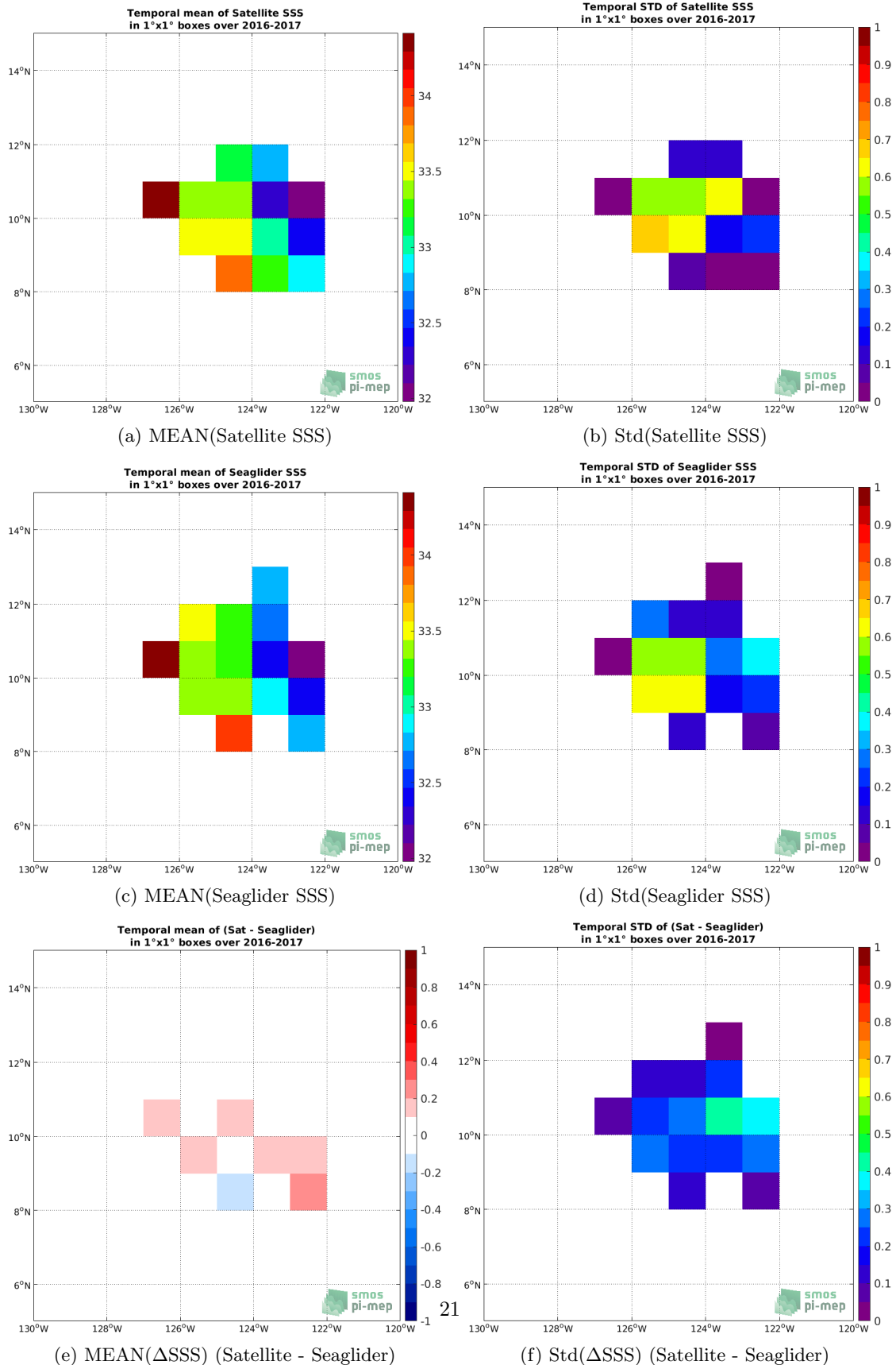
Figure 5: Temporal mean (left) and Std (right) of SSS from SMOS SSS L3 v5 - 9 Days (CATDS-CECOS-LOCEAN) (top), Seaglider (middle), and of \Delta SSS (Satellite - Seaglider). Only match-up pairs are used to generate these maps.
