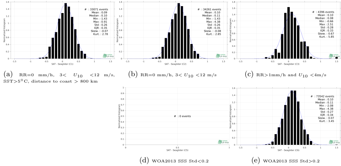
Figure 12: Normalized histogram of \Delta SSS (SMOS SSS L3 v5 - 9 Days (CATDS-CECOS-LOCEAN) - Seaglider) for 5 different subdatasets corresponding to: RR=0 mm/h, 3 < U_{10} < 12 m/s, SST > 5°C, distance to coast > 800 km (a), RR=0 mm/h, 3 < U_{10} < 12 m/s (b), RR > 1mm/h and U_{10} < 4 m/s (c), WOA2013 SSS Std < 0.2 (d), WOA2013 SSS Std > 0.2 (e).
