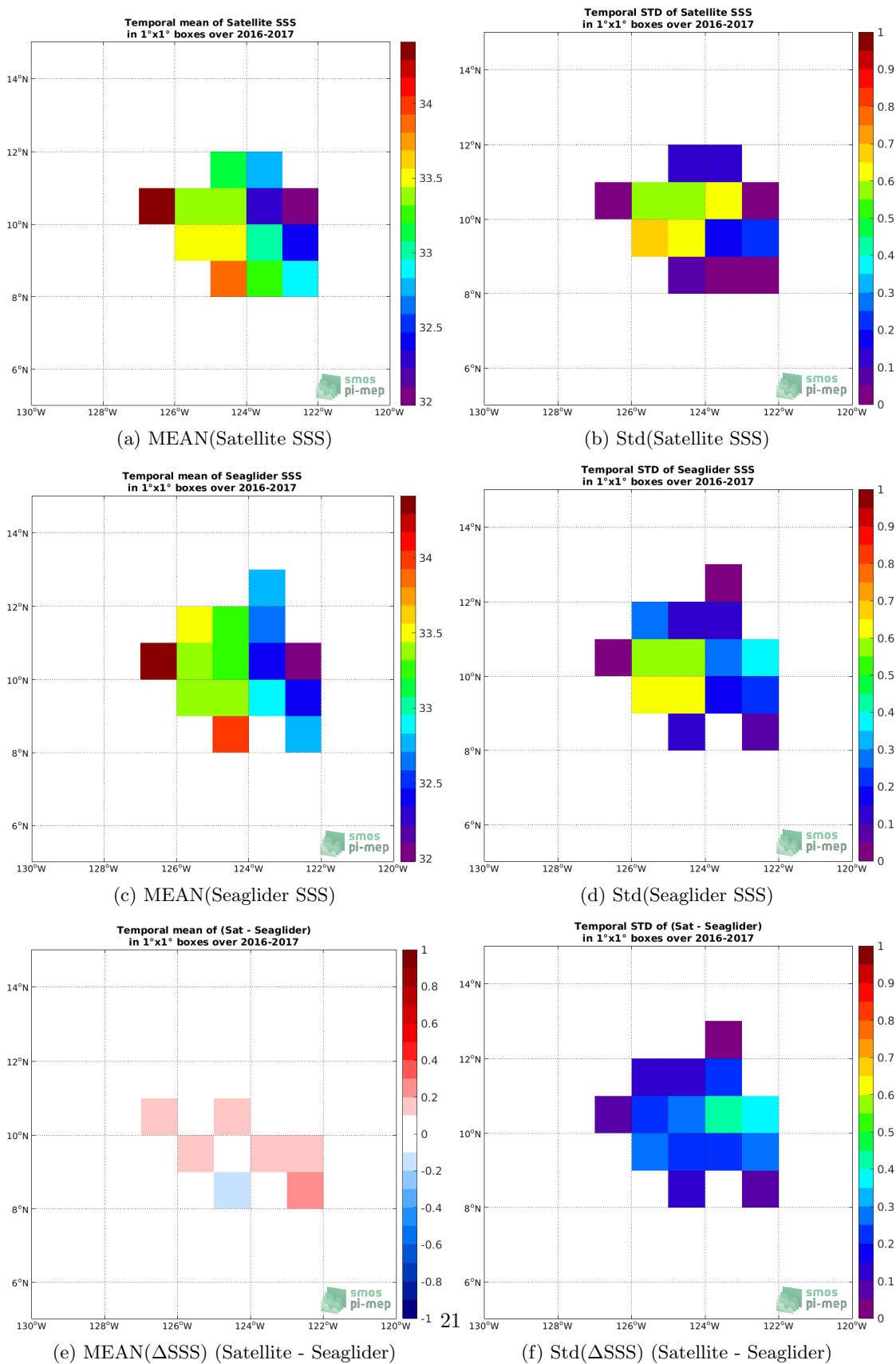
Figure 6: Temporal mean (left) and Std (right) of SSS from SMOS SSS L3 v5 - 9 Days (CATDS-CECOS-LOCEAN) (top), Seaglider (middle), and of \Delta SSS (Satellite - Seaglider). Only match-up pairs are used to generate these maps.
