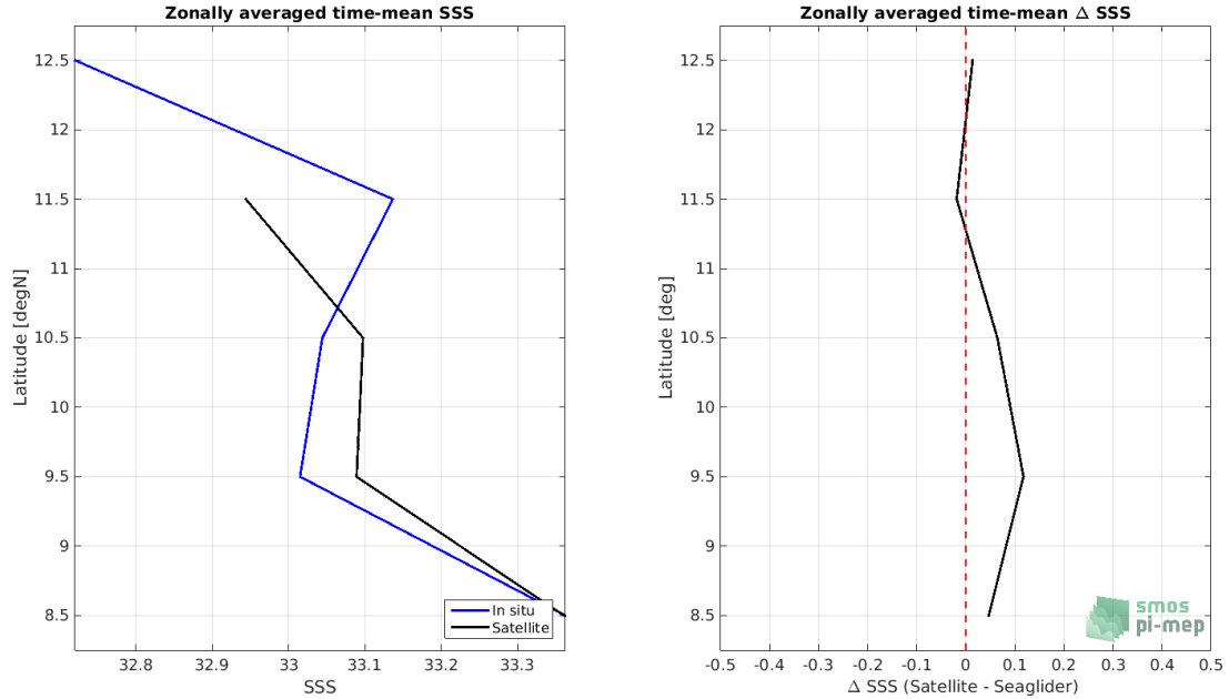
Figure 8: Left panel: Zonal mean SSS from SMOS SSS L3 v5 - 9 Days (CATDS-CECOS-LOCEAN) satellite product (black) and from Seaglider (blue). Right panel: Zonal mean of \Delta SSS (Satellite - Seaglider) for all the collected Pi-MEP match-up pairs estimated over the full satellite product period.
