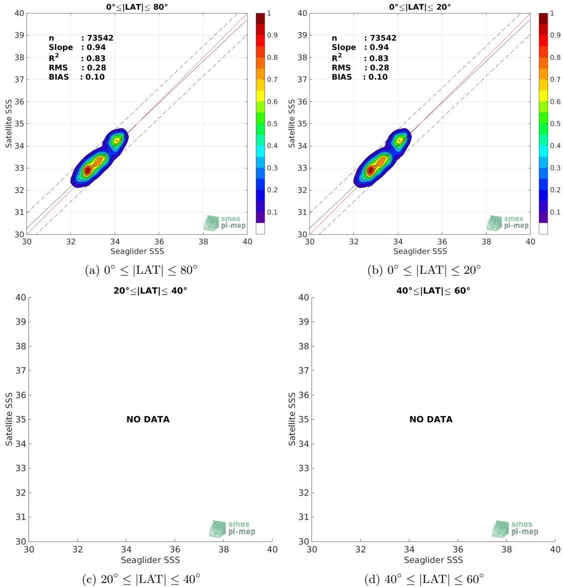
Figure 9: Contour maps of the concentration of SMOS SSS L3 v5 - 9 Days (CATDS-CECOS-LOCEAN) SSS (y-axis) versus Seaglider SSS (x-axis) at match-up pairs for different latitude bands. For each plot, the red line shows x=y . The black thin and dashed lines indicate a linear fit through the data cloud and the \pm 95\% confidence levels, respectively. The number match-up pairs n , the slope and R^2 coefficient of the linear fit, the root mean square (RMS) and the mean bias between satellite and in situ data are indicated for each latitude band in each plots.
