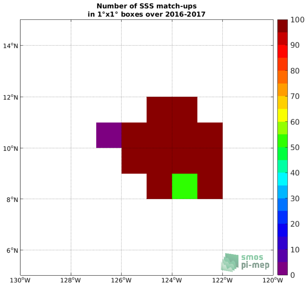
Figure 4: Number of SSS match-ups between Seaglider SSS and the SMOS SSS L3 v5 - 9 Days (CATDS-CECOS-LOCEAN) SSS product for the SPURS 2 Pi-MEP region over 1°x1° boxes and for the full satellite product period.
