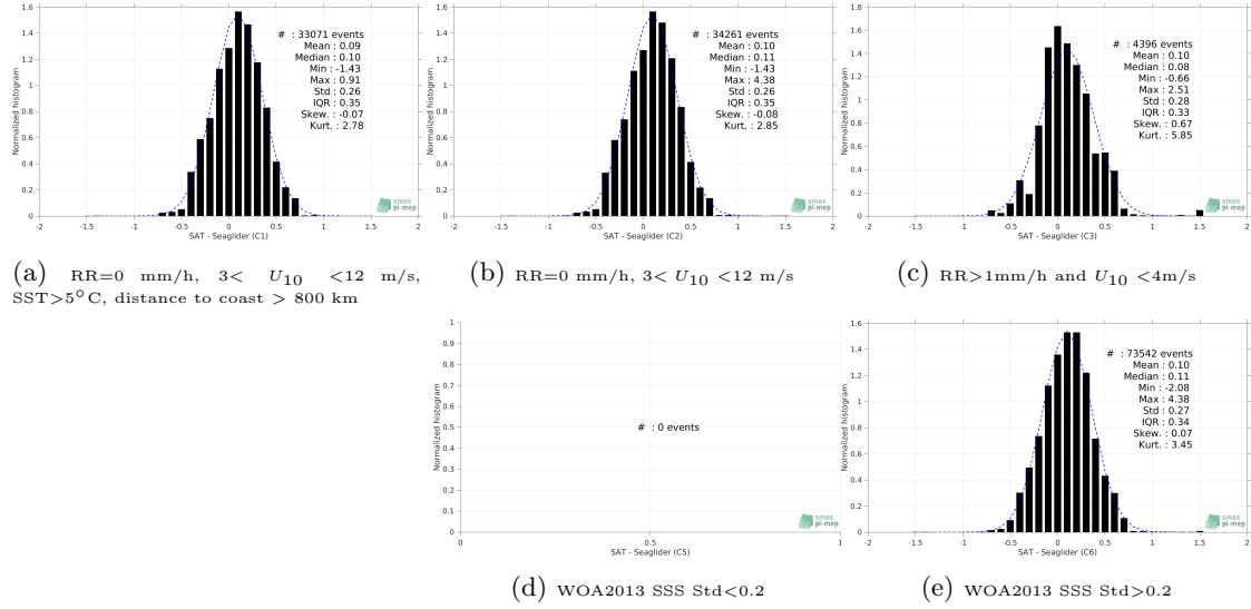
Figure 13: Normalized histogram of \Delta SSS (SMOS SSS L3 v5 - 9 Days (CATDS-CECOS-LOCEAN) - Seagliders) for 5 different subdatasets corresponding to: RR=0 mm/h, 3 < U_{10} < 12 m/s, SST>5°C, distance to coast > 800 km (a), RR=0 mm/h, 3 < U_{10} < 12 m/s (b), RR>1mm/h and U_{10} < 4 m/s (c), WOA2013 SSS Std<0.2 (d), WOA2013 SSS Std>0.2 (e).
