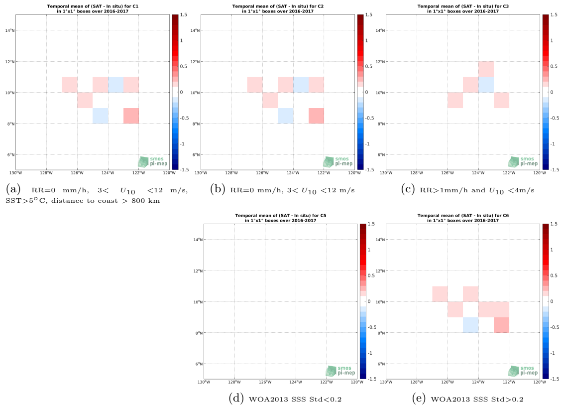
Figure 12: Temporal mean gridded over spatial boxes of size 1^\circ \times 1^\circ of \Delta SSS (SMOS SSS L3 v5 - 9 Days (CATDS-CECOS-LOCEAN) - Seaglider) for 5 different subdatasets corresponding to:RR=0 mm/h, 3 < U_{10} < 12 m/s, SST >5^\circ\text{C} , distance to coast > 800 km (a), RR=0 mm/h, 3 < U_{10} < 12 m/s (b), RR >1 mm/h and U_{10} < 4 m/s (c), WOA2013 SSS Std <0.2 (d), WOA2013 SSS Std >0.2 (e).
