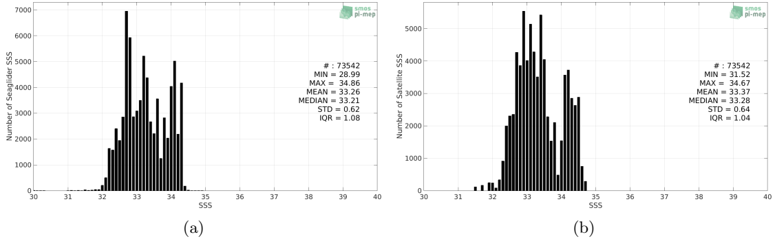
Figure 2: Histograms of SSS from Seaglider (a) and SMOS SSS L3 v5 - 9 Days (CATDS-CECOS-LOCEAN) (b) considering all match-up pairs per bins of 0.1 over the SPURS 2 Pi-MEP region and for the full satellite product period.
