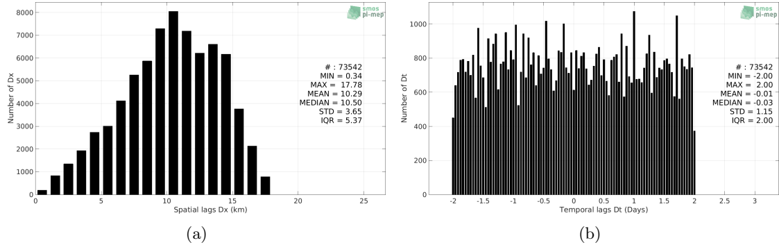
Figure 5: Histograms of the spatial (a) and temporal (b) lags between the time of the Seaglider measurements and the date of the corresponding SMOS SSS L3 v5 - 9 Days (CATDS-CECOS-LOCEAN) SSS product.
