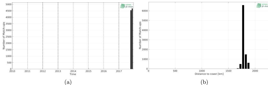
Figure 1: Number of match-ups between Saildrone and SMOS SSS L3 v5 - 9 Days (CATDS-CECOS-LOCEAN) SSS as a function of time (a) and as function of the distance to coast (b) over the SPURS 2 Pi-MEP region and for the full satellite product period.
