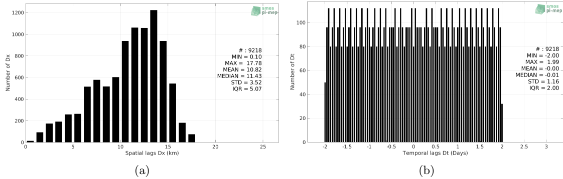
Figure 4: Histograms of the spatial (a) and temporal (b) lags between the location/time of the Saildrone measurement and the date of the corresponding SMOS SSS L3 v5 - 9 Days (CATDS-CECOS-LOCEAN) SSS pixel.
