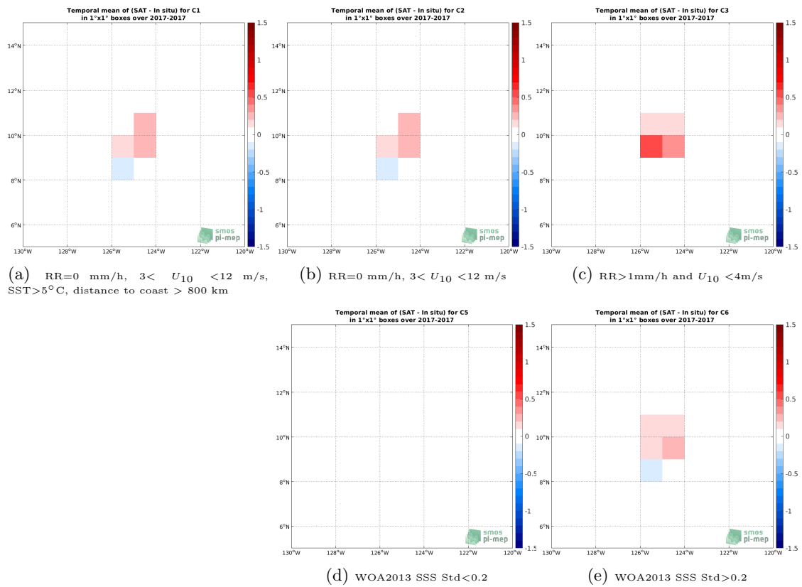
Figure 11: Temporal mean gridded over spatial boxes of size 1^\circ \times 1^\circ of \Delta SSS (SMOS SSS L3 v5 - 9 Days (CATDS-CECOS-LOCEAN) - Saildrone) for 5 different subdatasets corresponding to:RR=0 mm/h, 3 < U_{10} < 12 m/s, SST >5^\circ\text{C} , distance to coast > 800 km (a), RR=0 mm/h, 3 < U_{10} < 12 m/s (b), RR >1 mm/h and U_{10} < 4 m/s (c), WOA2013 SSS Std <0.2 (d), WOA2013 SSS Std >0.2 (e).
