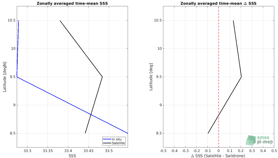
Figure 7: Left panel: Zonal mean SSS from SMOS SSS L3 v5 - 9 Days (CATDS-CECOS-LOCEAN) satellite product (black) and from Sairdrone (blue). Right panel: Zonal mean of \Delta SSS (Satellite - Sairdrone) for all the collected Pi-MEP match-up pairs estimated over the full satellite product period.
