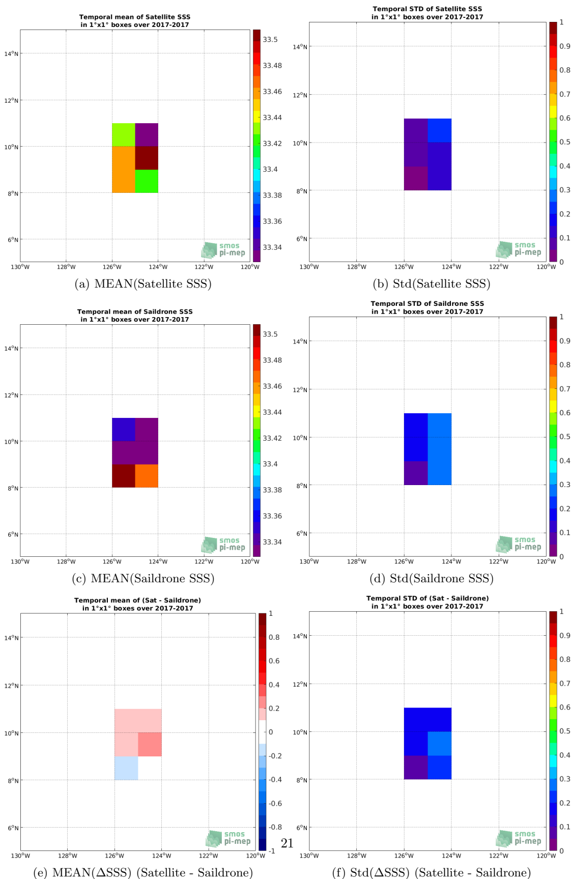
Figure 5: Temporal mean (left) and Std (right) of SSS from SMOS SSS L3 v5 - 9 Days (CATDS-CECOS-LOCEAN) (top), Saildrone (middle), and of \Delta SSS (Satellite - Saildrone). Only match-up pairs are used to generate these maps.
