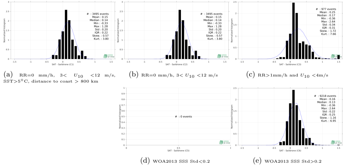
Figure 12: Normalized histogram of \Delta\text{SSS} (SMOS SSS L3 v5 - 9 Days (CATDS-CECOS-LOCEAN) - Saildrone) for 5 different subdatasets corresponding to: RR=0 mm/h, 3 < U_{10} < 12 m/s, SST > 5^\circ\text{C} , distance to coast > 800 km (a), RR=0 mm/h, 3 < U_{10} < 12 m/s (b), RR > 1\text{mm/h} and U_{10} < 4\text{m/s} (c), WOA2013 SSS Std < 0.2 (d), WOA2013 SSS Std > 0.2 (e).
