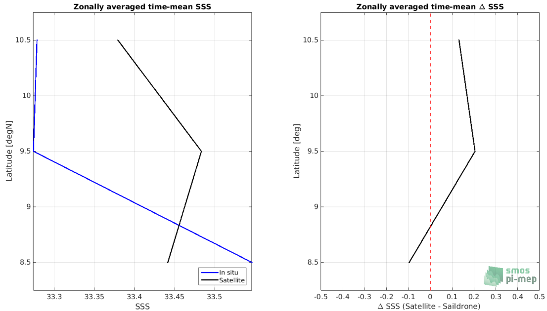
Figure 8: Left panel: Zonal mean SSS from SMOS SSS L3 v5 - 9 Days (CATDS-CECOS-LOCEAN) satellite product (black) and from Saildrone (blue). Right panel: Zonal mean of \Delta SSS (Satellite - Saildrone) for all the collected Pi-MEP match-up pairs estimated over the full satellite product period.
