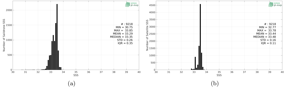
Figure 2: Histograms of SSS from Saildrone (a) and SMOS SSS L3 v5 - 9 Days (CATDS-CECOS-LOCEAN) (b) considering all match-up pairs per bins of 0.1 over the SPURS 2 Pi-MEP region and for the full satellite product period.
