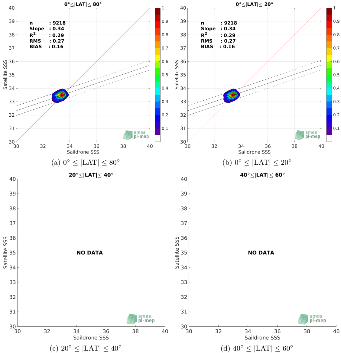
Figure 9: Contour maps of the concentration of SMOS SSS L3 v5 - 9 Days (CATDS-CECOS-LOCEAN) SSS (y-axis) versus Saildrone SSS (x-axis) at match-up pairs for different latitude bands. For each plot, the red line shows x=y . The black thin and dashed lines indicate a linear fit through the data cloud and the \pm 95\% confidence levels, respectively. The number match-up pairs n , the slope and R^2 coefficient of the linear fit, the root mean square (RMS) and the mean bias between satellite and in situ data are indicated for each latitude band in each plots.
