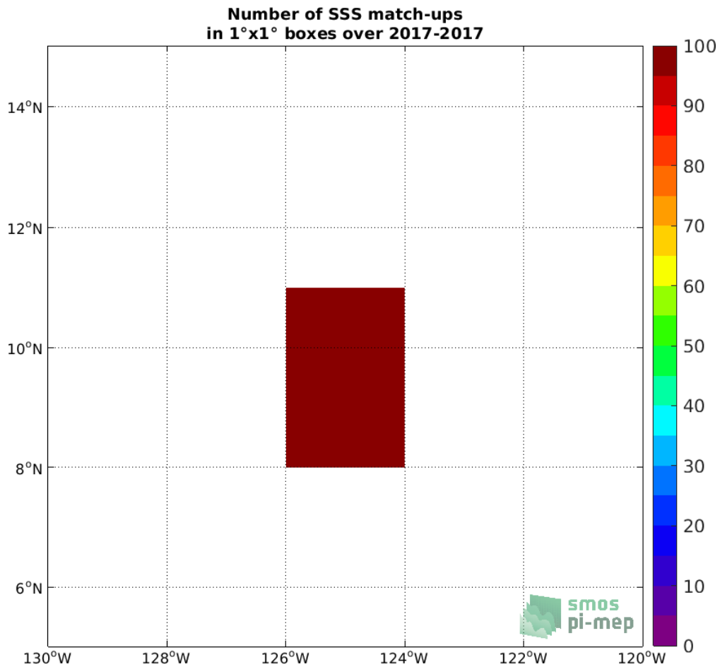
Figure 4: Number of SSS match-ups between Sairdron SSS and the SMOS SSS L3 v5 - 9 Days (CATDS-CECOS-LOCEAN) SSS product for the SPURS 2 Pi-MEP region over 1°x1° boxes and for the full satellite product period.
