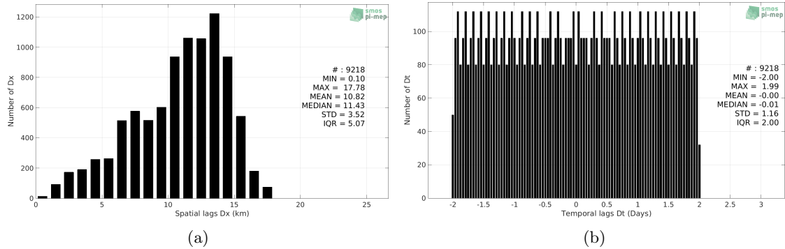
Figure 5: Histograms of the spatial (a) and temporal (b) lags between the time of the Saildrone measurements and the date of the corresponding SMOS SSS L3 v5 - 9 Days (CATDS-CECOS-LOCEAN) SSS product.
