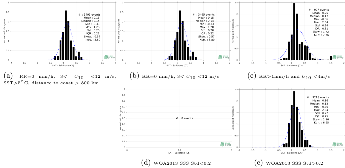
Figure 13: Normalized histogram of \Delta SSS (SMOS SSS L3 v5 - 9 Days (CATDS-CECOS-LOCEAN) - Saildrone) for 5 different subdatasets corresponding to: RR=0 mm/h, 3 < U_{10} < 12 m/s, SST>5°C, distance to coast > 800 km (a), RR=0 mm/h, 3 < U_{10} < 12 m/s (b), RR>1mm/h and U_{10} < 4 m/s (c), WOA2013 SSS Std<0.2 (d), WOA2013 SSS Std>0.2 (e).
