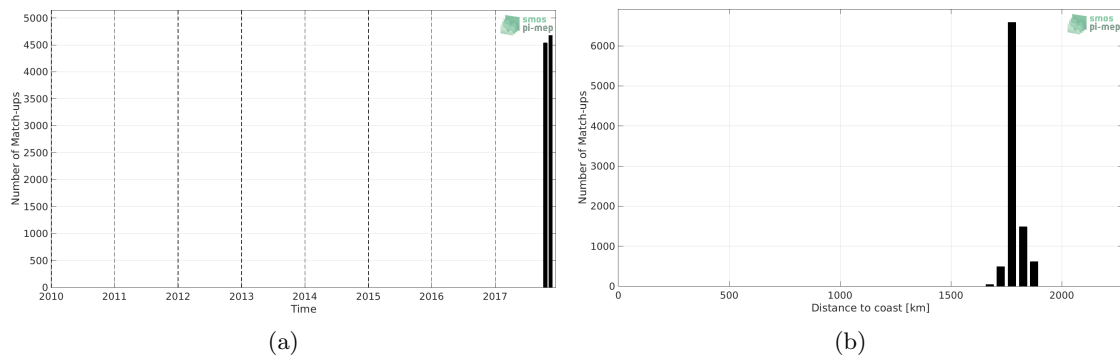
Figure 1: Number of match-ups between Sairdron and SMOS SSS L3 v5 - 9 Days (CATDS-CECOS-LOCEAN) SSS as a function of time (a) and as function of the distance to coast (b) over the SPURS 2 Pi-MEP region and for the full satellite product period.
