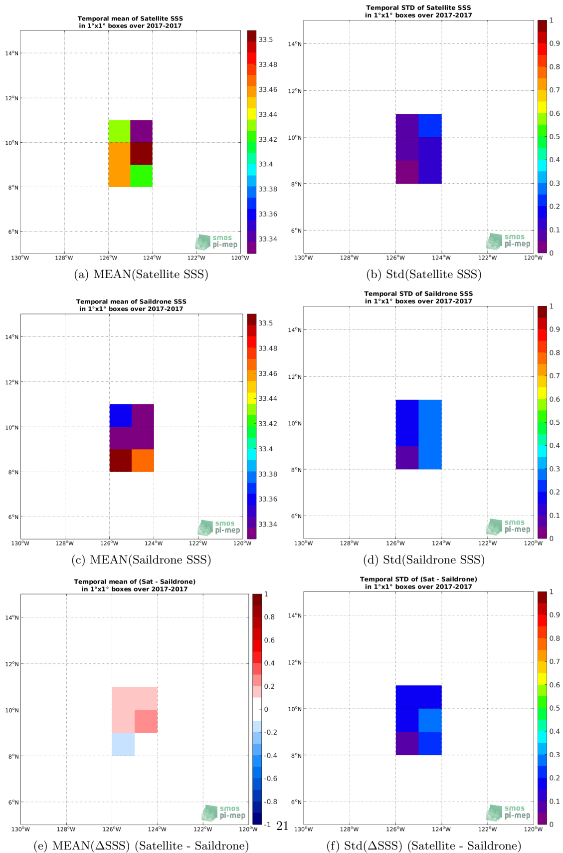
Figure 6: Temporal mean (left) and Std (right) of SSS from SMOS SSS L3 v5 - 9 Days (CATDS-CECOS-LOCEAN) (top), Saildrone (middle), and of \Delta SSS (Satellite - Saildrone). Only match-up pairs are used to generate these maps.
