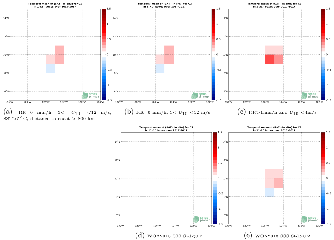
Figure 12: Temporal mean gridded over spatial boxes of size 1^\circ \times 1^\circ of \Delta\text{SSS} (SMOS SSS L3 v5 - 9 Days (CATDS-CECOS-LOCEAN) - Saildrone) for 5 different subdatasets corresponding to:RR=0 mm/h, 3 < U_{10} < 12 m/s, SST >5^\circ\text{C} , distance to coast > 800 km (a), RR=0 mm/h, 3 < U_{10} < 12 m/s (b), RR >1 mm/h and U_{10} < 4 m/s (c), WOA2013 SSS Std <0.2 (d), WOA2013 SSS Std >0.2 (e).
