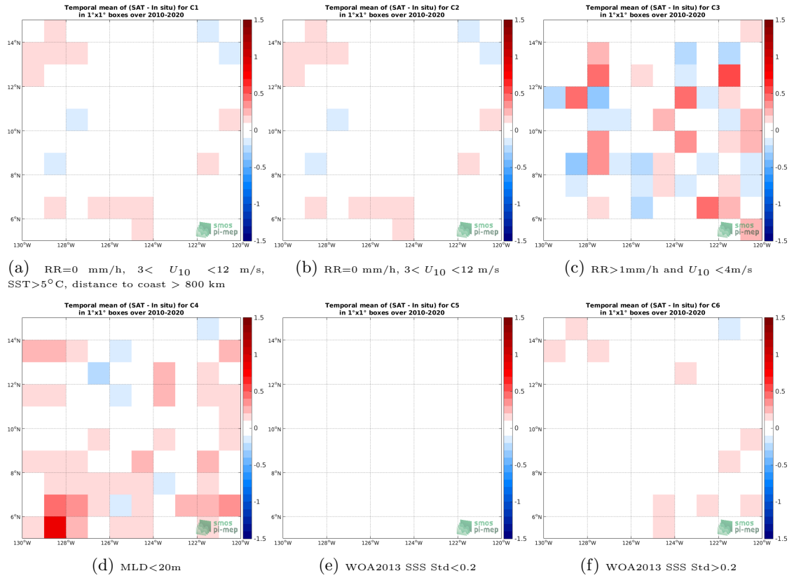
Figure 12: Temporal mean gridded over spatial boxes of size 1^\circ \times 1^\circ of \Delta SSS (SMOS SSS L3 v5 - 9 Days (CATDS-CECOS-LOCEAN) - Argo) for 6 different subdatasets corresponding to:RR=0 mm/h, 3 < U_{10} < 12 m/s, SST >5^\circ C, distance to coast > 800 km (a), RR=0 mm/h, 3 < U_{10} < 12 m/s (b), RR >1 mm/h and U_{10} < 4 m/s (c),MLD <20 m (d),WOA2013 SSS Std <0.2 (e),WOA2013 SSS Std >0.2 (f).
