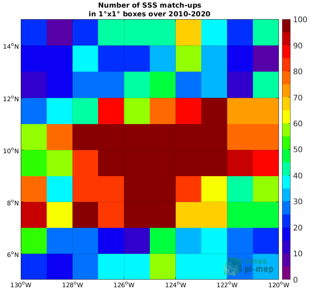
Figure 4: Number of SSS match-ups between Argo SSS and the SMOS SSS L3 v5 - 9 Days (CATDS-CECOS-LOCEAN) SSS product for the SPURS 2 Pi-MEP region over 1°x1° boxes and for the full satellite product period.
