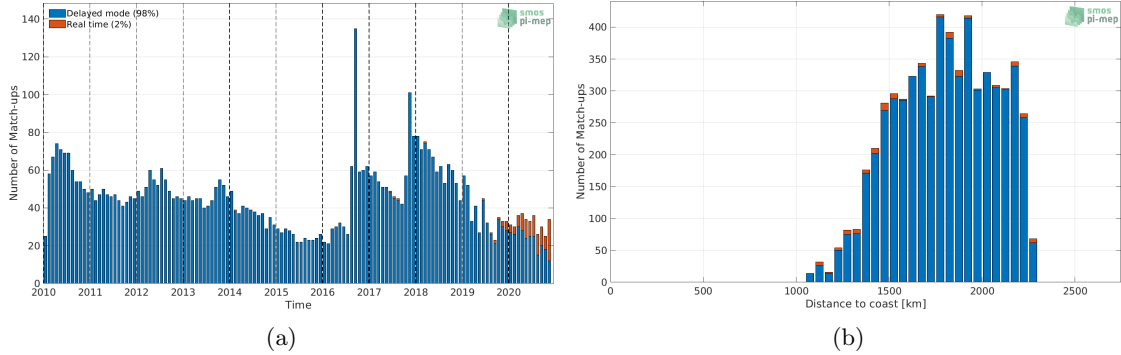
Figure 1: Number of match-ups between Argo and SMOS SSS L3 v5 - 9 Days (CATDS-CECOS-LOCEAN) SSS as a function of time (a) and as function of the distance to coast (b) over the SPURS 2 Pi-MEP region and for the full satellite product period.
