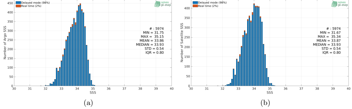
Figure 2: Histograms of SSS from Argo (a) and SMOS SSS L3 v5 - 9 Days (CATDS-CECOS-LOCEAN) (b) considering all match-up pairs per bins of 0.1 over the SPURS 2 Pi-MEP region and for the full satellite product period.
