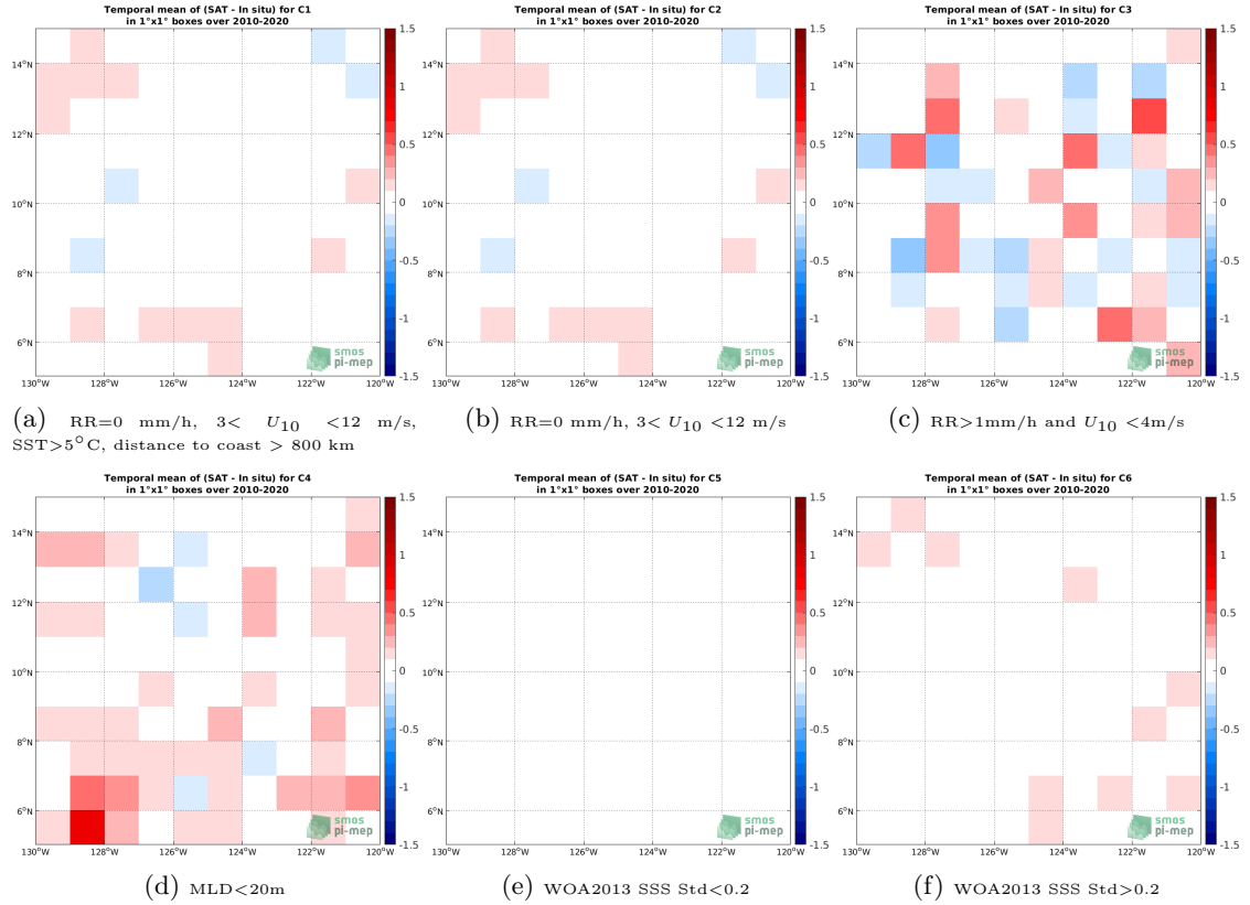
Figure 12: Temporal mean gridded over spatial boxes of size 1^\circ \times 1^\circ of \Delta SSS (SMOS SSS L3 v5 - 9 Days (CATDS-CECOS-LOCEAN) - Argo) for 6 different subdatasets corresponding to: RR=0 mm/h, 3 < U_{10} < 12 m/s, SST > 5^\circ C , distance to coast > 800 km (a), RR=0 mm/h, 3 < U_{10} < 12 m/s (b), RR > 1 mm/h and U_{10} < 4 m/s (c), MLD < 20 m (d), WOA2013 SSS Std < 0.2 (e), WOA2013 SSS Std > 0.2 (f).
