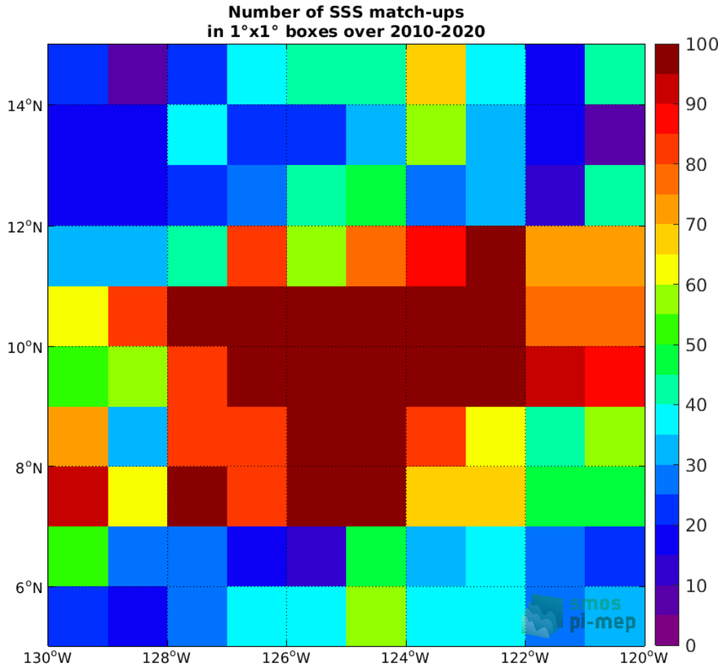
Figure 4: Number of SSS match-ups between Argo SSS and the SMOS SSS L3 v5 - 9 Days (CATDS-CECOS-LOCEAN) SSS product for the SPURS 2 Pi-MEP region over 1°x1° boxes and for the full satellite product period.
