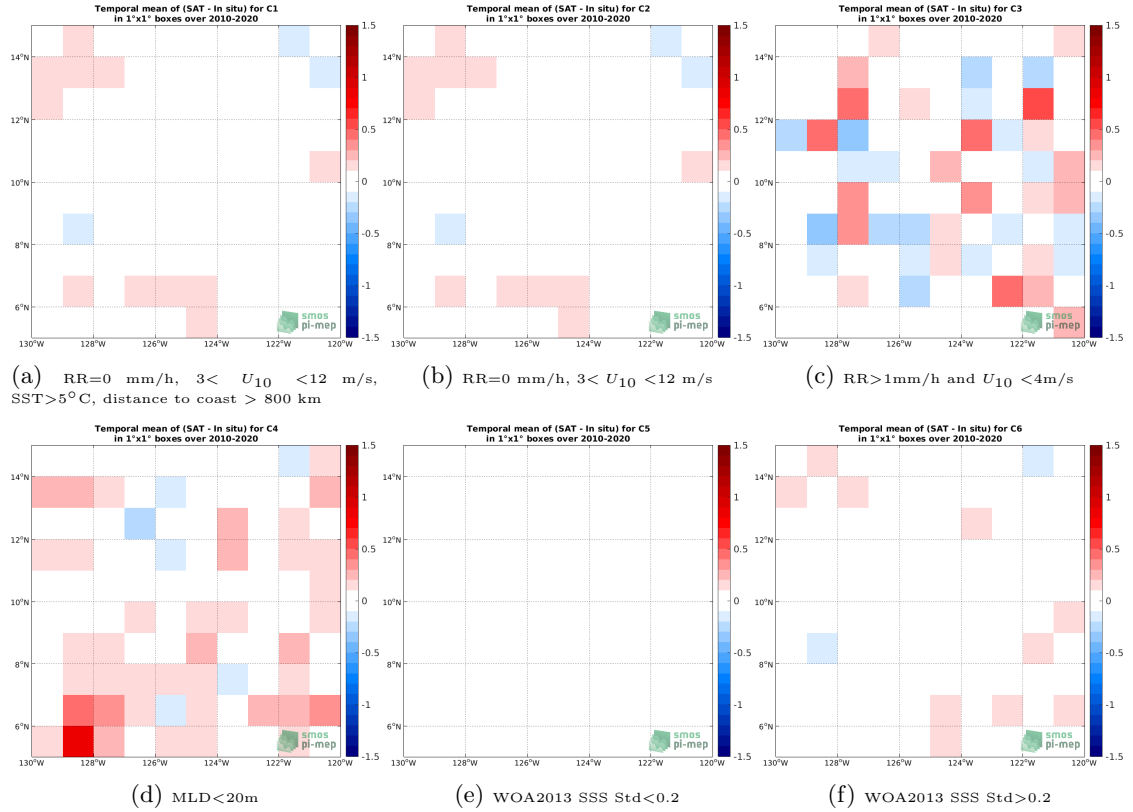
Figure 12: Temporal mean gridded over spatial boxes of size 1^\circ \times 1^\circ of \Delta SSS (SMOS SSS L3 v5 - 9 Days (CATDS-CECOS-LOCEAN) - Argo) for 6 different subdatasets corresponding to:RR=0 mm/h, 3 < U_{10} < 12 m/s, SST >5^\circ C, distance to coast > 800 km (a), RR=0 mm/h, 3 < U_{10} < 12 m/s (b), RR >1 mm/h and U_{10} < 4 m/s (c),MLD <20 m (d),WOA2013 SSS Std <0.2 (e),WOA2013 SSS Std >0.2 (f).
