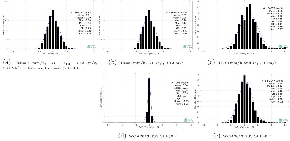
Figure 12: Normalized histogram of \Delta SSS (SMOS SSS L3 v5 - 18 Days (CATDS-CECOS-LOCEAN) - Waveglider) for 5 different subdatasets corresponding to: RR=0 mm/h, 3 < U_{10} < 12 m/s, SST>5°C, distance to coast > 800 km (a), RR=0 mm/h, 3 < U_{10} < 12 m/s (b), RR>1mm/h and U_{10} < 4 m/s (c), WOA2013 SSS Std<0.2 (d), WOA2013 SSS Std>0.2 (e).
