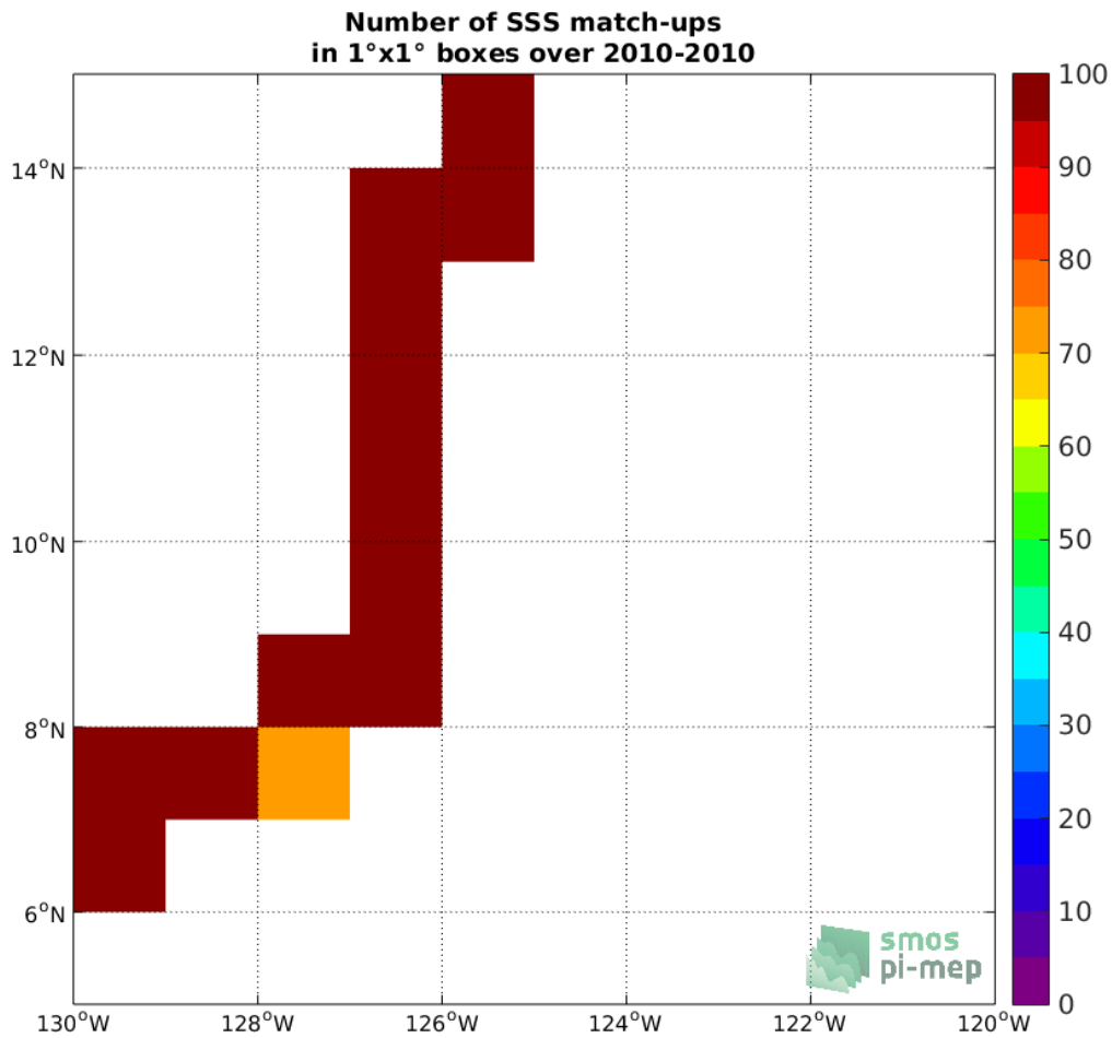
Figure 4: Number of SSS match-ups between TSG (GOSUD-Sailing-ship) SSS and the SMOS SSS L3 v5 - 18 Days (CATDS-CECOS-LOCEAN) SSS product for the SPURS 2 Pi-MEP region over 1°×1° boxes and for the full satellite product period.
