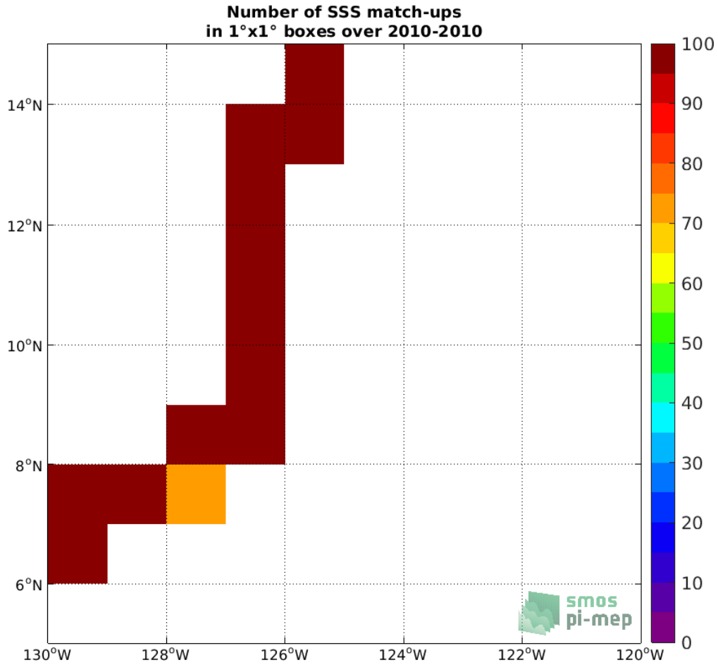
Figure 4: Number of SSS match-ups between TSG (GOSUD-Sailing-ship) SSS and the SMOS SSS L3 v5 - 18 Days (CATDS-CECOS-LOCEAN) SSS product for the SPURS 2 Pi-MEP region over 1°x1° boxes and for the full satellite product period.
