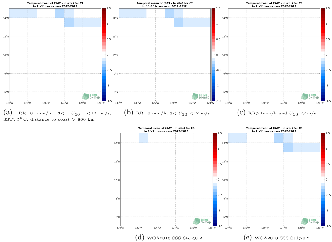
Figure 12: Temporal mean gridded over spatial boxes of size 1^\circ \times 1^\circ of \Delta SSS (SMOS SSS L3 v5 - 18 Days (CATDS-CECOS-LOCEAN) - TSG (GOSUD-Research-vessel)) for 5 different sub-datasets corresponding to:RR=0 mm/h, 3 < U_{10} < 12 m/s, SST>5°C, distance to coast > 800 km (a), RR=0 mm/h, 3 < U_{10} < 12 m/s (b), RR>1mm/h and U_{10} < 4 m/s (c), WOA2013 SSS Std<0.2 (d), WOA2013 SSS Std>0.2 (e).
