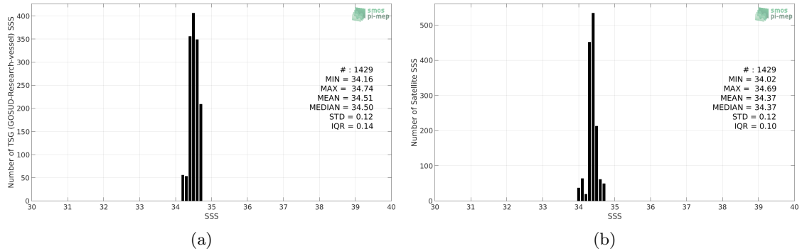
Figure 2: Histograms of SSS from TSG (GOSUD-Research-vessel) (a) and SMOS SSS L3 v5 - 18 Days (CATDS-CECOS-LOCEAN) (b) considering all match-up pairs per bins of 0.1 over the SPURS 2 Pi-MEP region and for the full satellite product period.
