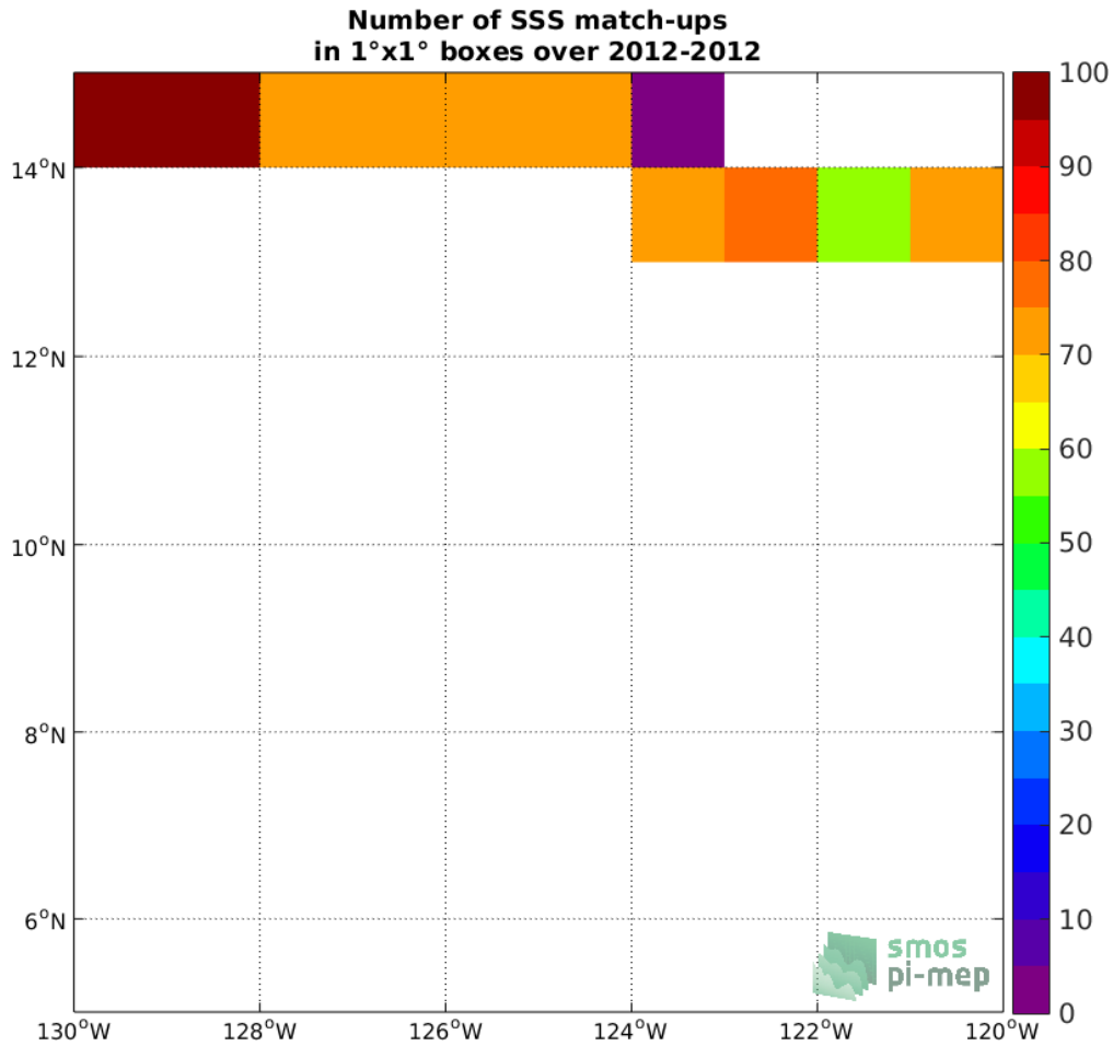
Figure 4: Number of SSS match-ups between TSG (GOSUD-Research-vessel) SSS and the SMOS SSS L3 v5 - 18 Days (CATDS-CECOS-LOCEAN) SSS product for the SPURS 2 Pi-MEP region over 1^\circ \times 1^\circ boxes and for the full satellite product period.
