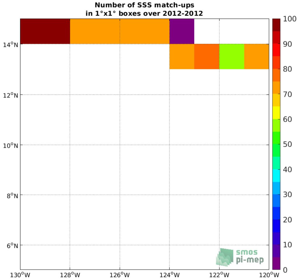
Figure 4: Number of SSS match-ups between TSG (GOSUD-Research-vessel) SSS and the SMOS SSS L3 v5 - 18 Days (CATDS-CECOS-LOCEAN) SSS product for the SPURS 2 Pi-MEP region over 1°x1° boxes and for the full satellite product period.
