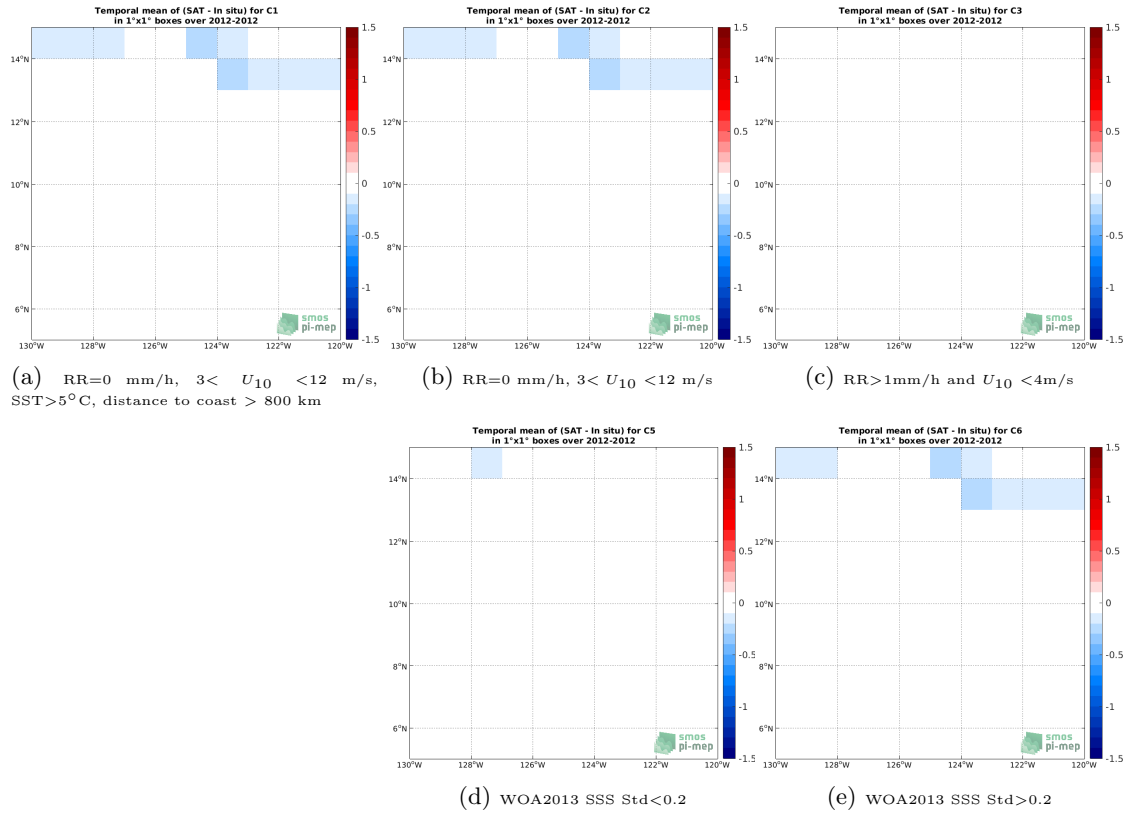
Figure 12: Temporal mean gridded over spatial boxes of size 1^\circ \times 1^\circ of \Delta SSS (SMOS SSS L3 v5 - 18 Days (CATDS-CECOS-LOCEAN) - TSG (GOSUD-Research-vessel)) for 5 different subdatasets corresponding to:RR=0 mm/h, 3 < U_{10} < 12 m/s, SST>5°C, distance to coast > 800 km (a), RR=0 mm/h, 3 < U_{10} < 12 m/s (b), RR>1mm/h and U_{10} < 4 m/s (c), WOA2013 SSS Std<0.2 (d), WOA2013 SSS Std>0.2 (e).
