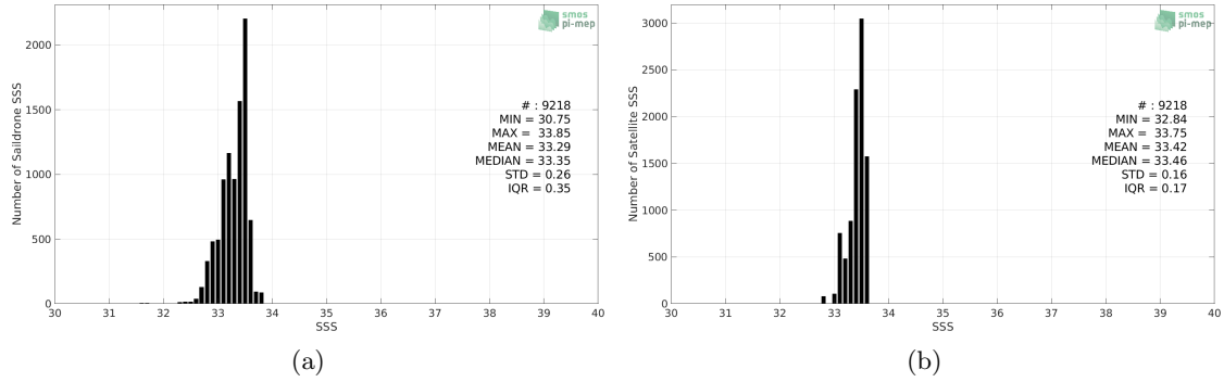
Figure 2: Histograms of SSS from Saifdrone (a) and SMOS SSS L3 v5 - 18 Days (CATDS-CECOS-LOCEAN) (b) considering all match-up pairs per bins of 0.1 over the SPURS 2 Pi-MEP region and for the full satellite product period.
