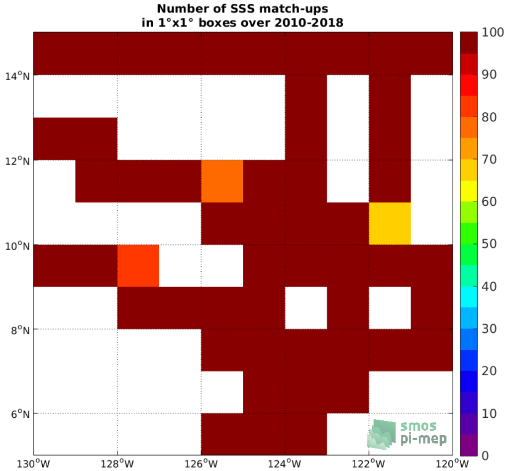
Figure 4: Number of SSS match-ups between TSG (SAMOS) SSS and the SMOS SSS L3 v4 - 9 Days (CATDS-CECOS-LOCEAN) SSS product for the SPURS 2 Pi-MEP region over 1°x1° boxes and for the full satellite product period.
