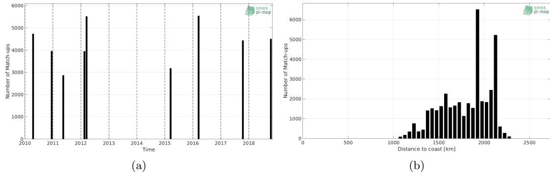
Figure 1: Number of match-ups between TSG (SAMOS) and SMOS SSS L3 v4 - 9 Days (CATDS-CECOS-LOCEAN) SSS as a function of time (a) and as function of the distance to coast (b) over the SPURS 2 Pi-MEP region and for the full satellite product period.
