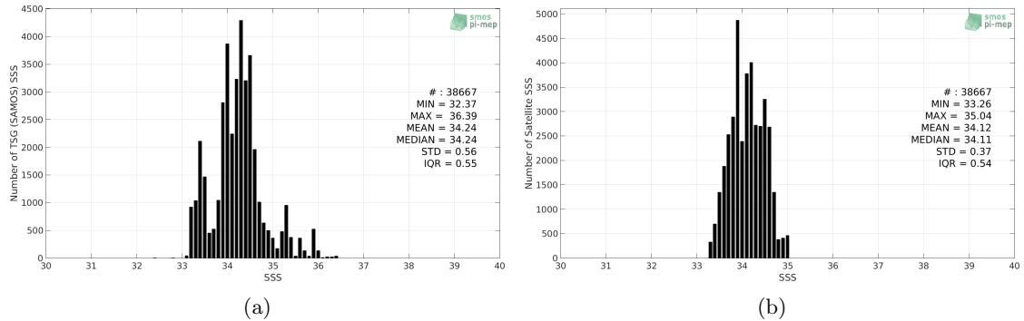
Figure 2: Histograms of SSS from TSG (SAMOS) (a) and SMOS SSS L3 v4 - 9 Days (CATDS-CECOS-LOCEAN) (b) considering all match-up pairs per bins of 0.1 over the SPURS 2 Pi-MEP region and for the full satellite product period.
