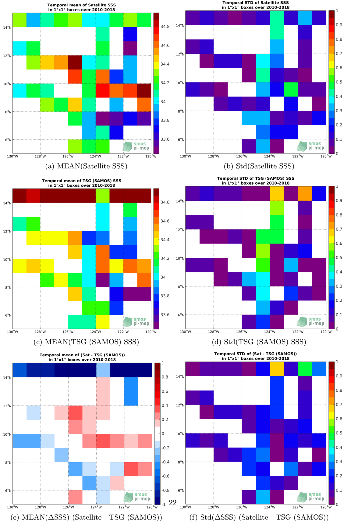
Figure 6: Temporal mean (left) and Std (right) of SSS from SMOS SSS L3 v4 - 9 Days (CATDS-CECOS-LOCEAN) (top), TSG (SAMOS) (middle), and of \Delta SSS (Satellite - TSG (SAMOS)). Only match-up pairs are used to generate these maps.
