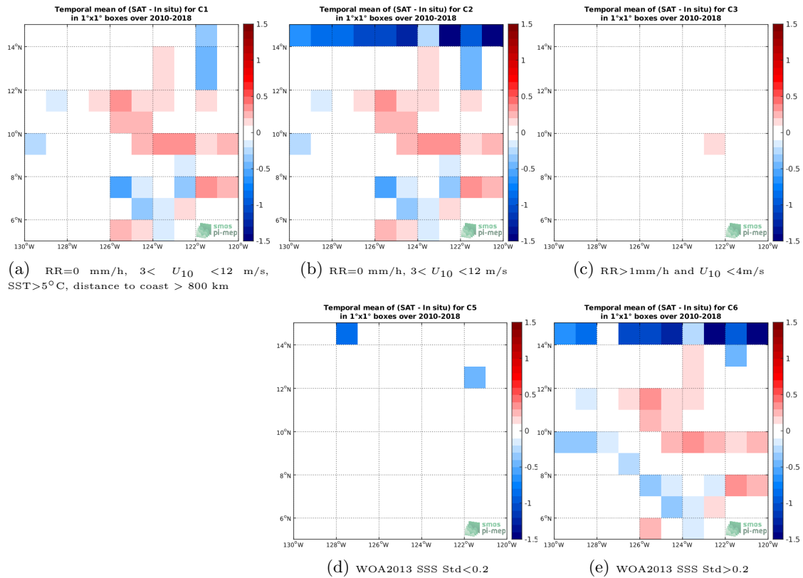
Figure 12: Temporal mean gridded over spatial boxes of size 1^\circ \times 1^\circ of \Delta SSS (SMOS-L3-CATDS-CECOS-LOCEAN-V4-9DAYS-25KM - TSG-SAMOS) for 5 different subdatasets corresponding to:RR=0 mm/h, 3 < U_{10} < 12 m/s, SST >5^\circ C, distance to coast > 800 km (a), RR=0 mm/h, 3 < U_{10} < 12 m/s (b), RR >1 mm/h and U_{10} < 4 m/s (c), WOA2013 SSS Std <0.2 (d), WOA2013 SSS Std >0.2 (e).
