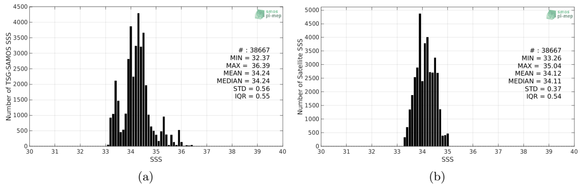
Figure 2: Histograms of SSS from TSG-SAMOS (a) and SMOS-L3-CATDS-CECOS-LOCEAN-V4-9DAYS-25KM (b) considering all match-up pairs per bins of 0.1 over the SPURS 2 Pi-MEP region and for the full satellite product period.
