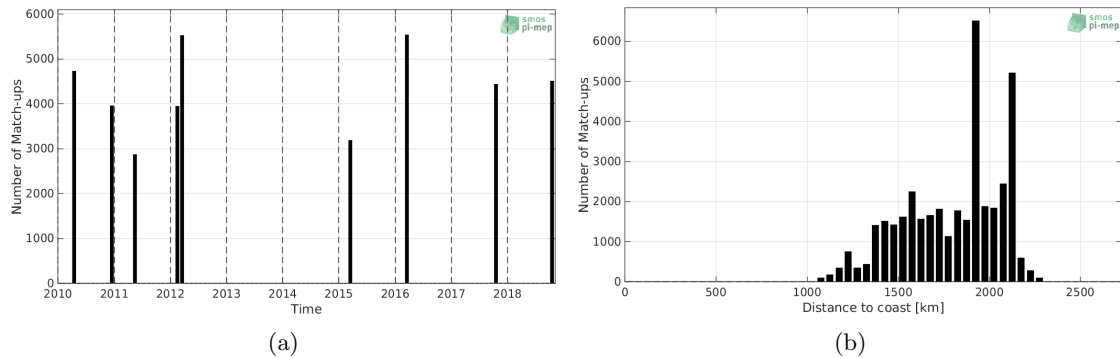
Figure 1: Number of match-ups between TSG-SAMOS and SMOS-L3-CATDS-CECOS-LOCEAN-V4-9DAYS-25KM SSS as a function of time (a) and as function of the distance to coast (b) over the SPURS 2 Pi-MEP region and for the full satellite product period.
