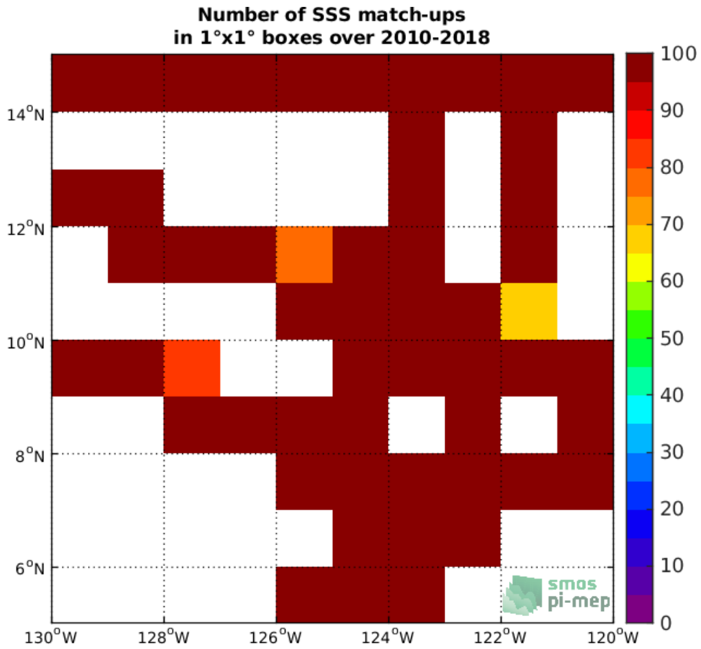
Figure 4: Number of SSS match-ups between TSG-SAMOS SSS and the SMOS-L3-CATDS-CECOS-LOCEAN-V4-9DAYS-25KM SSS product for the SPURS 2 Pi-MEP region over 1°x1° boxes and for the full satellite product period.
