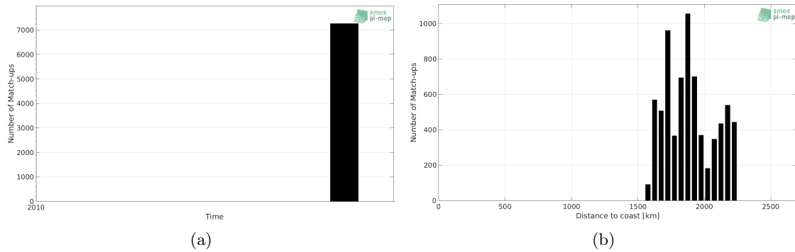
Figure 1: Number of match-ups between TSG-GOSUD-Sailing-ship and SMOS-L3-CATDS-CECOS-LOCEAN-V4-9DAYS-25KM SSS as a function of time (a) and as function of the distance to coast (b) over the SPURS 2 Pi-MEP region and for the full satellite product period.
