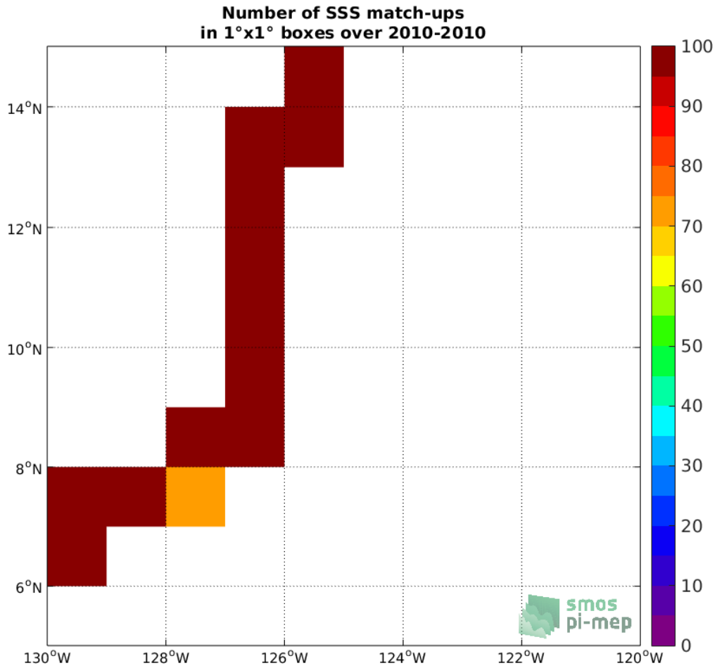
Figure 4: Number of SSS match-ups between TSG-GOSUD-Sailing-ship SSS and the SMOS-L3-CATDS-CECOS-LOCEAN-V4-9DAYS-25KM SSS product for the SPURS 2 Pi-MEP region over 1°x1° boxes and for the full satellite product period.
