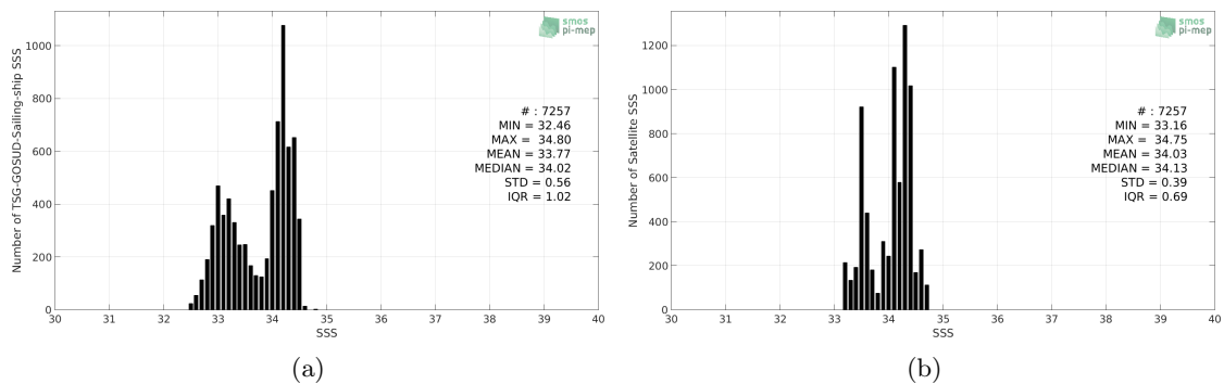
Figure 2: Histograms of SSS from TSG-GOSUD-Sailing-ship (a) and SMOS-L3-CATDS-CECOS-LOCEAN-V4-9DAYS-25KM (b) considering all match-up pairs per bins of 0.1 over the SPURS 2 Pi-MEP region and for the full satellite product period.
