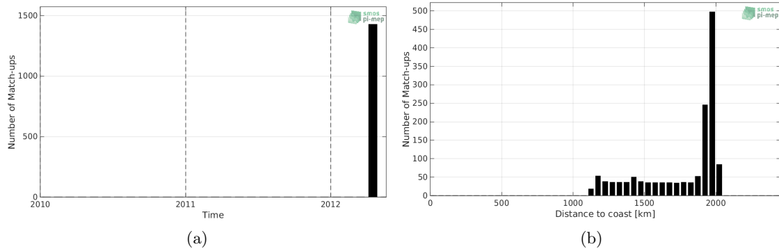
Figure 1: Number of match-ups between TSG-GOSUD-Research-vessel and SMOS-L3-CATDS-CECOS-LOCEAN-V4-9DAYS-25KM SSS as a function of time (a) and as function of the distance to coast (b) over the SPURS 2 Pi-MEP region and for the full satellite product period.
