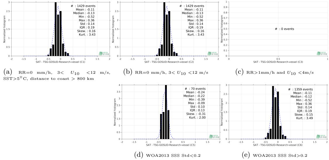
Figure 13: Normalized histogram of \Delta SSS (SMOS-L3-CATDS-CECOS-LOCEAN-V4-9DAYS-25KM - TSG-GOSUD-Research-vessel) for 5 different subdatasets corresponding to: RR=0 mm/h, 3 < U_{10} < 12 m/s, SST > 5°C, distance to coast > 800 km (a), RR=0 mm/h, 3 < U_{10} < 12 m/s (b), RR > 1mm/h and U_{10} < 4 m/s (c), WOA2013 SSS Std < 0.2 (d), WOA2013 SSS Std > 0.2 (e).
