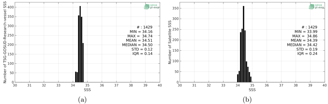
Figure 2: Histograms of SSS from TSG-GOSUD-Research-vessel (a) and SMOS-L3-CATDS-CECOS-LOCEAN-V4-9DAYS-25KM (b) considering all match-up pairs per bins of 0.1 over the SPURS 2 Pi-MEP region and for the full satellite product period.
