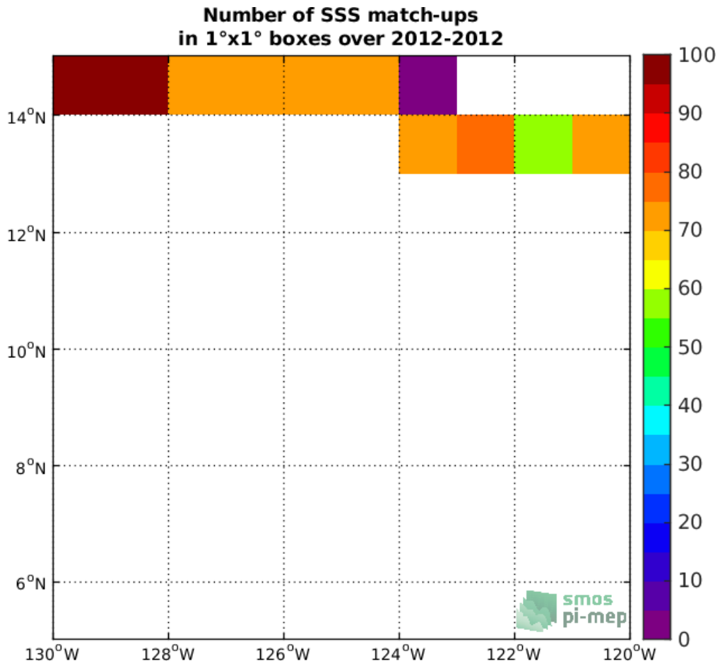
Figure 4: Number of SSS match-ups between TSG-GOSUD-Research-vessel SSS and the SMOS-L3-CATDS-CECOS-LOCEAN-V4-9DAYS-25KM SSS product for the SPURS 2 Pi-MEP region over 1°x1° boxes and for the full satellite product period.
