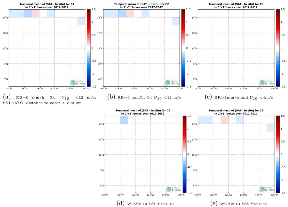
Figure 12: Temporal mean gridded over spatial boxes of size 1^\circ \times 1^\circ of \Delta SSS (SMOS-L3-CATDS-CECOS-LOCEAN-V4-9DAYS-25KM - TSG-GOSUD-Research-vessel) for 5 different subdatasets corresponding to:RR=0 mm/h, 3 < U_{10} < 12 m/s, SST >5^\circ C, distance to coast > 800 km (a), RR=0 mm/h, 3 < U_{10} < 12 m/s (b), RR >1 mm/h and U_{10} < 4 m/s (c), WOA2013 SSS Std <0.2 (d), WOA2013 SSS Std >0.2 (e).
