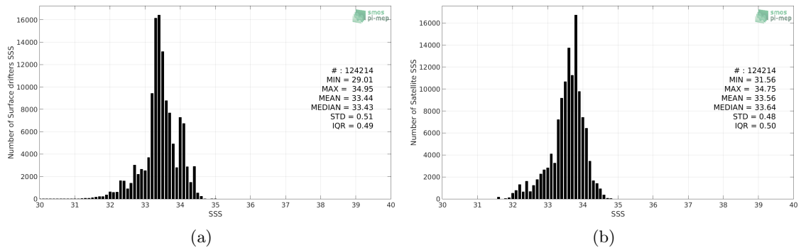
Figure 2: Histograms of SSS from Surface drifters (a) and SMOS-L3-CATDS-CECOS-LOCEAN-V4-9DAYS-25KM (b) considering all match-up pairs per bins of 0.1 over the SPURS 2 Pi-MEP region and for the full satellite product period.
