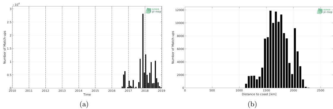
Figure 1: Number of match-ups between Surface drifters and SMOS-L3-CATDS-CECOS-LOCEAN-V4-9DAYS-25KM SSS as a function of time (a) and as function of the distance to coast (b) over the SPURS 2 Pi-MEP region and for the full satellite product period.
