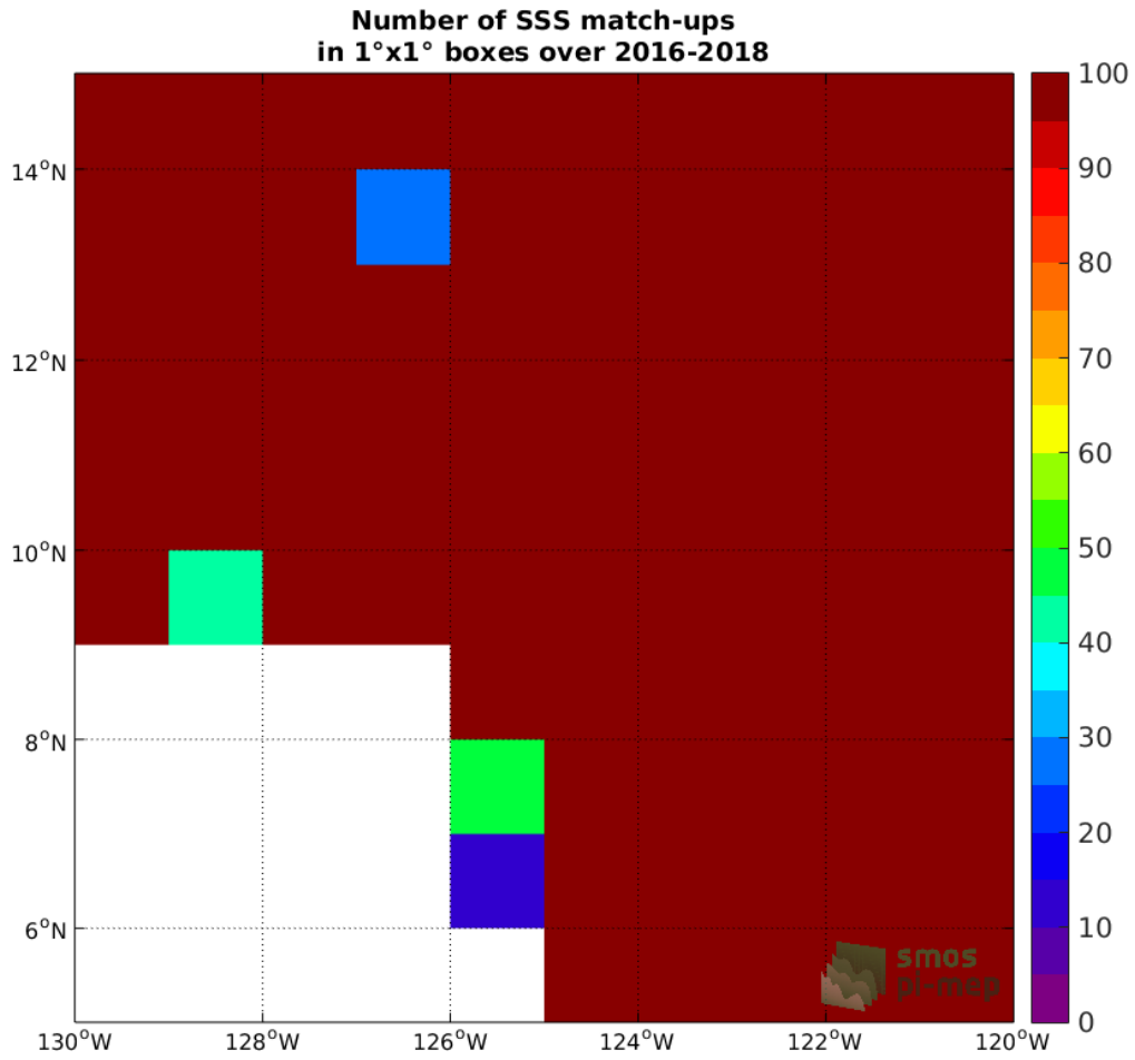
Figure 3: Number of SSS match-ups between Surface drifters SSS and the SMOS-L3-CATDS-CECOS-LOCEAN-V4-9DAYS-25KM SSS product for the SPURS 2 Pi-MEP region over 1°x1° boxes and for the full satellite product period.
