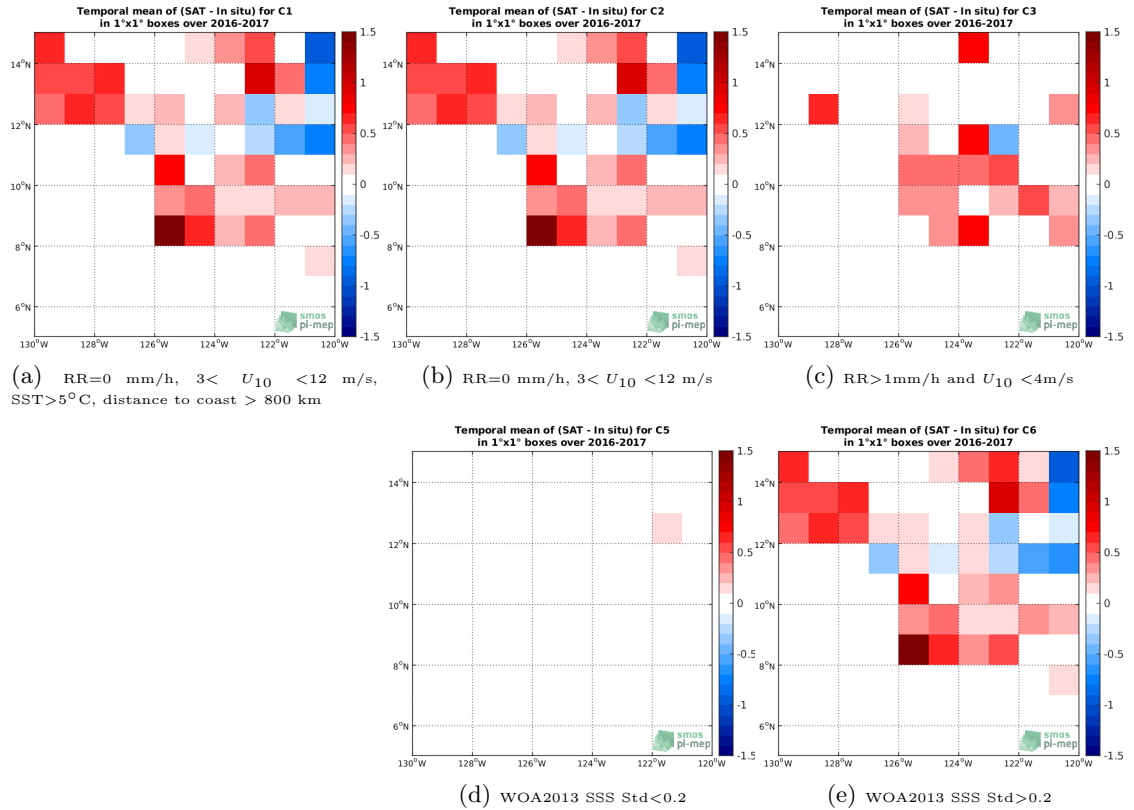
Figure 11: Temporal mean gridded over spatial boxes of size 1^\circ \times 1^\circ of \Delta SSS (SMOS-L3-CATDS-CECOS-LOCEAN-V4-9DAYS-25KM - Surface drifters) for 5 different subdatasets corresponding to: RR=0 mm/h, 3 < U_{10} < 12 m/s, SST >5^\circ\text{C} , distance to coast > 800 km (a), RR=0 mm/h, 3 < U_{10} < 12 m/s (b), RR >1 mm/h and U_{10} < 4 m/s (c), WOA2013 SSS Std <0.2 (d), WOA2013 SSS Std >0.2 (e).
